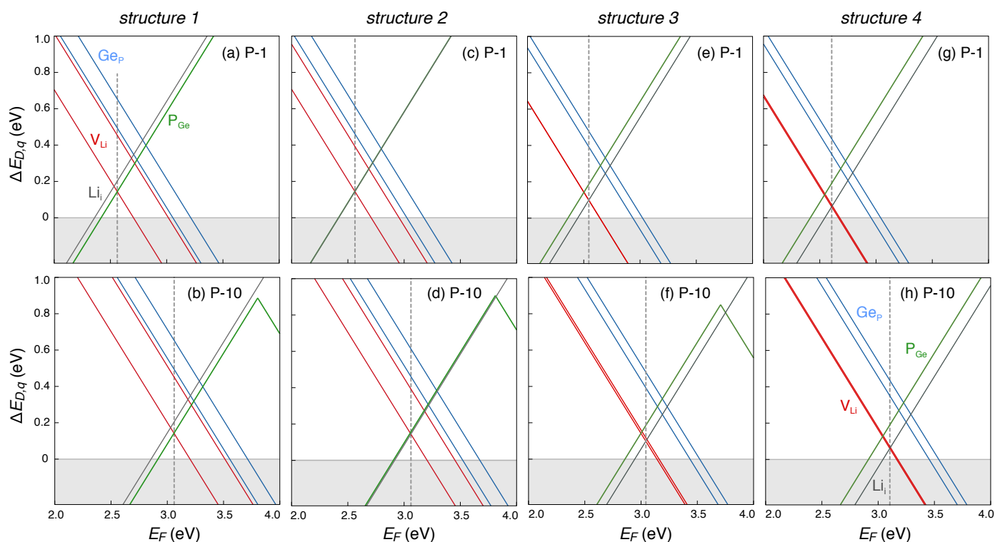
Fig. 5 Formation energies of native point defects ( V_{Li} , Li_i , P_{Ge} , and Ge_P ) as functions of Fermi energy ( E_F ) in LGPS structures 1-4 (Figure 3) at elemental chemical potentials corresponding to P-1 (a, c, e, g), and P-10 (b, d, f, h). E_F is referenced to the valence band maximum. Multiple lines of the same color represent the same defect type at different Wyckoff sites.
