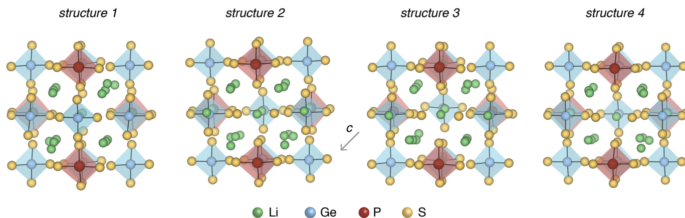
Fig. 3 Four representative LGPS structures selected for defect calculations. All four structures exhibit the so-called Z configuration of the \text{GeS}_4 and \text{P1S}_4 tetrahedra. The structures differ in the Li site occupations and have slightly different volumes per atom (19.74, 19.84, 19.94, 20.02 \text{\AA}^3/\text{atom} ).
