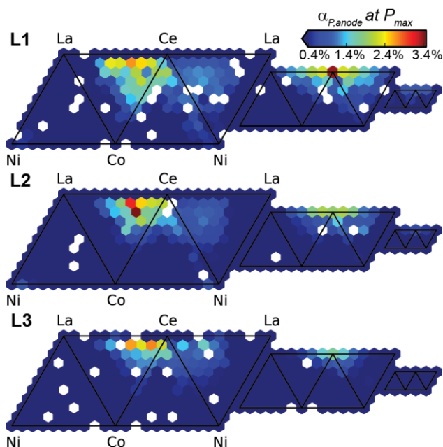
Fig. 10. Power conversion efficiency ( \alpha_{P,anode} ) for each photoanode at its maximum power point. The conversion efficiency is calculated as the ratio of the maximum electrochemical power generation ( P_{max} ) to the consumed optical power (reflected or absorbed irradiation, P_{consumed} ). For bare BiVO_4 , this efficiency is below the colour scale at 0.16%.
