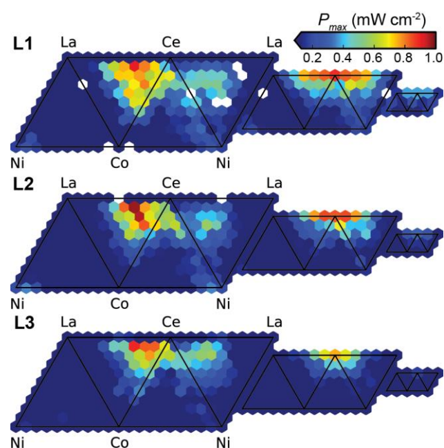
Fig. 5. Composition maps of P_{max} for all three catalyst loadings, plotted with a common colour scale using the flattened pseudo-ternary triangle scheme of Figure 4a.
