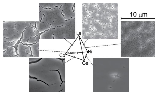
Fig. 2. The pseudo-quaternary catalyst composition space tetrahedron is shown with points marking the 1:1 mixtures along each of the 6 pseudo-binary lines. A scanning electron microscopy image ( 10 \times 10 \mu\text{m} square) is shown for each of these compositions with the L3 loading, revealing the presence of 1 \mu\text{m} -scale cracks.
