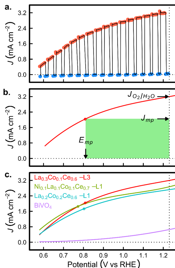
Fig. 3. (a) Anodic sweep of the CV acquired on L3 sample \text{La}_{0.3}\text{Co}_{0.1}\text{Ce}_{0.6}\text{O}_x with illuminated (1.34 s) and dark (0.67 s) intervals highlighted in red and blue, respectively. (b) Disregarding the current transients upon illumination toggling, the photocurrent density is fit to a 3 rd order polynomial (red line), providing the J_{\text{photo}}(V) signal from which performance metrics are calculated. The short circuit current density ( J_{\text{O}_2/\text{H}_2\text{O}} ) is labelled as well as the maximum power point (red circle), which corresponds to an electrochemical power generation of P_{\text{max}} (shaded green area). (c) Representative photocurrent density signals from 3 of the best photoanodes are shown along with the photocurrent density signal from bare BiVO _4 . The maximum power point is circled for each photoanode.
