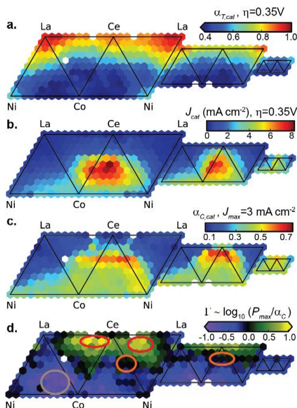
Fig. 8. Composition maps of (a) optical transmission efficiency ( \alpha_{T,cat} ), (b) catalytic current density ( J_{cat} ), and the ensuing (c) combined figure of merit ( \alpha_{C,cat} ) for the L3 catalyst samples from the FTO/glass-supported library. The parameter \Gamma compares photoanode performance ( P_{max} ) to that predicted by \alpha_{C,cat} , and the corresponding composition map is shown in (d).
