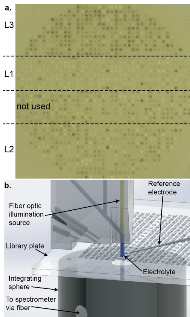
Fig. 1. (a) Photograph of the 10 cm \times 10 cm FTO/glass plate with the (Ni-La-Co-Ce) O_x catalyst library on BiVO _4 . The regions of the library containing catalyst loadings L1, L2, and L3 are marked, with each of these regions containing the same 286 catalyst compositions. (b) Schematic of the scanning droplet cell (SDC) instrument in which the catalyst library is suspended between a 3-electrode electrochemical cell and an integrating sphere that collects transmitted light. The SDC contacts a single photoanode sample and is rastered across the library. Some SDC components have been removed for clarity.
