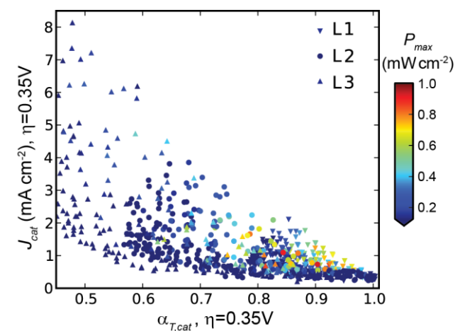
Fig. 7. Each of the 858 library samples is plotted according to the optical transmission efficiency ( \alpha_{T,cat} ) and catalytic activity ( J_{cat} ) measured on the FTO/glass-supported library. Each sample is coloured by the P_{max} measured on the BiVO_4 photoanode library. Each sample with high P_{max} (green to red colours) is surrounded by samples with much lower P_{max} , demonstrating the lack of a systematic relationship among \alpha_{T,cat} , J_{cat} , and P_{max} .
