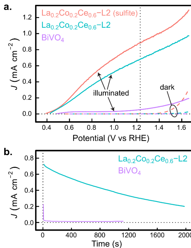
Fig. 6. (a) The anodic sweep from 6 CV measurements using a traditional cell and AM 1.5 light source. The illuminated (solid line) and dark (dashed line) current density are shown for bare BiVO_4 and for the scaled-up La_{0.2}Co_{0.2}Ce_{0.6}O_x -L2 sample; the latter sample was measured without and then with the addition of 0.1 M sulfite ( Na_2SO_3 ) to the 0.1 M NaOH electrolyte. (b) The stability of the short circuit photocurrent density (1.23 V vs RHE) of bare BiVO_4 and scaled-up La_{0.2}Co_{0.2}Ce_{0.6}O_x -L2 are measured under AM 1.5 illumination.
