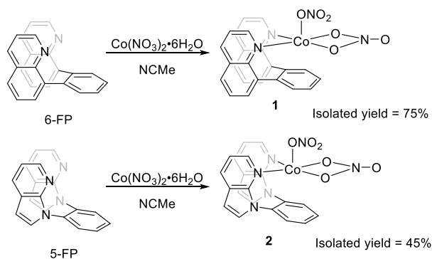
Scheme 4. Synthetic routes to (6-FP) \text{Co}(\text{NO}_3)_2 ( 1 , top) (6-FP = 8,8'-(1,2-phenylene)diquinoline) and (5-FP) \text{Co}(\text{NO}_3)_2 ( 2 , bottom) (5-FP = 1,2-bis(N-7-azaindoly)benzene).
