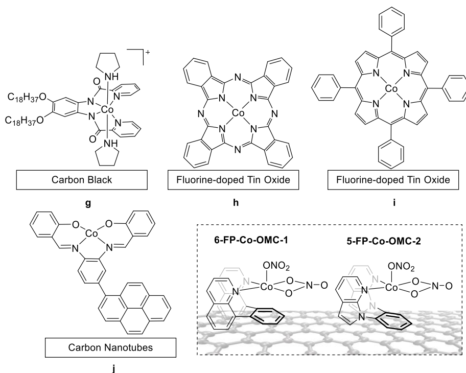
Scheme 2. Depiction of selected cobalt heterogenized catalysts for electrochemical water oxidation. g : ref 50; h : ref 53; i : ref 28; j : ref 55; 6-FP-Co-OMC-1 and 5-FP-Co-OMC-2 : this work.
