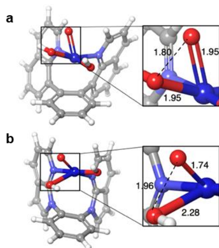
Figure 9. DFT-Optimized transition states for O–O bond generation via intramolecular reductive elimination. (a) The 6-FP-Co system. (b) The 5-FP-Co system. These calculations were performed with implicit PBF solvation plus two explicit water molecules, which are omitted from the graphic for clarity. Lengths are in Å.
