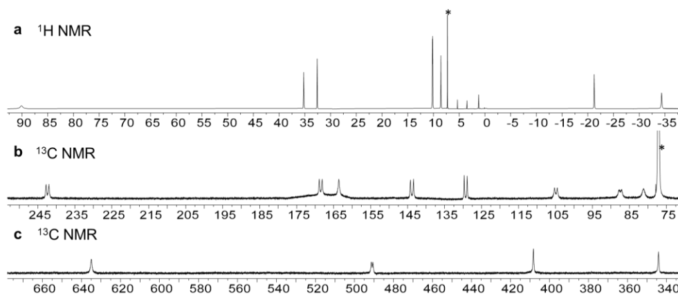
Figure 2. NMR characterization of (6\text{-FP})\text{Co}(\text{NO}_3)_2 . (a) ^1\text{H} NMR spectrum of (6\text{-FP})\text{Co}(\text{NO}_3)_2 ( 1 ) in \text{CDCl}_3 . (b) ^{13}\text{C} NMR spectrum from 70 to 250 ppm of (6\text{-FP})\text{Co}(\text{NO}_3)_2 ( 1 ) in \text{CDCl}_3 . (c) ^{13}\text{C} NMR spectrum from 330 to 680 ppm of (6\text{-FP})\text{Co}(\text{NO}_3)_2 ( 1 ) in \text{CDCl}_3 . * Indicates \text{CDCl}_3 in spectra.
