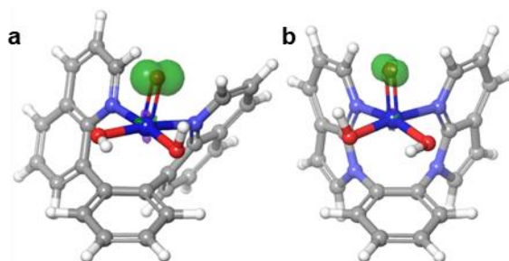
Figure 8. DFT-optimized structures of Co molecular complexes. (a) (6\text{-FP})\text{Co}(\text{OH})_2(\text{O}) . (b) (5\text{-FP})\text{Co}(\text{OH})_2(\text{O}) . Spin density surfaces are also provided. The Spin density surface areas for (6\text{-FP})\text{Co}(\text{OH})_2(\text{O}) and (6\text{-FP})\text{Co}(\text{OH})_2(\text{O}) are 8.58 and 5.68 Å 2 , respectively. Note that the oxygen spin is in a p orbital overlapping the OH at a 90° O-Co-OH dihedral angle.
