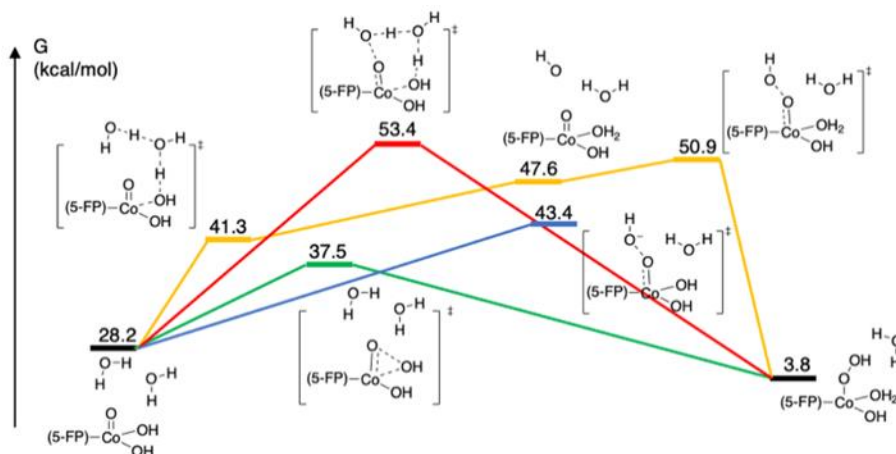
Scheme 7. DFT Free energies at 298 K for the possible O–O bond formation mechanisms: path 1 (green), 2 (orange), 3 (red), and 4 (blue). Free energies are relative to the (5-FP)Co(OH) 2 (H 2 O) starting state. Relative energies are not to scale.
