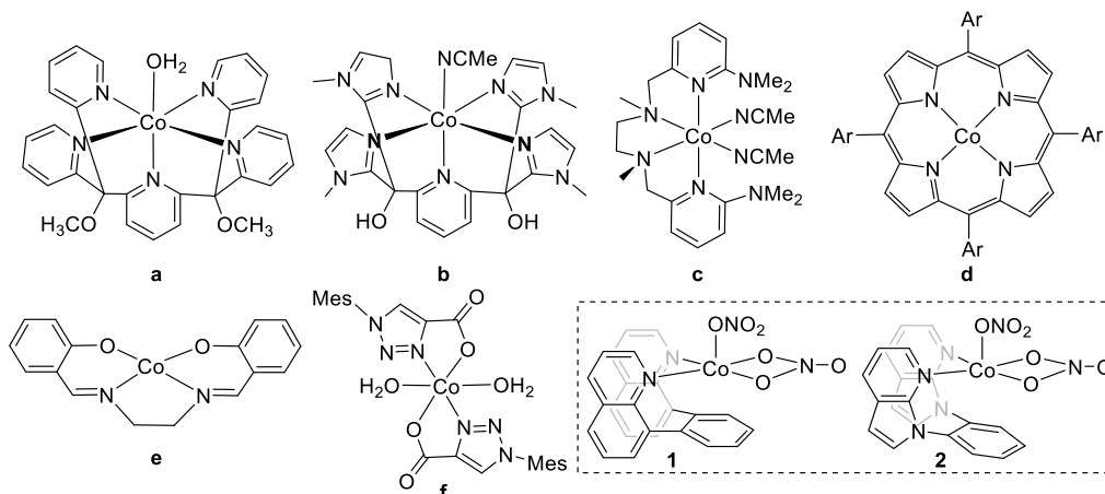
Scheme 1. Molecular structures of selected cobalt(II) molecular precatalysts for electrochemical water oxidation . a: ref 33 and 34; b: ref 22; c: ref 23; d: ref 24 and 36; e: ref 29; f: ref 37; 1 and 2: this work.
