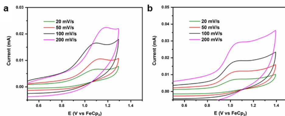
Figure 4. Electrochemical characterization of Co complexes in homogeneous system. (a) Cyclic voltammogram of (6-FP)Co(NO 3 ) 2 ( 1 ) in MeCN at variable scan rates. (b) Cyclic voltammogram of (5-FP)Co(NO 3 ) 2 ( 2 ) in MeCN at variable scan rates.
