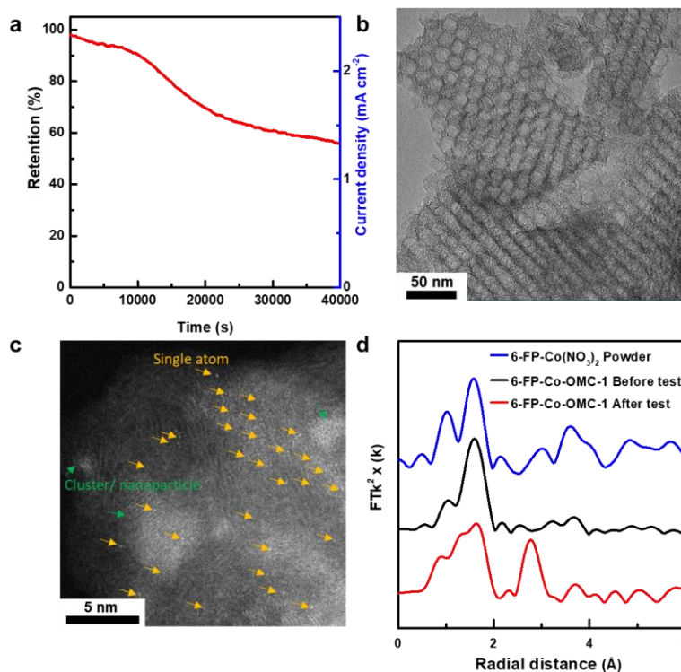
Figure 7. OER stability investigation on (6-FP)Co(NO 3 ) 2 loaded OMC. (a) Stability test of 6-FP-Co-OMC-1 with chronoamperometry (CA) test for 11 hours. (b) TEM image of 6-FP-Co-OMC-1 after CA test at 300 mV overpotential. (c) HAADF-STEM image of 6-FP-Co-OMC-1 after CA test at 300 mV overpotential. (d) EXAFS analysis for (6-FP)Co(NO 3 ) 2 ( 1 ) and 6-FP-Co-OMC-1 before and after OER test.
