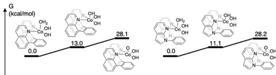
Scheme 5. DFT free energies at 298 K for the oxidation of (6\text{-FP})\text{Co}(\text{OH})_2(\text{H}_2\text{O}) (left) and (5\text{-FP})\text{Co}(\text{OH})_2(\text{H}_2\text{O}) (right). Free energies are calculated at 0.7 V vs. RHE.
