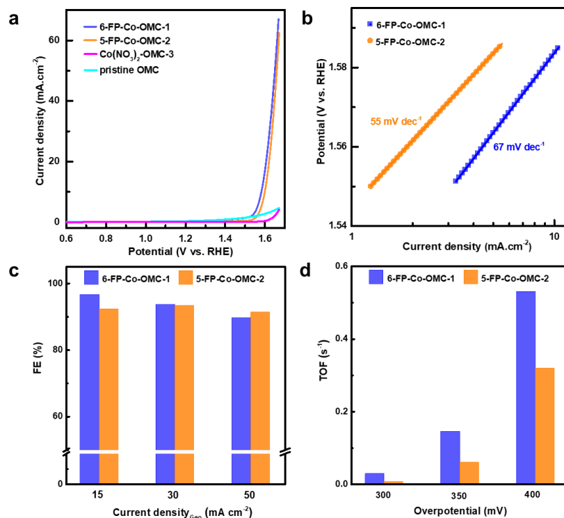
Figure 6. OER catalytic performance of Co complexes loaded OMC. (a) LSV plot of 6-FP-Co-OMC-1 (dark blue), 5-FP-Co-OMC-2 (orange), Co(NO 3 ) 2 -OMC-3 (pink) and pristine OMC (light blue). (b) Tafel plot of 6-FP-Co-OMC-1 (blue) and 5-FP-Co-OMC-2 (orange). (c) Faradic efficiency of 6-FP-Co-OMC-1 and 5-FP-Co-OMC-2 at different current densities. (d) TOFs of 6-FP-Co-OMC-1 and 5-FP-Co-OMC-2 at different OER overpotential.
