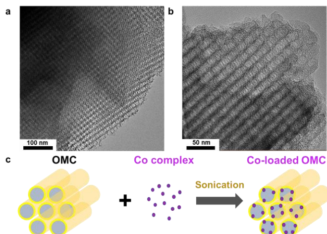
Figure 5. Morphology characterizations of OMC and Co complex loaded OMC. (a) TEM of the OMC after 900 °C treatment in forming gas (5% H 2 in N 2 ). (b) TEM image of 6-FP-Co-OMC-1 . (c) Schematic illustration of immobilization of Co complex on OMC.
