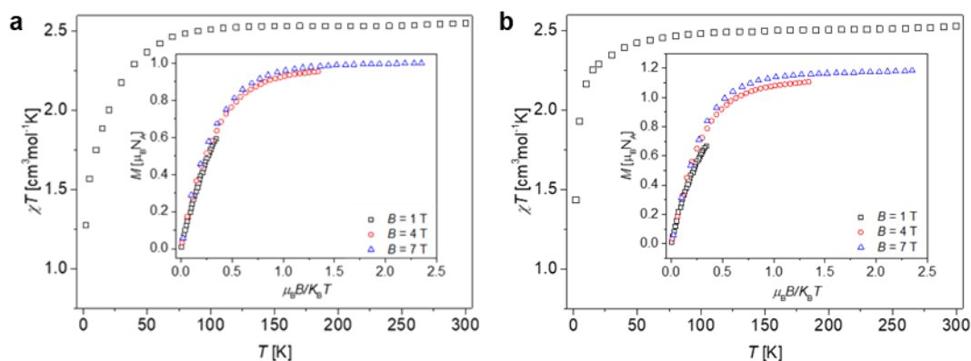
Figure 3. Magnetic susceptibility of (a) 1 ; and (b) 2 , as \chi T product vs temperature. (inset) Reduced magnetization at magnetic fields of 1 T ( \square ), 4 T ( \circ ) and 7 T ( \Delta ) for 1 and 2 , respectively.
