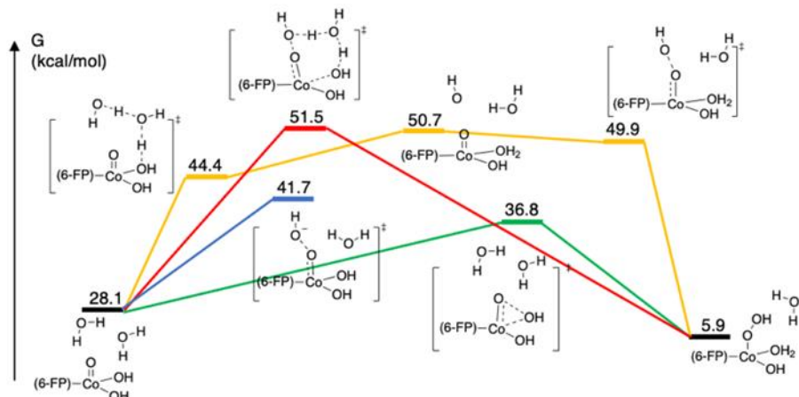
Scheme 6. DFT Free energies at 298 K for the possible O–O bond formation mechanisms: path 1 (green), 2 (orange), 3 (red), and 4 (blue). Free energies are relative to the (6-FP)Co(OH) 2 (H 2 O) starting state. Relative energies are not to scale.
