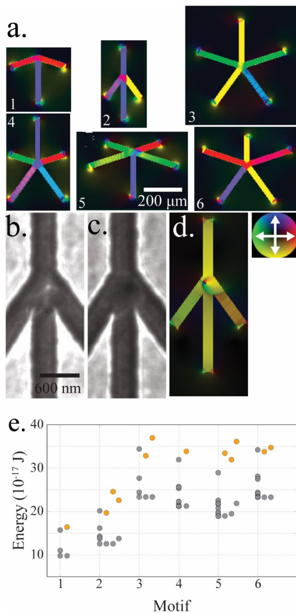
Figure 2—See online for color. a) Micromagnetic simulations for vertex motifs 1–6 in their lowest energy configuration. The color in each bar shows the direction of magnetization as indicated by the color wheel on the right. b) Fresnel contrast LTEM image of a counterclockwise magnetic vortex in a Motif-2 vertex, which appears as a white dot. c) Fresnel contrast LTEM image showing a clockwise magnetic vortex (black dot). d) Micromagnetic simulation of a clockwise vortex as seen in c). e) Plot showing the energy calculated from micromagnetic simulations for having a vortex in each of the vertex motifs. The orange dots indicate the energy of a motif configuration with a vortex in it and the gray dots underneath indicate the energy of the corresponding configuration with no vortex. For two orange dots corresponding to a gray dot with the same energy value, the difference represents the difference in energy between a clockwise and counterclockwise vortex. The gray dots to the left for each vertex motif show the energies of all the configurations without a vortex. Only the configurations in which vortices were observed experimentally were simulated.
