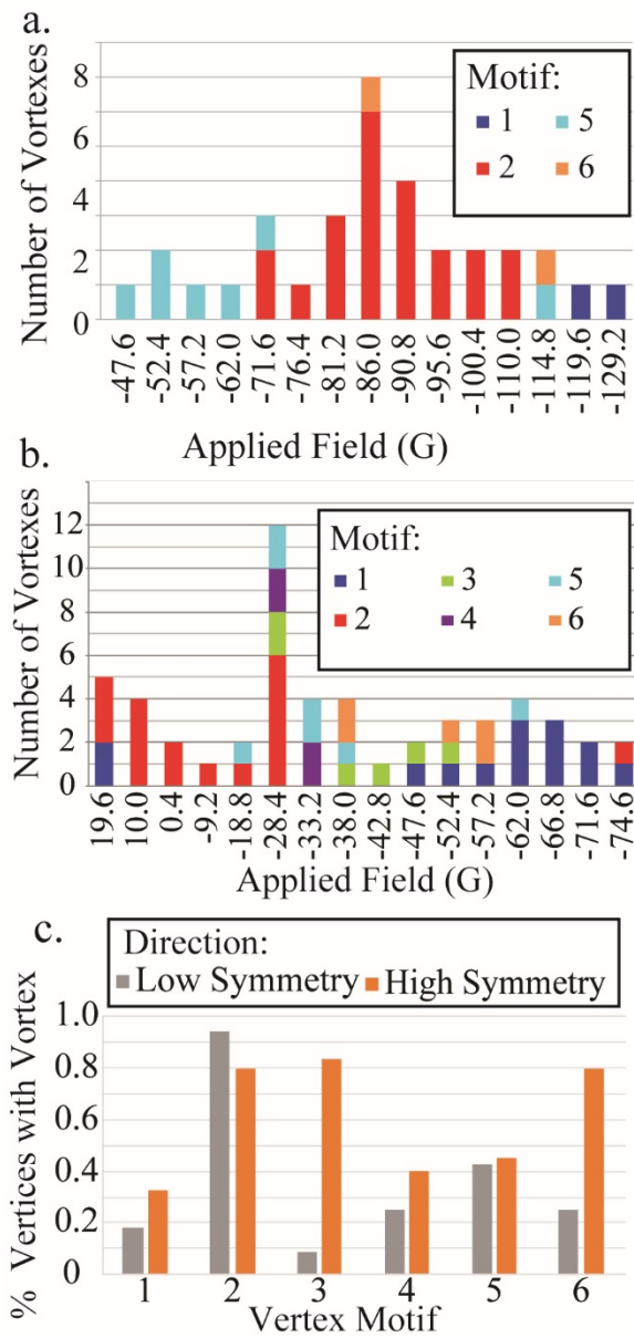
Figure 3—See online for color. a) A graph showing the number of vortexes that formed as a function of applied field, for the field applied along a low symmetry direction. Each bar is divided into one or more colors indicating the number of vortexes that formed in each motif type (see key below). b) A graph showing the same information as in a) but with the applied field along a high-symmetry direction. c) A graph showing the percentage of each vertex motif in which a vortex was observed, for the low-symmetry field direction (gray) and the high-symmetry field direction (orange).
