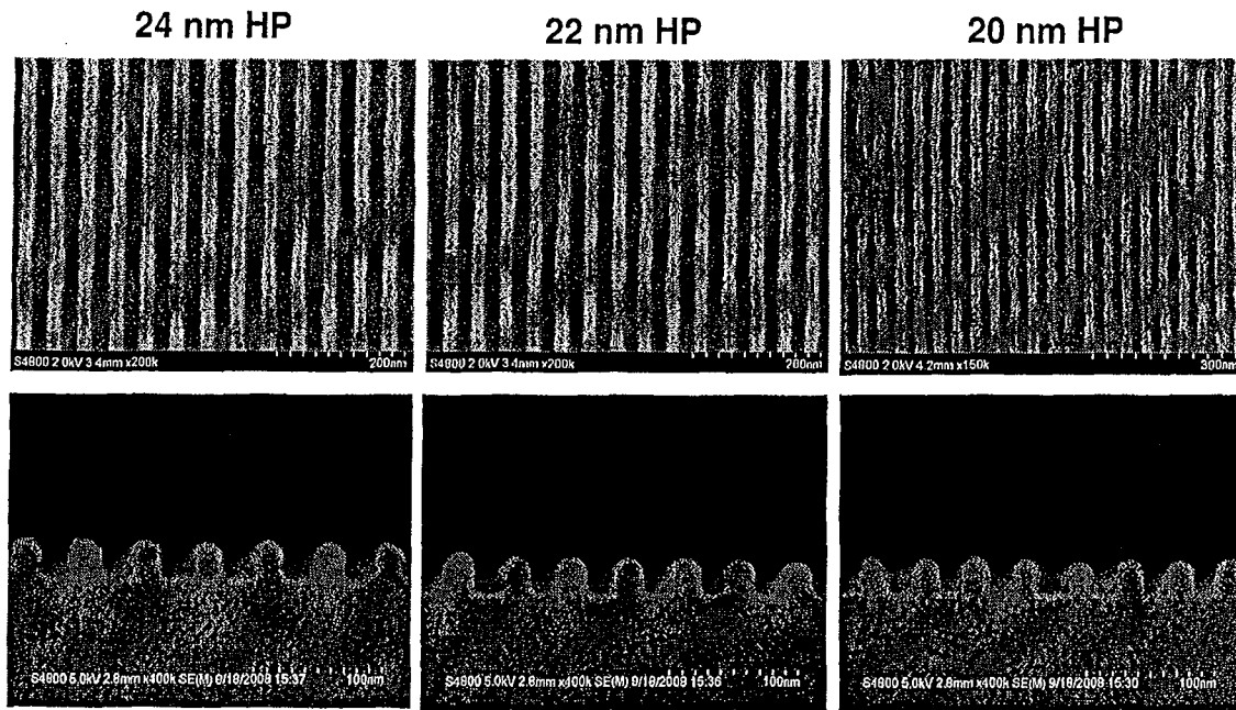
Fig. 2. Imaging results from a chemically amplified resist with a sensitivity of 15.2 mJ/cm 2 .
