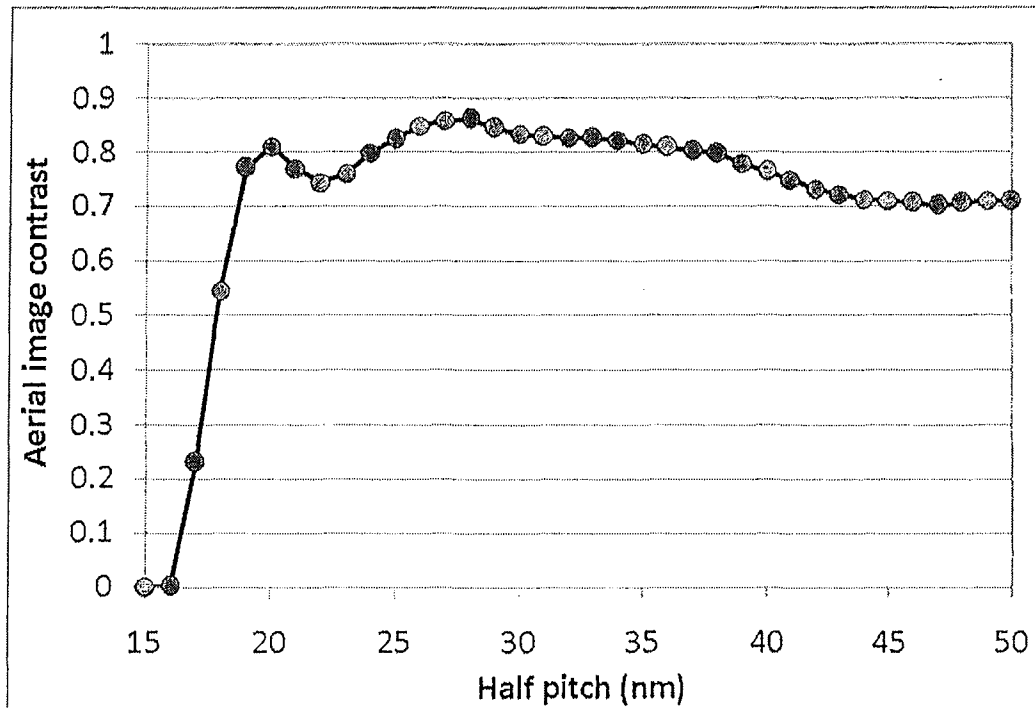
Fig. 1. Computed aerial-image contrast for the SEMATECH Berkeley MET using modified illumination (dipole, pole radius \sigma = 0.1 , pole offset \sigma = 0.57 , pole orientation = 45^\circ ).
