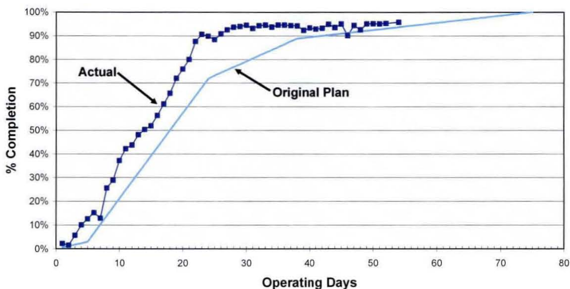
Fig. 1. Comparison of Predicted and Actual Waste Retrieval Rates from Tank C-103
