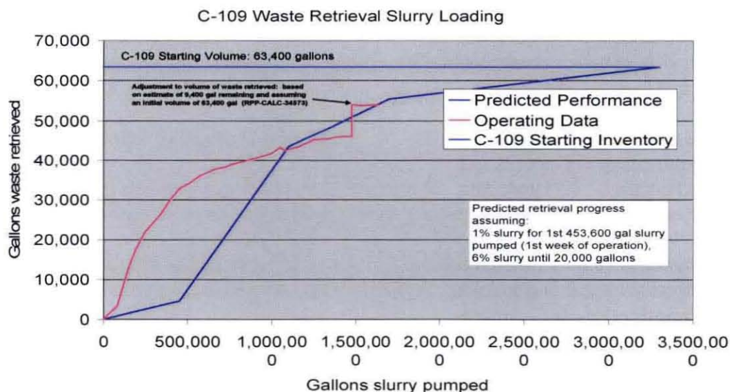
Fig. 3. C-109 Waste Retrieval Efficiency
