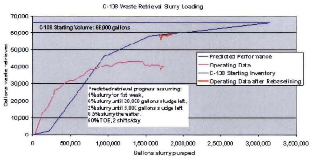
Fig. 2. C-108 Waste Retrieval Slurry Loading
