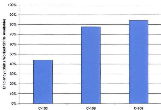
Fig. 4. Comparison of Modified Sluicing Efficiencies
