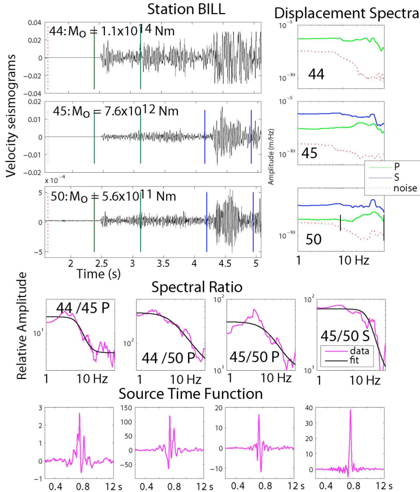
Figure 3. Example of the direct wave analysis for 3 earthquakes in one cluster of Au Sable Forks aftershocks. We show the vertical component, velocity seismograms, with the noise, P and S windows marked. The corresponding displacement spectra are shown using the same color coding. The spectral ratios and source time functions obtained by transforming the ratios back to the time domain are shown at the bottom. Earthquake 44 appears to have a complex source time function with at least 2 subevents.
