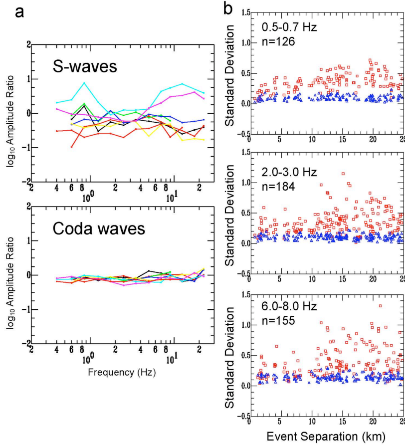
Figure 1. (a) An example of amplitude ratio pairs for a pair of events (M3.6 and 3.7) separated by 16 km epicentral distance. (Top) direct S-wave ratios for 8 color-coded stations show significant scatter over the entire frequency range, whereas (bottom) the coda wave amplitude ratios are very stable from station to station. (b) amplitude ratio standard deviation versus event separation for coda (blue triangles) and direct waves (red squares) for all ratios that had at least 5 stations recording. Three frequency bands are shown: top 0.5-0.7 Hz, middle 2.0-3.0 Hz, and bottom 6.0-8.0 Hz. Note that the coda scatter shows almost no dependence on distance, in contrast to the direct waves, and is roughly a factor of 3 smaller.
