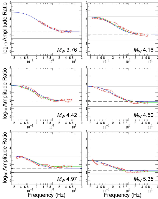
Figure 2. Spectral ratios for the Hector Mine mainshock relative to 6 aftershocks. In each figure, we show the low and high frequency asymptotes from equation 1 as solid black horizontal lines and dashed lines represent the case when p = 1.5 . The average for each band is shown by red triangles and red lines represent \pm 1\sigma . Blue lines represent the best fitting MDAC spectral ratios that fit all 6 ratios simultaneously, whereas the green lines represent the case when each ratio was fit individually. We find that the best fitting model corresponds to a reference event of M_w 5.0 with an apparent stress of 0.1 MPa and a scaling parameter ( \psi ), of 0.25, in good agreement with previous studies using independent methods.
