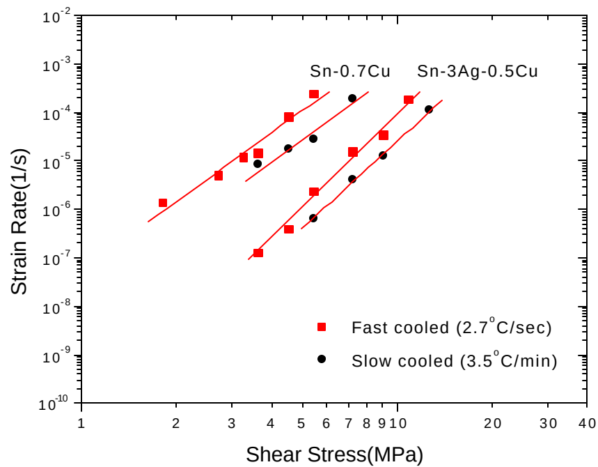
Figure 9. The influence of the cooling rate on creep at 130°C in Sn-0.7Cu and Sn-3Ag-0.5Cu solder joints.
