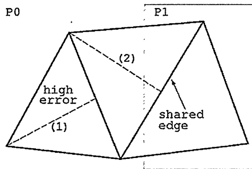
Figure 2. Edge Bisected by Owning Processor
