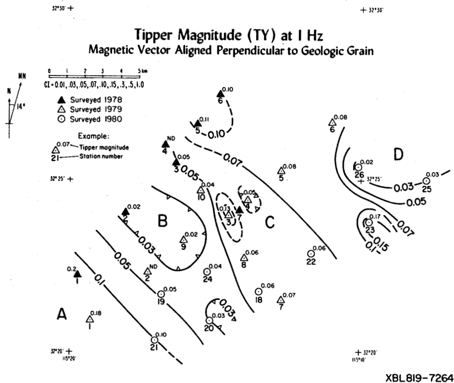
Figure 10. Map of the tipper amplitude, T_y , at 1 Hz over the area of the geothermal field. The magnetic vector is aligned perpendicular to geologic grain, or in a northeast-southwest direction. T_y is sensitive to the resistive rocks of the Cucupá Range (A), an elongate, deep sedimentary basin (B), the resistive dome of the reservoir apex (C) and the encroachment of colder, less saline water from the Colorado River (D).
