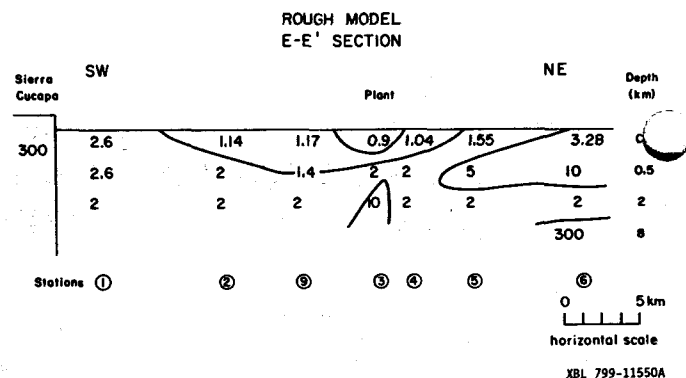
Figure 3. Approximate subsurface model inferred from magnetotelluric data along line E-E'. Values in ohm-meters.
