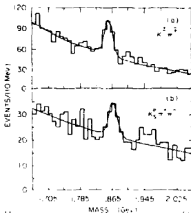
Fig. 21. K^+\pi^+ and K_S^0\pi^+\pi^- mass spectra from the CIF experiment for events with M_{K^+\pi^-} = M_{K^0\pi^-} (or M_{K^+\pi^-} = M_{K^0\pi^-} ) around 145 MeV.
