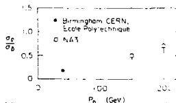
Fig. 30. Ratio of \sigma(pN \rightarrow J/\psi + X) / \sigma(pN \rightarrow J/\psi + X) as a function of incident energy.
