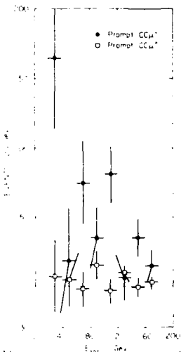
Fig. 15. Prompt CC \mu^+ and \mu^- spectra from CBHS experiment using the extrapolation method.
