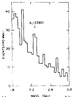
Fig. 10. K^0 \pi^+ and \Lambda \pi^+ mass spectrum from the vD exposure.
