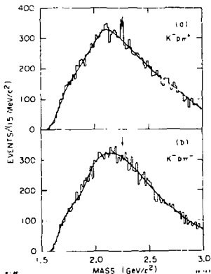
Fig. 5. a) K^- p \pi^+ and b) K^- p \pi^- mass spectrum from the LSM experiment ( K^- trigger).
