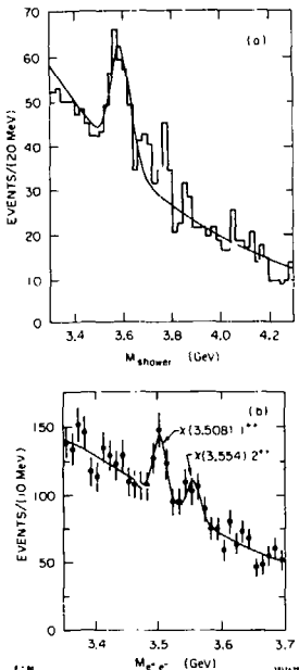
Fig. 32. Mass spectrum of the J/\psi + \gamma system from the WALL experiment using a calorimeter (a) and spectrometer (b).
