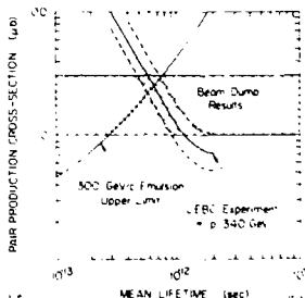
Fig. 35. Results of charm production cross section from the LEBC experiment and comparison with other results.
