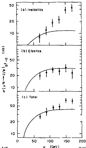
Fig. 34. v distribution of elastic and inelastic J/\psi 's from the EMC collaboration. The curves are predictions of the \gamma g F model (higher lying charmonium states are used as source of inelastic events for the purpose of the calculation).
