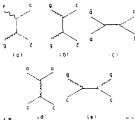
Fig. 1. Typical 1st ord QCD diagrams for open charm production by photons and hadrons: a) \gamma g \rightarrow c\bar{c} , b) g g \rightarrow c\bar{c} , c) q\bar{q} \rightarrow c\bar{c} , d) g \rightarrow c\bar{c} , e) q \rightarrow c\bar{c} .
