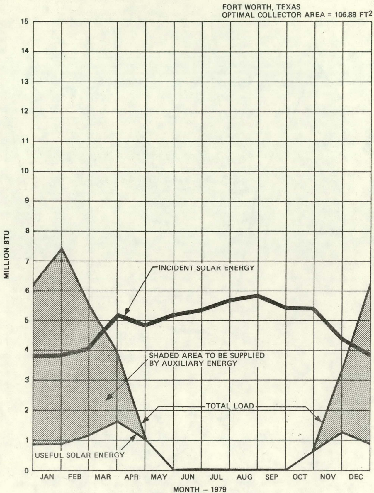
Figure 5.1-2 (c) Thermal Performance of Solar Energy System with Optimized Collector Area for Fort Worth, Texas
