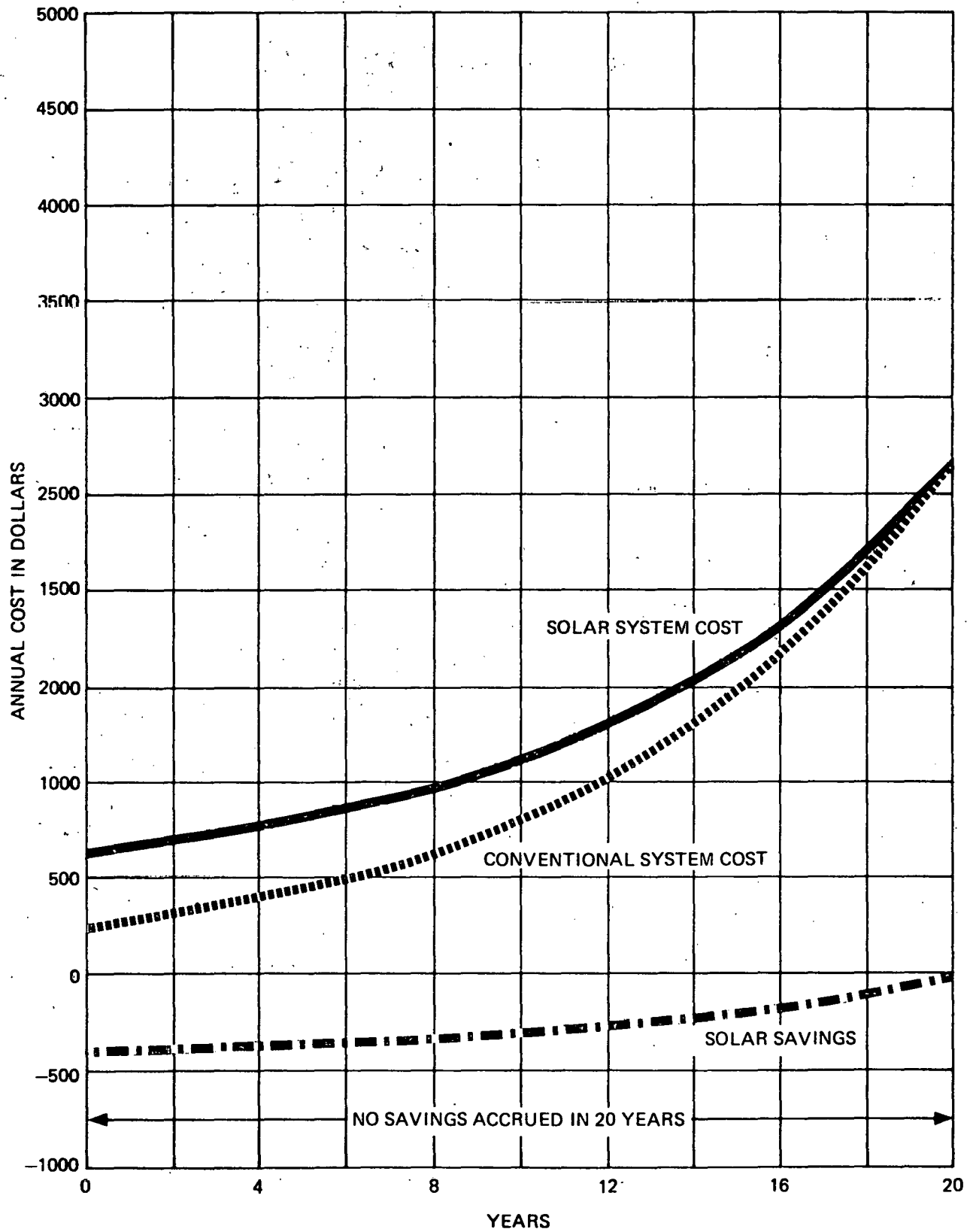
Figure 5.2-2 (a) Annual Expenses for Solar System and Conventional System for Lincoln, Nebraska
