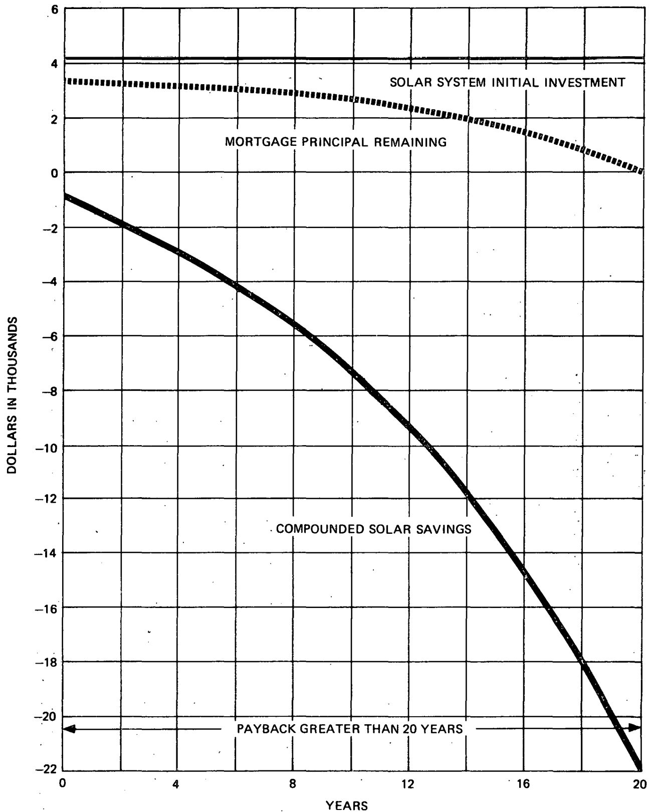
Figure 5.2-3 (e) Payback for Solar Energy System for Washington, D.C.
