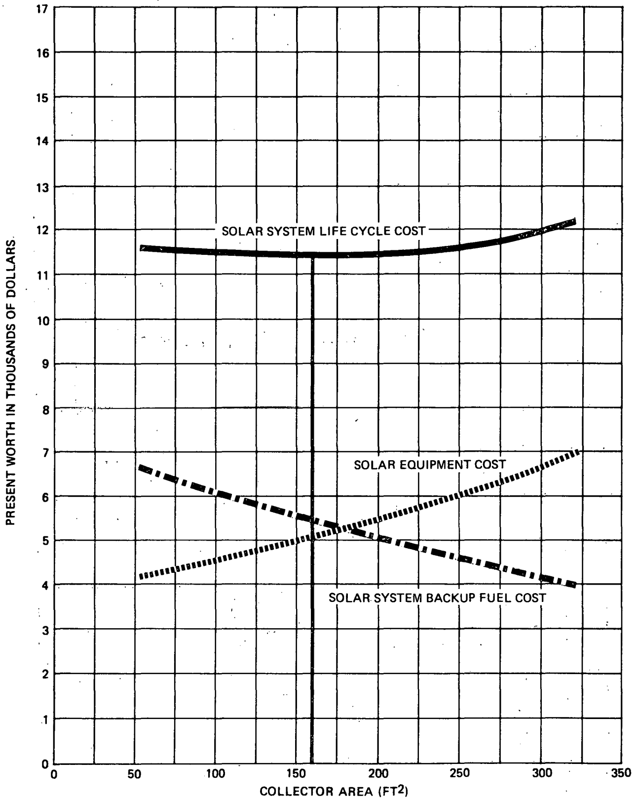
Figure 5.2-1 (a) Optimization of Collector Area for Lincoln, Nebraska
