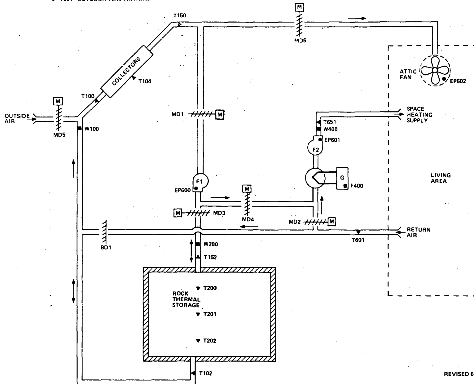
Figure 1. SEECO LINCOLN SOLAR ENERGY SYSTEM SCHEMATIC
