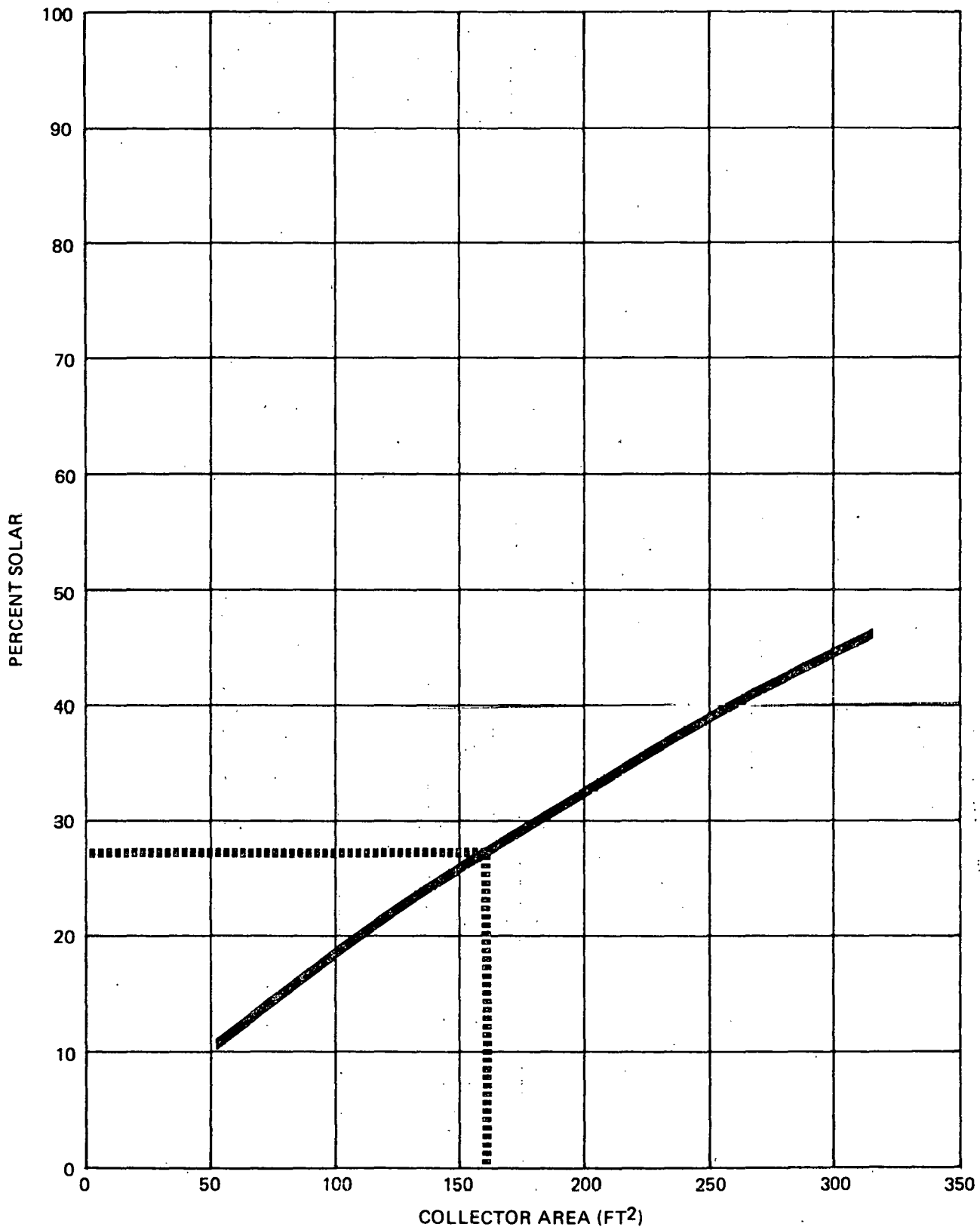
Figure 5.1-1 (a) Solar Fraction vs Collector Area for Lincoln, Nebraska
