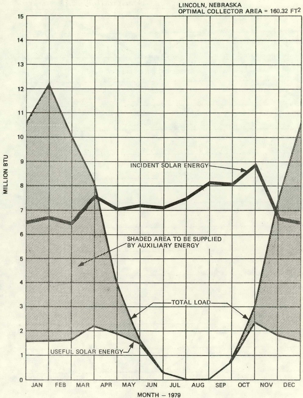
Figure 5.1-2 (a) Thermal Performance of Solar Energy System with Optimized Collector Area for Lincoln, Nebraska
