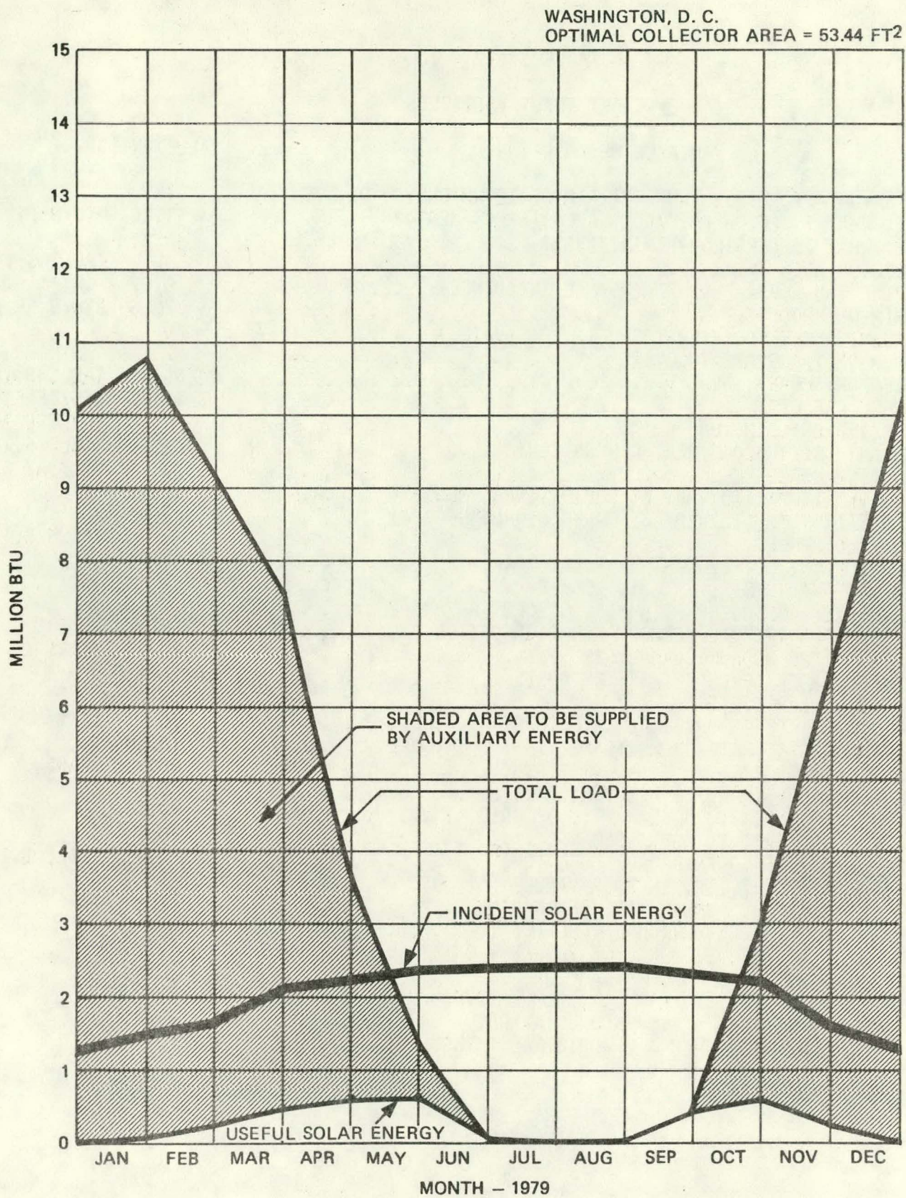
Figure 5.1-2 (e) Thermal Performance of Solar Energy System with Optimized Collector Area for Washington, D. C.
