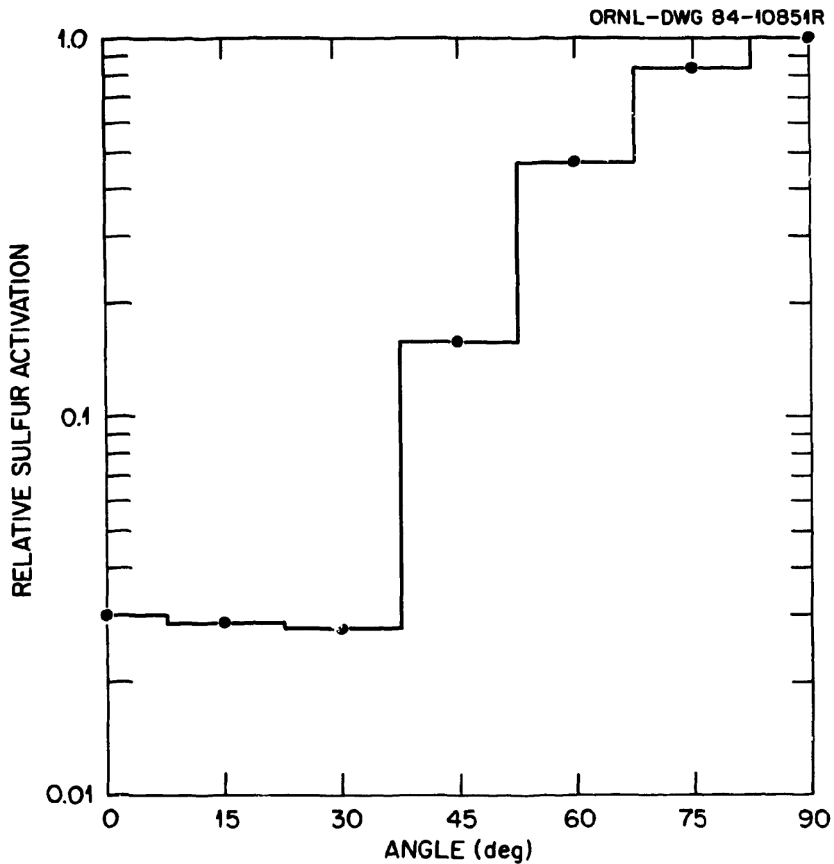
Figure 2. Experimental ORNL data on sulfur activation at 75 cm from the core and at angular intervals of 15° between the nose (0°) and waist (90°) of the reactor (Fig. 1). The data are normalized to sulfur activation at the 90° detector location.
