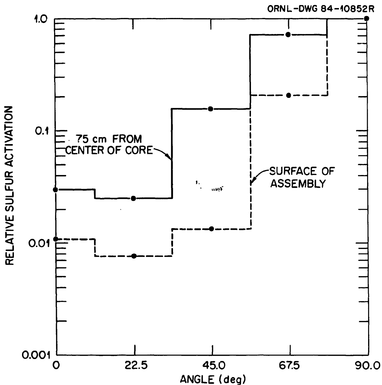
Figure 3. Experimental ORNL data on sulfur activation at the surface and 75 cm from the core and at angular intervals of 22.5° between the nose (0°) and waist (90°) of the reactor (Fig. 1). The data are normalized to sulfur activation at the 90° detector locations.
