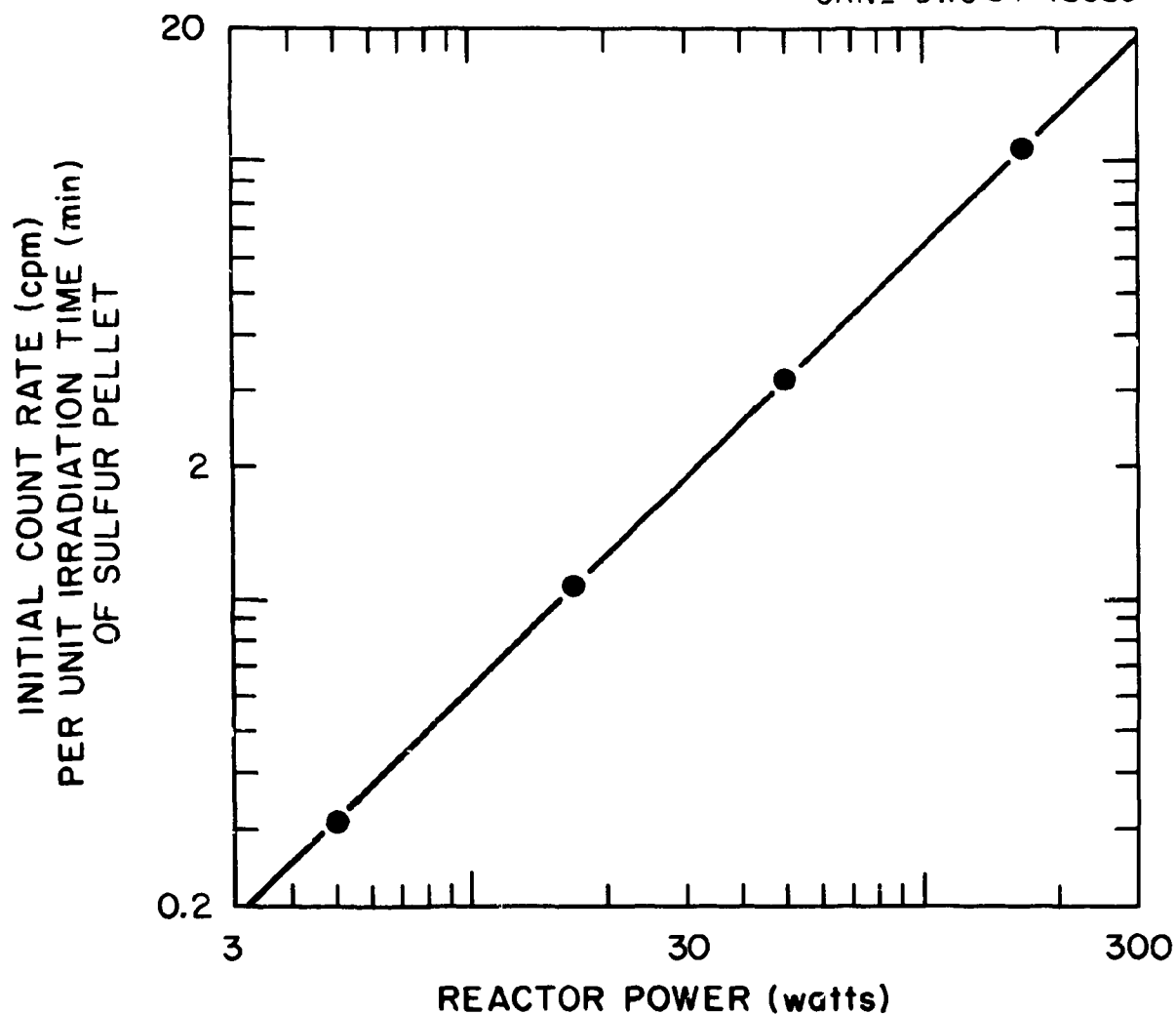
Figure 4. Experimental ORNL data on sulfur activation for varying reactor power levels. The sulfur pellets were exposed at the surface-90° detector location (Fig. 1).
