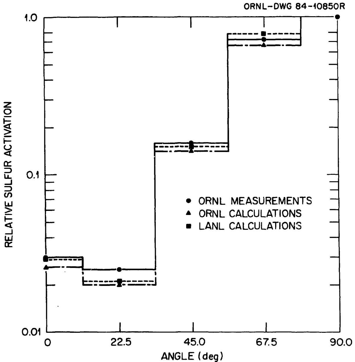
Figure 5. Comparison of measured and calculated data on sulfur activation at 75 cm from the core and at angular intervals of 22.5^\circ between the nose ( 0^\circ ) and waist ( 90^\circ ) of the reactor (Fig. 1). The various data sets are normalized to sulfur activation at the waist detector locations.
