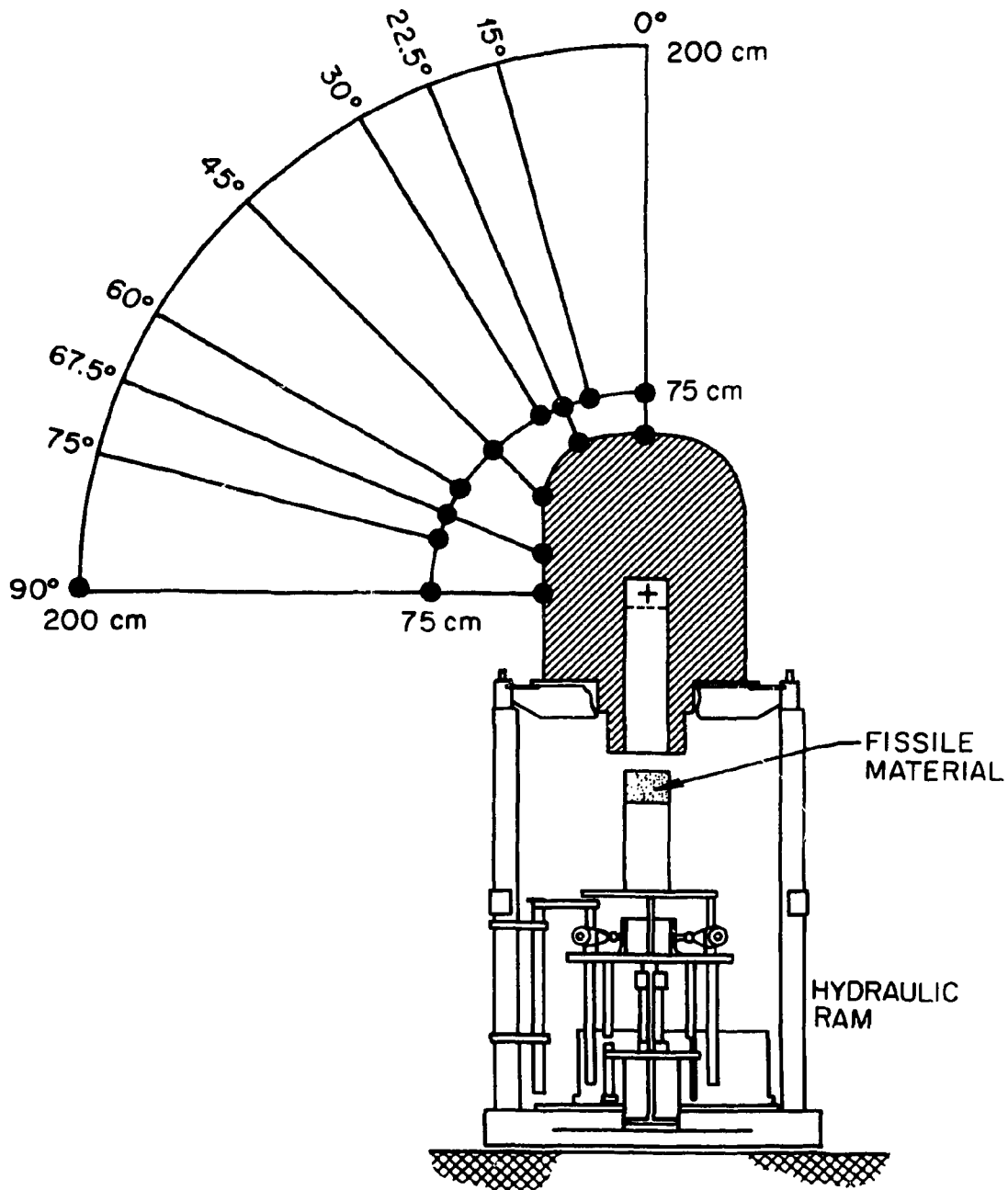
Figure 1. Detector locations (●) used in ORNL measurements of the activation of sulfur by fast neutrons from the Little Boy-Comet Critical Assembly.
