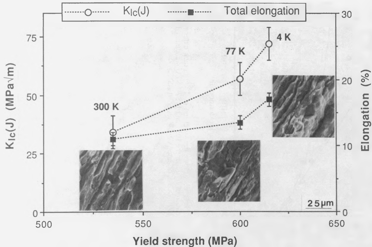
Figure 3.1 Summary of 2090-T81 L strength and L-T toughness combination as a function of temperature. Tensile data were obtained at T/2 . Error bars represent scatter in data. Insets are scanning electron micrographs of fracture surfaces of J_{Ic} specimens used to determine fracture toughness.
