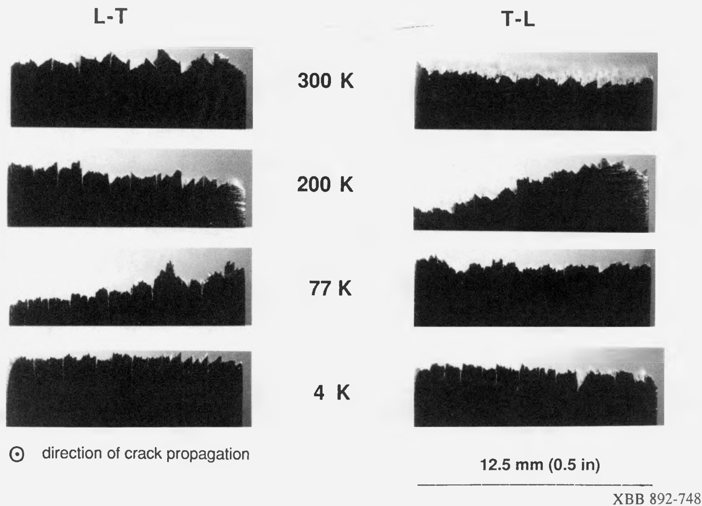
Figure 5.20 Optical micrographs showing fracture profile and splitting in 2091-T8 J c specimens. Specimens were sectioned perpendicular to crack path near the crack initiation point. Cross section shown is the entire thickness of specimen.
