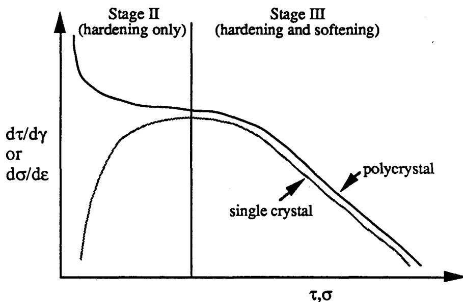
Figure 4.1 Schematic illustration of strain hardening behavior as a function of true stress \sigma (polycrystal) or true shear stress \tau (single crystal) in Stages II and III of deformation. \epsilon and \gamma are the true strain (polycrystal) and true shear strain (single crystal), respectively. (After Mecking, 1975.)
