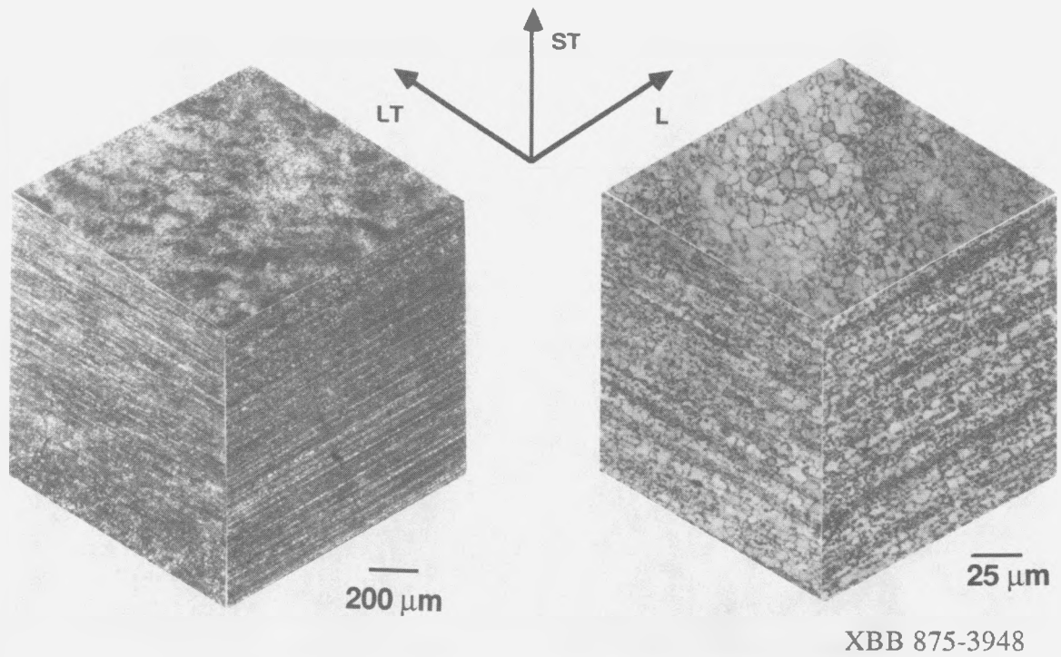
Figure 2.4 Composite optical micrographs showing grain structure of superplastically formable modification of 2090.
