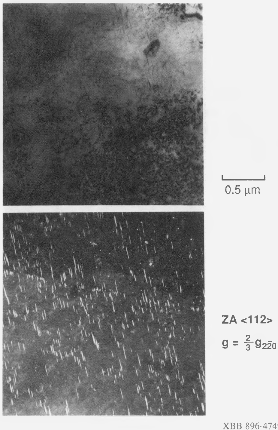
Figure 2.3 Bright-field, dark-field pair of transmission electron micrographs illustrating the microstructure of 2091-T8. The diffraction beam g = \frac{2}{3} g_{22\bar{2}0} corresponds to one variant each of the T_1 and S' precipitates. In the dark-field micrograph, T_1 plates are viewed edge-on as streaks, while S' rods are viewed end-on as dots. The \delta' precipitate is also present.
