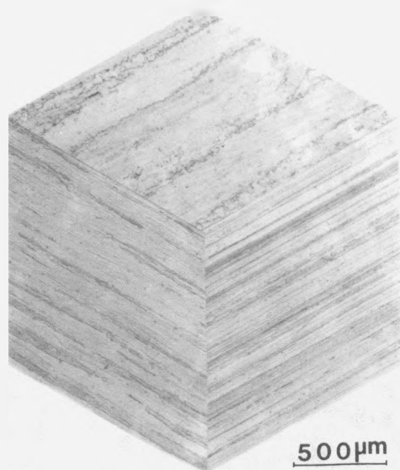
Figure 2.1 Composite optical micrograph showing grain structure of 2090-T81.
