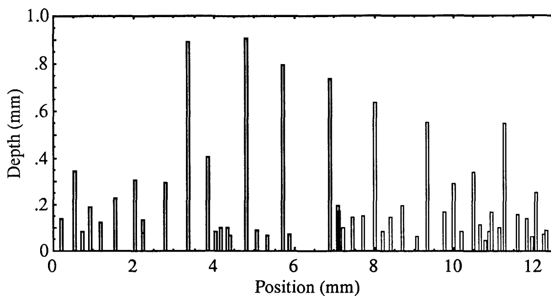
Figure 5.17 Schematic split profile obtained after digitizing splits in optical micrographs of polished cross section of J_{Ic} specimen. Data shown are for a 2090-T81 specimen tested at 77 K in the L-T orientation.
