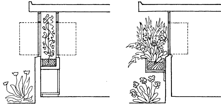
A) SECTION THROUGH PLANTER BETWEEN DOUBLE GLAZING - OPENING STANDARD WINDOWS, STORAGE BELOW PLANTER
