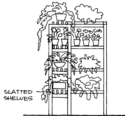
SECTION THROUGH FREESTANDING PLANTER SCREEN
