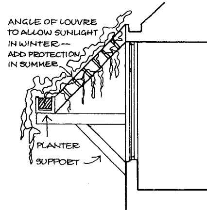
SECTION SHOWING PROTECTED ANGLED WINDOW SHADE
