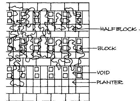
ELEVATION OF CONCRETE BLOCK PLANTER SCREEN USING A COMBINATION OF FULL & HALF BLOCKS
