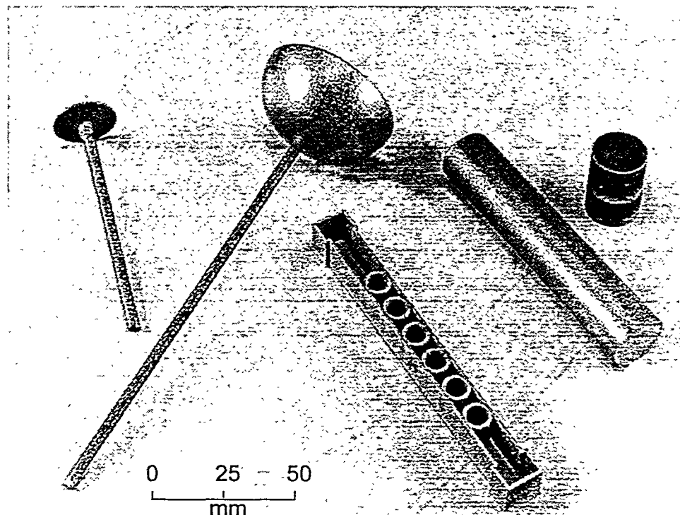
Figure 3. Representative DLF parts and assemblies. From left to right, tantalum stem and disc, 316 stainless steel stem and hemisphere, 316 stainless steel tube assembly and housing, and Inconel 690 solid cylinders.
