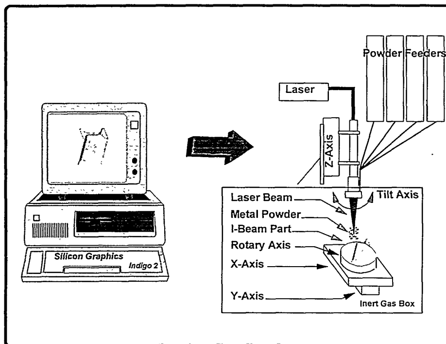
Figure 1. Schematic Diagram of the 5-Axis DLF System
