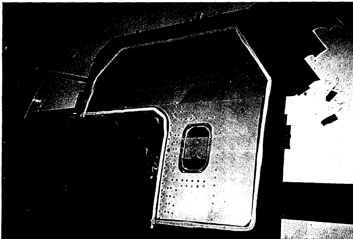
Figure 9 : Anodized Door Corner Prepared for Doubler Bonding Process
