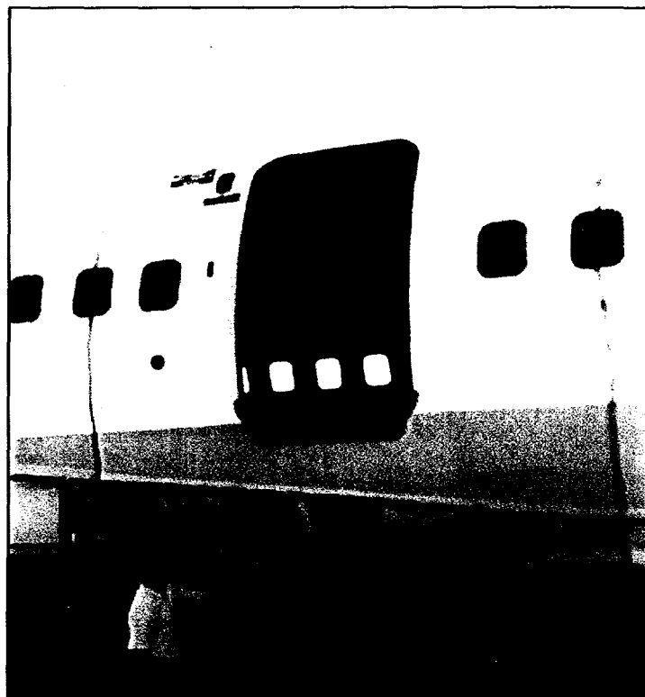
Figure 2: Widebody Fuselage Test Article (L-1011 Door Surround Structure)
