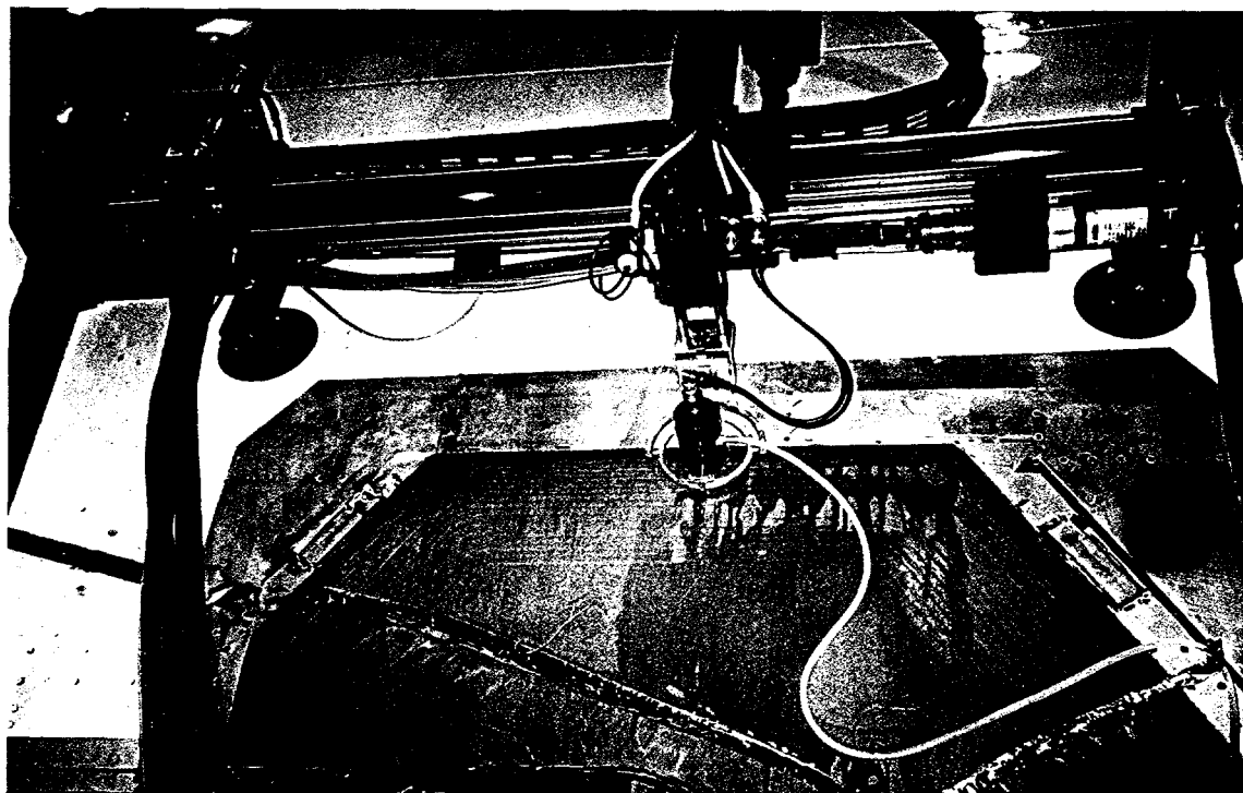
Figure 6: Automated Ultrasonic Scanner Inspecting the Composite Doubler on L-1011 Fuselage
