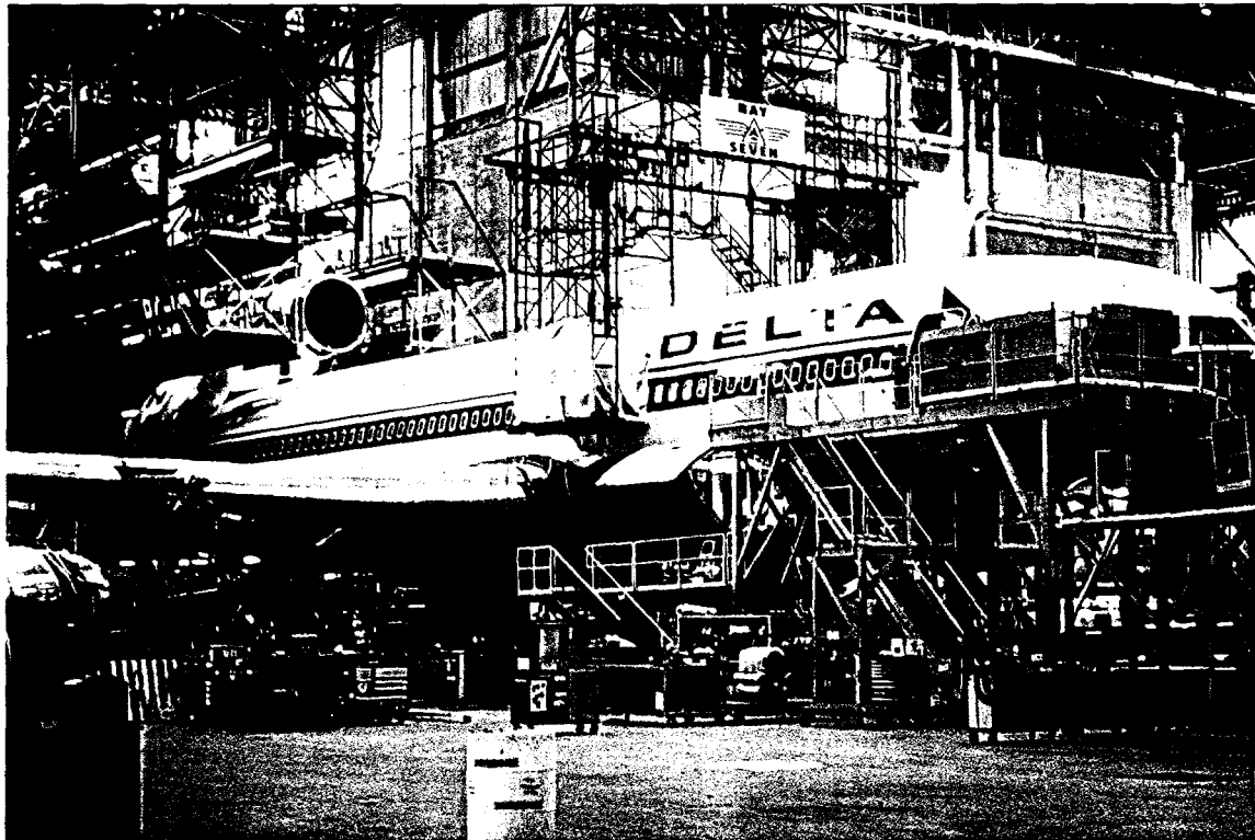
Figure 8 : Delta L-1011 Aircraft During Installation of Composite Doubler; Work Stand is Positioned Next to Right Side Passenger Door
