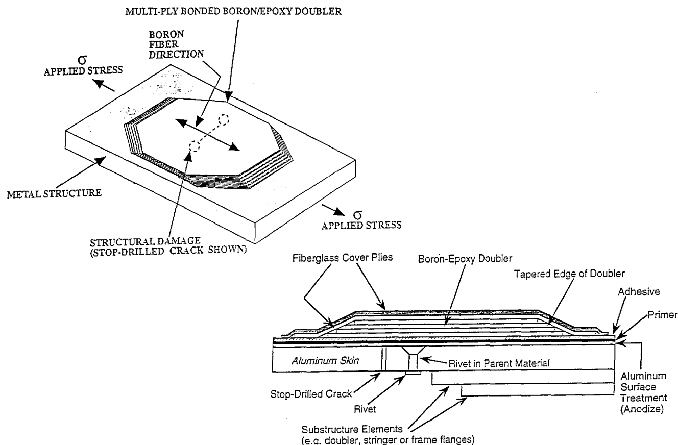
Figure 1: Schematic of Bonded Composite Doubler Installation on an Aluminum Skin
