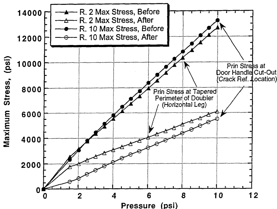
Figure 5: Comparison of Principal Stresses Before and After Doubler Installation
