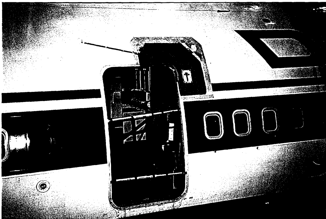
Figure 10: Finished Product - Composite Doubler Following Cure Process
