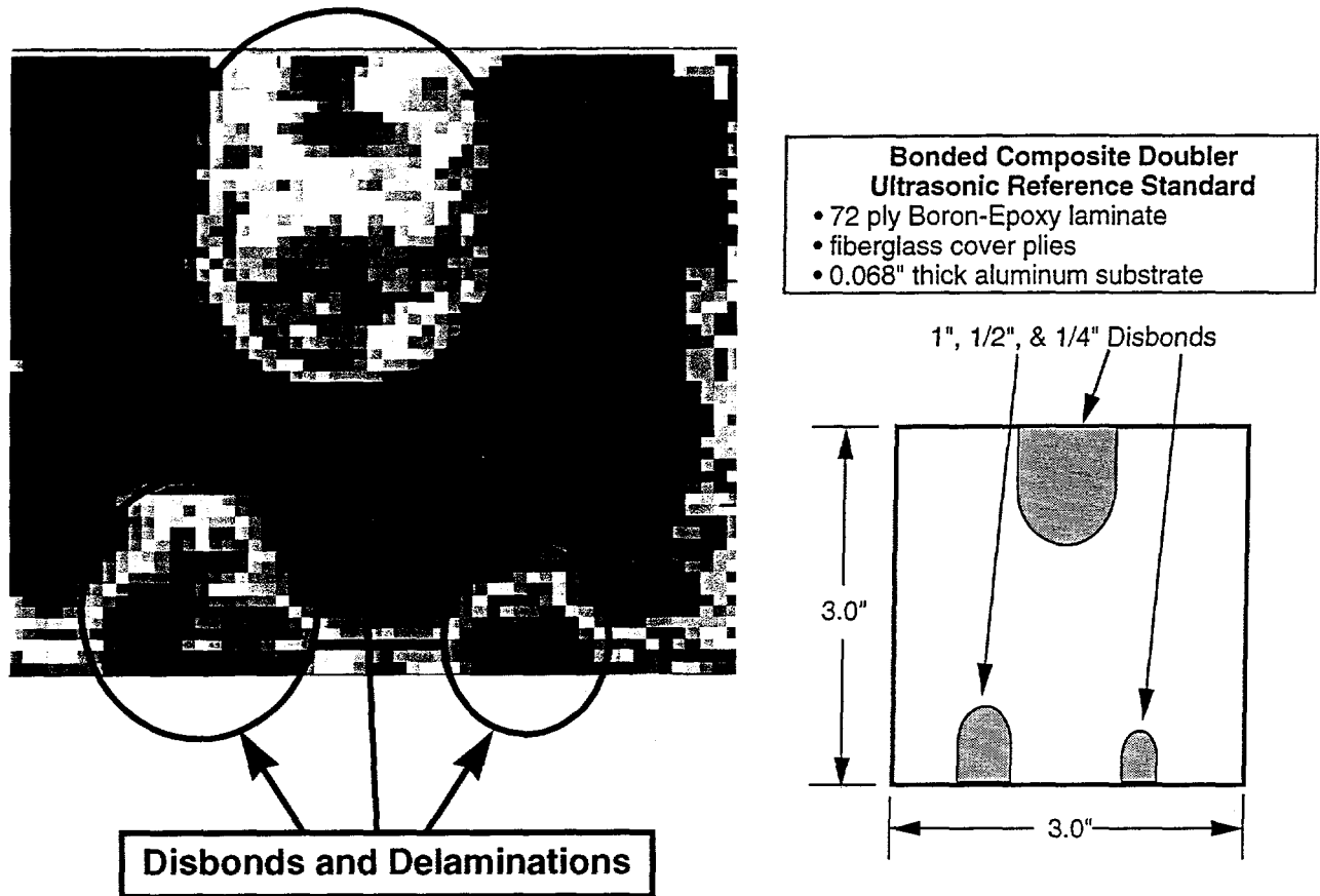
Figure 7: Sample C-Scan Image from Ultrasonic Inspection of 72-Ply Reference Standard Containing Engineered Flaws
