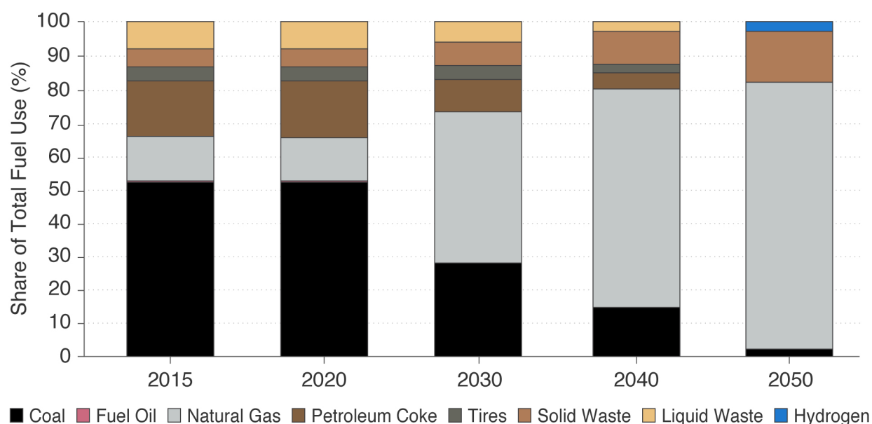
FIGURE A 11. FUEL MIX PROJECTIONS FOR THE U.S. CEMENT INDUSTRY UNDER NEAR ZERO GHG SCENARIO, 2015-2050
