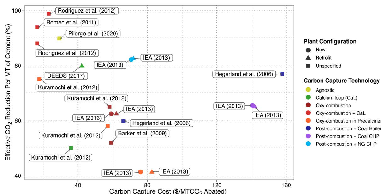
FIGURE 56. ESTIMATES OF COST OF CO 2 AVOIDED AND CORRESPONDING EFFECTIVE CO 2 REDUCTION RATE USING VARIOUS CARBON CAPTURE TECHNOLOGIES IN CEMENT PRODUCTION AS REPORTED IN LITERATURE. 317
