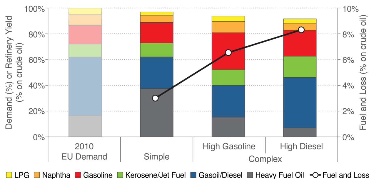
FIGURE 38. TYPICAL PRODUCT YIELD AND ENERGY INTENSITY FOR EU REFINERIES OF DIFFERENT COMPLEXITY 269
