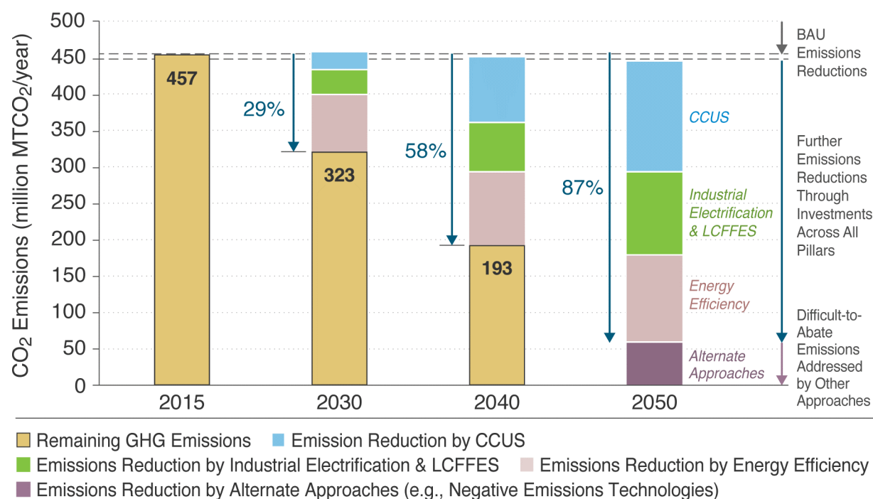
FIGURE 60. CO 2 EMISSIONS REDUCTION POTENTIAL (MILLION MT) THROUGH THE APPLICATION OF THE DECARBONIZATION PILLARS FOR THE U.S. IRON AND STEEL, CHEMICAL, FOOD, PETROLEUM REFINING, AND CEMENT MANUFACTURING SUBSECTORS (EXCLUDING FEEDSTOCKS).
