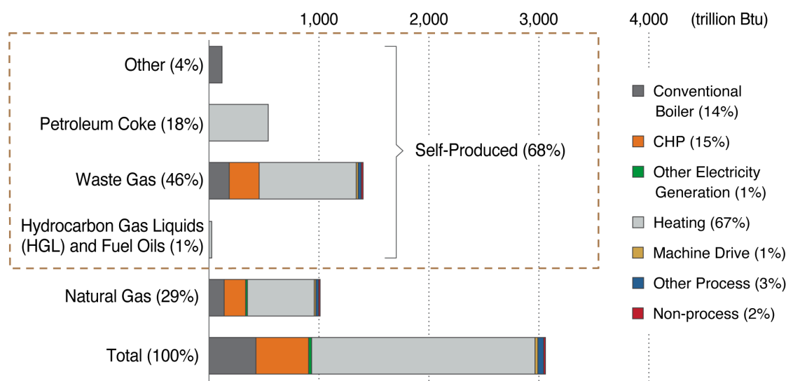
FIGURE 39. FUEL ENERGY CONSUMPTION AT U.S. PETROLEUM REFINERIES IN 2018, BROKEN OUT BY FUEL AND END USE 272
