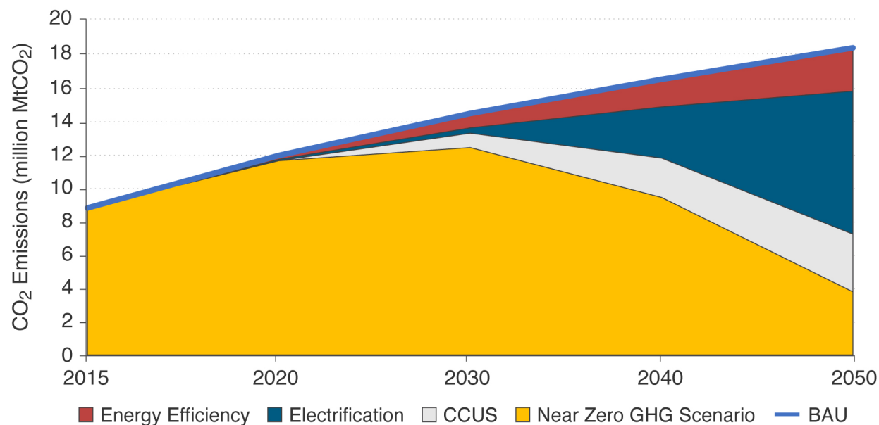
FIGURE A 8. AREA PLOT OF PILLAR CONTRIBUTIONS TO CO 2 REDUCTION FOR THE AMMONIA INDUSTRY.
