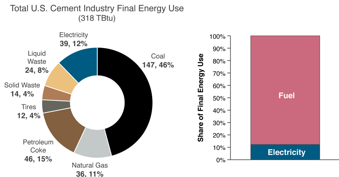
FIGURE 47. ENERGY MIX IN THE U.S. CEMENT INDUSTRY IN 2015.
