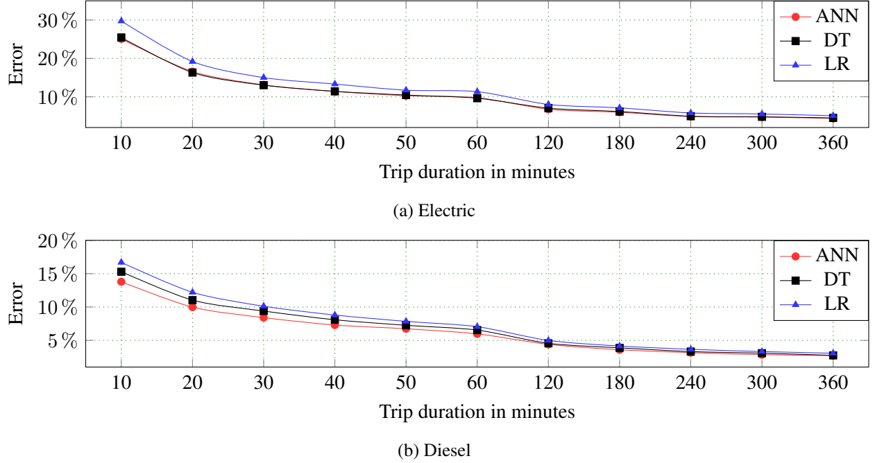
Figure 7: Energy prediction error for longer trips, consisting of many samples, with neural network (ANN), decision tree (DT), and linear regression (LR).
