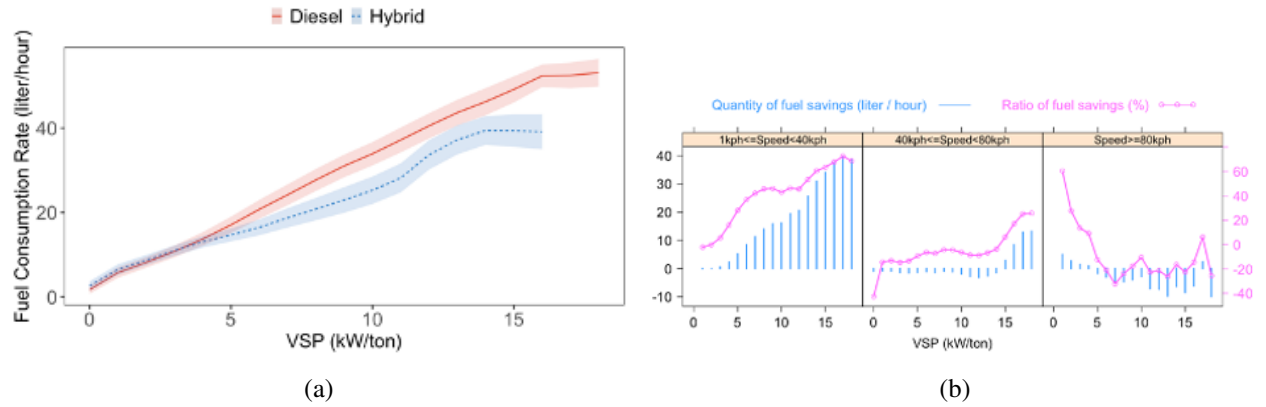
Figure 10: (a) Mean fuel rate (liter per hour) and 95% confidence interval (shaded area) for diesel and hybrid bus as a function of instantaneous vehicle specific power bins from 0 to 18 kW/ton with 1 kW/ton interval. (b) Fuel savings of hybrid buses as compared with diesel buses by driving speed and instantaneous vehicle specific power bins.
