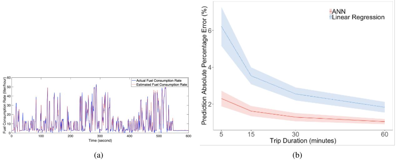
Figure 11: (a) Second-by-second actual fuel consumption rate (liter per hour) versus estimated fuel consumption rate for one trip. (b) Mean absolute percentage error and 95 percentage confidence intervals for predictions of artificial neural network (ANN) model and linear regression model with the same independent variables as a function of trip duration.
