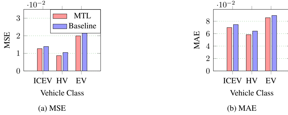
Figure 13: (a) MSE and (b) MAE of MTL model compared to vehicle-specific neural network models (baseline) on testing set. Prediction target: emissions (kg CO 2 ).
