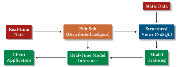
Figure 2: HD-EMMA data architecture overview.
