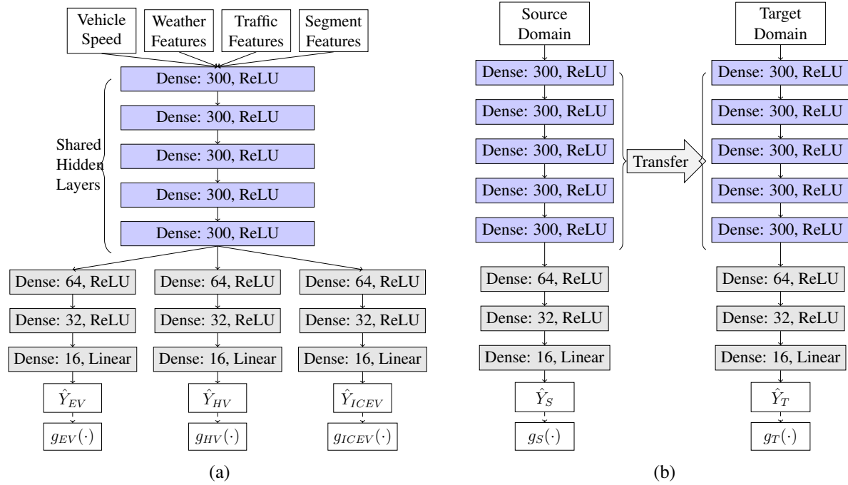
Figure 12: (a) MTL Model: DNN with hard parameter sharing for predicting emissions (kg CO 2 ) of EVs ( \hat{Y}_{EV} ), HVs ( \hat{Y}_{HV} ) and ICEVs ( \hat{Y}_{ICEV} ). (b) ITL Model: shared-hidden layer parameters are frozen and transferred to the target model. Energy consumed (kWh) is a linear function g_i(\cdot) for vehicle class i .
