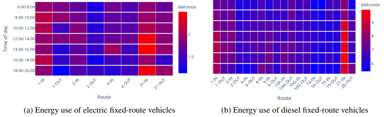
Figure 3: Average energy used in kWh/mile by trip and by the time of day for (a) electric and (b) diesel fixed-route transit vehicles. Scale for diesel is between 5-10 KWh/mile; scale for electric is between 0.7-3 KWh/mile. The variance shows that there are specific trips that are more energy efficient with electric vehicles than others. Further, there are specific routes like 21-inbound where using an EV will have a higher impact than other routes. All of these differences factor into the optimization problem.
