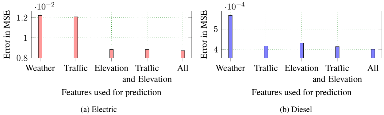
Figure 6: Mean squared error for energy prediction with various sets of features. Note that electric and diesel energy are measured in different units. The predictions are based on artificial neural networks.
