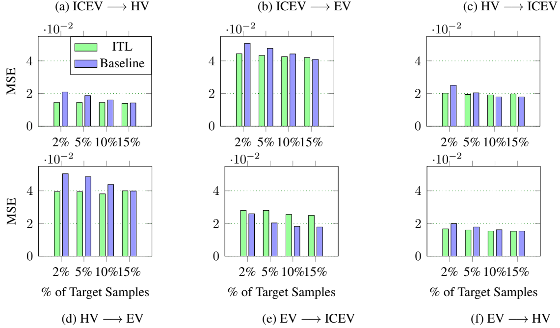
Figure 14: ITL models compared to corresponding baselines. ITL model is trained on full dataset in the source vehicle class and is evaluated on the target vehicle class (source \rightarrow target). Average MSE compared to fraction of data samples used for training in the target vehicle class. Prediction target: emissions (kg CO 2 ).
