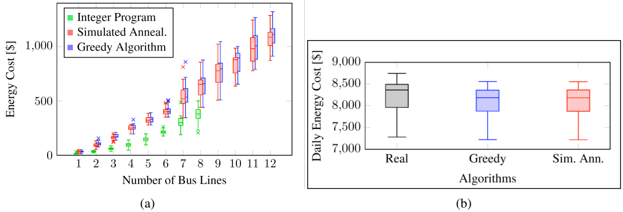
Figure 15: (a) Energy costs for assignments using the integer program, simulated annealing, and greedy algorithm for various number of bus lines. (b) Energy costs for assignments using the greedy algorithm and simulated annealing for complete daily schedules, compared to existing real-world assignments.
