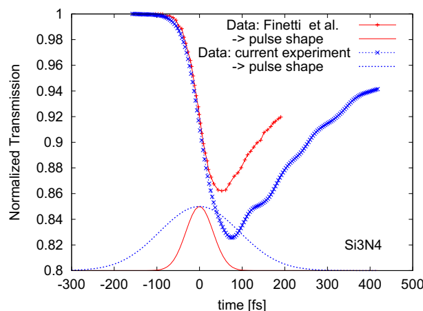
Figure 1. Normalized transmissivity, T(t)/T_{\text{equib}} of XUV irradiated \text{Si}_3\text{N}_4 recorded in the experiment performed at the FERMI facility by Finetti et al. 3 (pulse duration of 75 fs FWHM) and in our current experiment (pulse duration of 220 fs FWHM), when probed with the optical pulses of wavelength \lambda = 630 nm. Temporal profiles of XUV pulses are also schematically depicted. The experimental data represent averages over at least 600 single shots.
