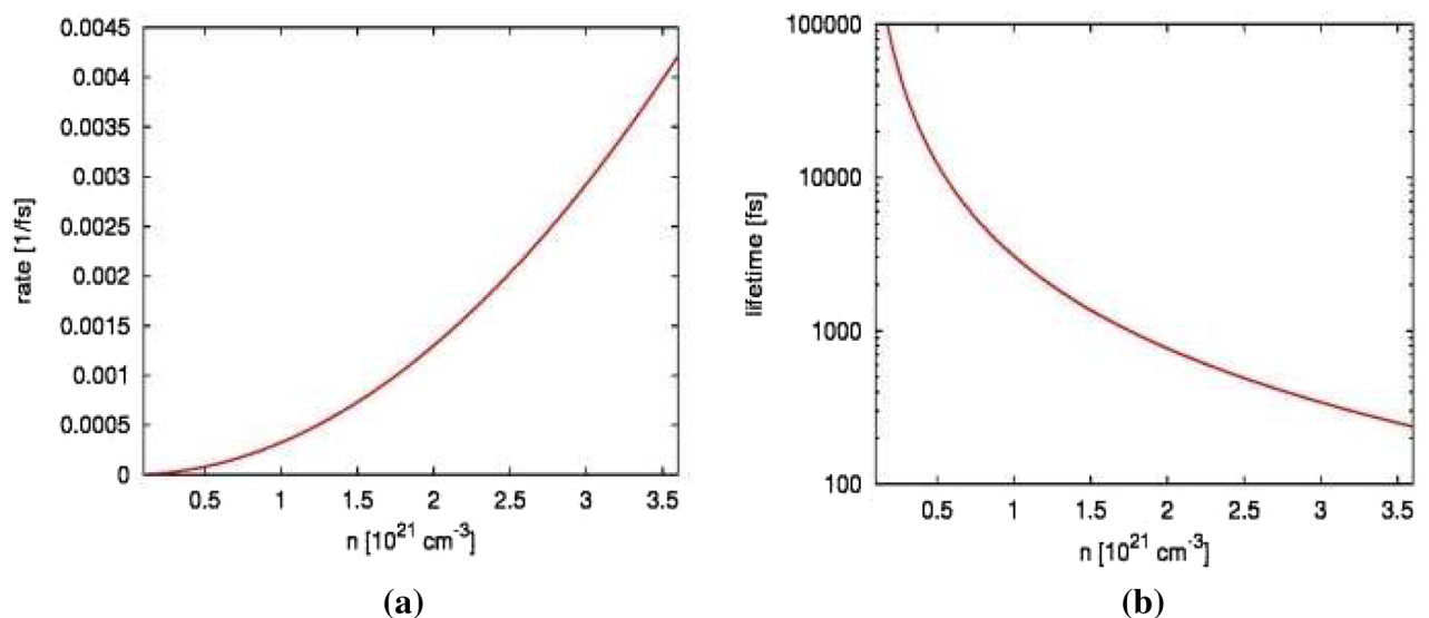
Figure 5. (a) The effective recombination rate, C_{\text{AR}} \cdot n^2 , and (b) the respective lifetime, \tau_{\text{AR}} = 1/(C_{\text{AR}} \cdot n^2) for C_{\text{AR}} \approx 3.25 \cdot 10^{-31} \text{ cm}^6/\text{s} plotted as a function of free electron density, n within the regime of n relevant for this study.
