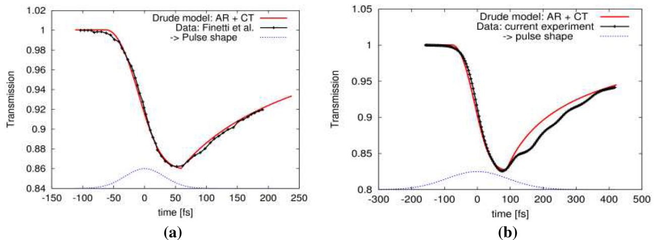
Figure 4. Normalized transmissivity, T(t)/T_{\text{equip}} of XUV irradiated \text{Si}_3\text{N}_4 recorded in the experiment performed at: (a) the FERMI facility by Finetti et al. 3 (pulse duration of \sim 75 fs FWHM), and (b) in our current experiment (pulse duration of \sim 220 fs FWHM), when probed with the optical pulses of wavelength \lambda = 630 nm. The experimental data represent averages over at least 600 single shots. They are compared with the results of the simulation in case when the Auger recombination (AR) and carrier transport (CT) were taken into account. Temporal profile of XUV pulses is also schematically depicted.
