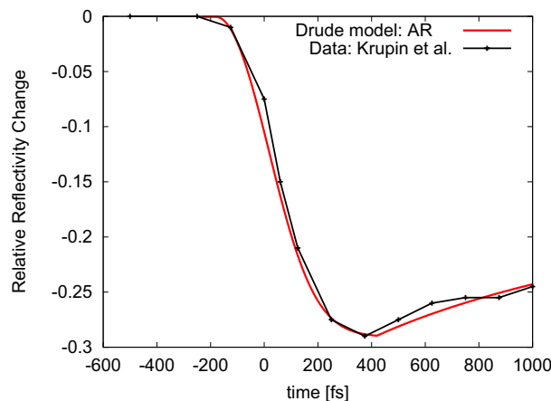
Figure 6. Relative change of reflectivity, (R(t) - R_{\text{equib}})/R_{\text{equib}} in soft X-ray irradiated \text{Si}_3\text{N}_4 recorded in the experiment by Krupin et al. 7 (Fig. 3 therein). The data were averaged over many single shots. FEL photon energy was 540 eV. Note that the XFEL pulse duration ( \sim 50 – 150 fs FWHM) was not precisely measured in this experiment. Also, the time 'zero' denotes here the time instant when the reflectivity starts to decrease. The probe pulse wavelength was \lambda = 800 nm. The published data reproduced from Ref. [8] are then compared to the results of our calculations in which only the Auger recombination (AR) was taken into account.
