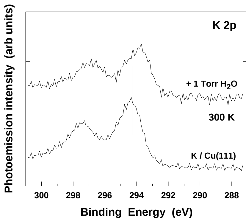
Figure 2. K 2p XPS spectra recorded before and after exposing a K/Cu(111) surface to to 1 Torr of water at 300 K for five minutes. The coverage of K in the K/Cu(111) system was \sim 0.15 ML.
