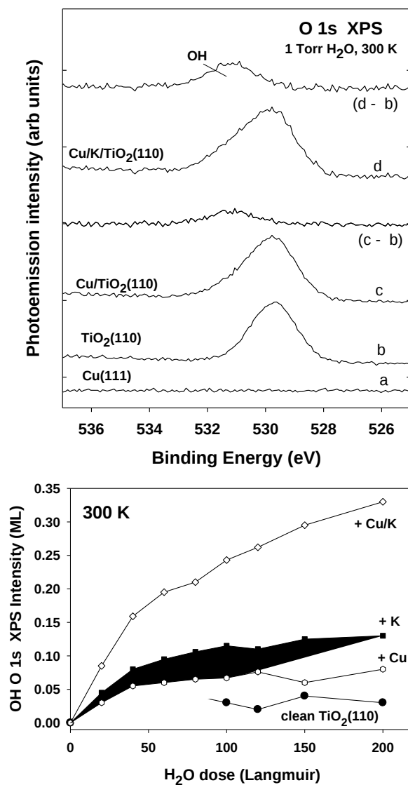
Figure 6. Formation of adsorbed OH by water dissociation at 300 K on Cu(111), TiO 2 (110), K/TiO 2 (110) ( \Theta_K \sim 0.15 ML), Cu/TiO 2 (110) ( \Theta_{Cu} \sim 0.3 ML), and Cu/K/TiO 2 (110) ( \Theta_{Cu} \sim 0.3 ML; \Theta_K \sim 0.15 ML). The surfaces were exposed to water under UHV conditions, bottom panel, or to 1 Torr of water for five minutes in a batch reactor, top panel.
