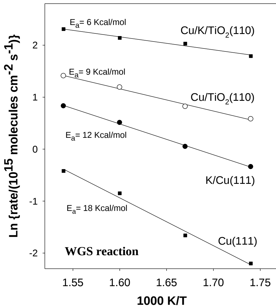
Figure 5. Arrhenius plots for the water-gas shift on Cu(111), K/Cu(111) ( \Theta_K \sim 0.2 \text{ ML} ), Cu/TiO 2 (110) ( \Theta_{Cu} \sim 0.3 \text{ ML} ), and Cu/K/TiO 2 (110) ( \Theta_{Cu} \sim 0.3 \text{ ML} ; \Theta_K \sim 0.15 \text{ ML} ). Reaction conditions: 20 Torr of CO. 10 Torr of water.
