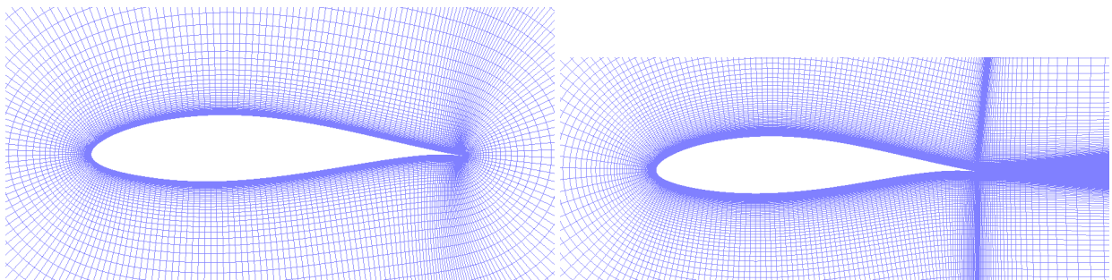
Figure 4.3. Close up of the airfoil section of both O-type (left) and C-type (right) grids for NACA 63 3 -418 airfoil.
