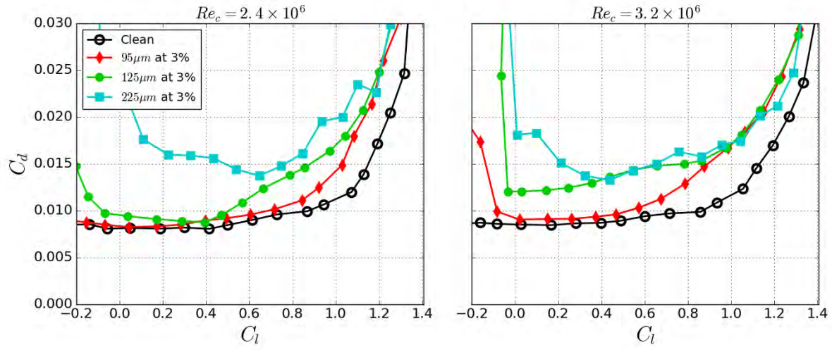
Figure 3.14. Effect of roughness height on lift and drag, S814 airfoil, 95\mu\text{m} , 125\mu\text{m} , 225\mu\text{m} heights, all at 3% distribution density and from tunnel entry 7.
