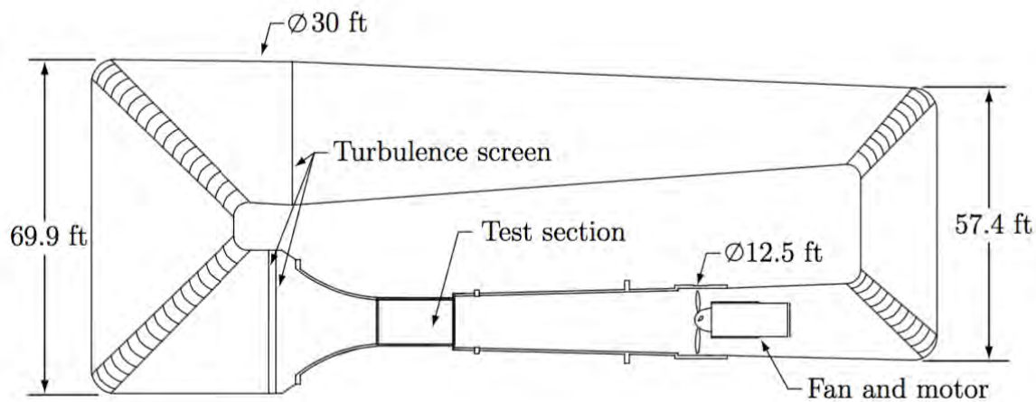
Figure 3.1. Overview of the Oran W. Nicks Low Speed Wind Tunnel.
