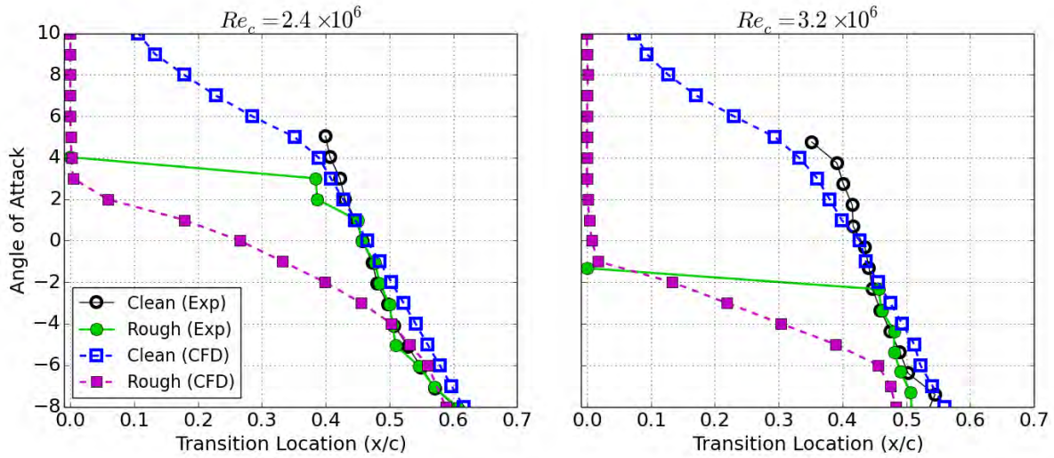
Figure 7.32. Comparison of upper surface transition location prediction with experimental results, S814 airfoil, k/c = 154 \times 10^{-6} roughness applied from x/c = -0.14 : 0.025 , distribution density 3%, k_s/c = 80 \times 10^{-6} input into roughness model.
