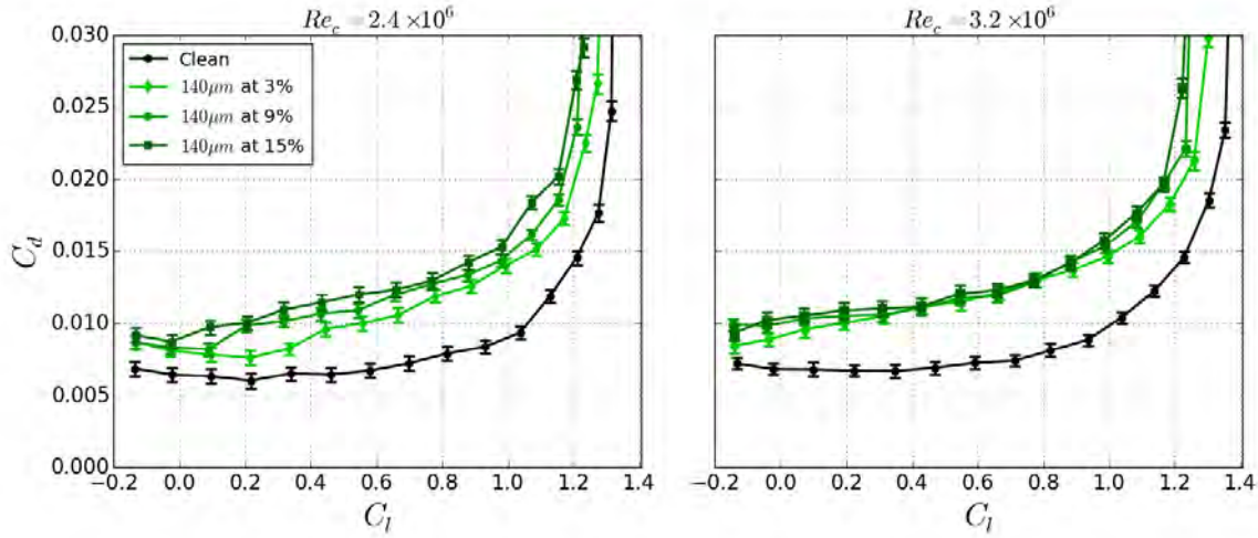
Figure 3.12. Effect of roughness distribution density on lift and drag, NACA 63-418, 3%, 9%, and 15% distribution densities, all at 140\mu\text{m} height and from tunnel entry 3.
