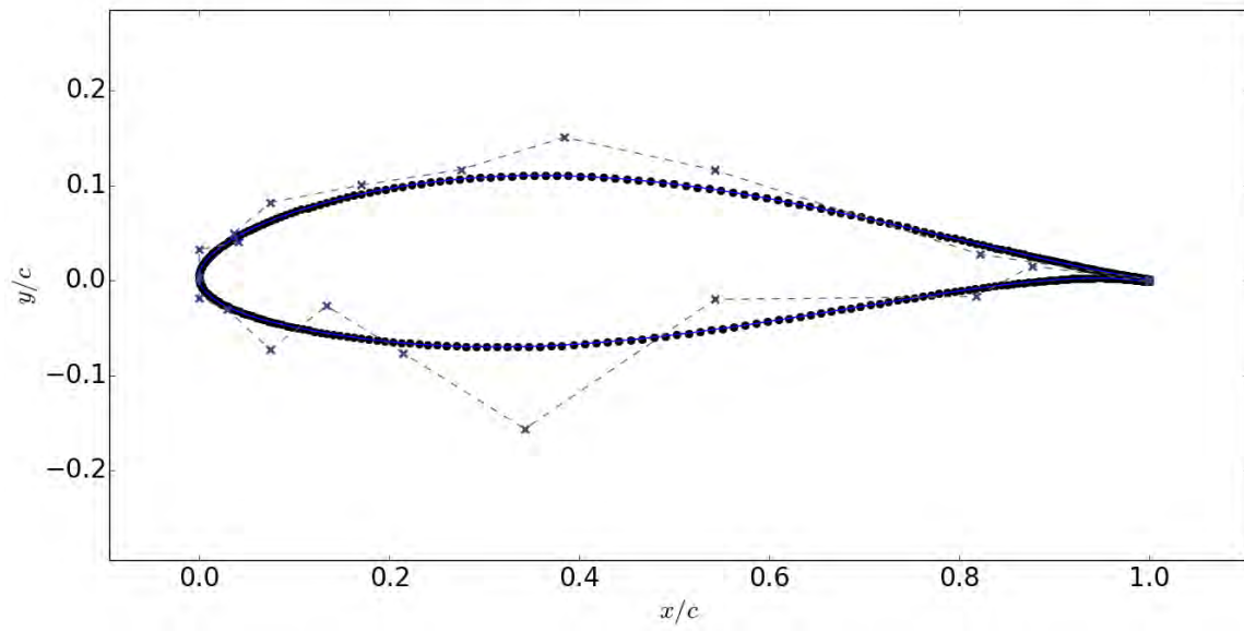
Figure 4.4. Graphical representation of Bezier curves used for NACA 63 3 -418 airfoil, control points indicated by x's with the dashed line connecting them.
