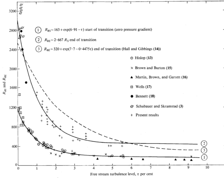
Figure 2.4. Plot of Re_{\theta_t} correlations against freestream turbulence intensity, adapted from Abu-Ghannam and Shaw [24]
