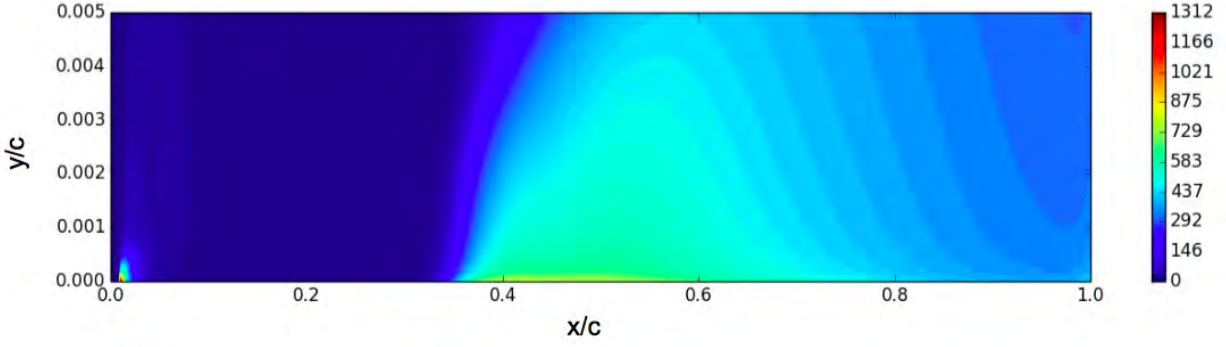
Figure 7.1. Contours of A_r over rough flat plate, k_s/c = 200 \times 10^{-6} , Re_c = 1.3 \times 10^6 , zero pressure gradient, roughness applies x/c = 0.02 - 1.0
