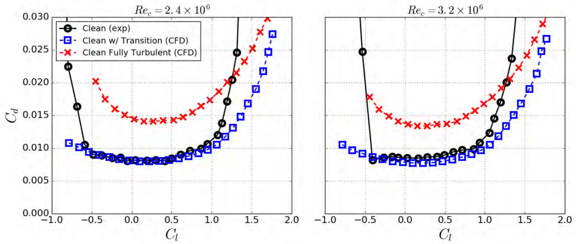
Figure 5.16. Drag polar for S814, experimental results taken from tunnel entries at Texas A&M, freestream turbulence set to 0.75%.
