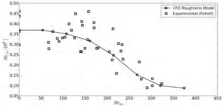
Figure 7.8. Roughness Reynolds number ( Re_{k_s} ) plotted against location of transition onset ( Re_{xt} ) for flat plate, adverse pressure gradient.
