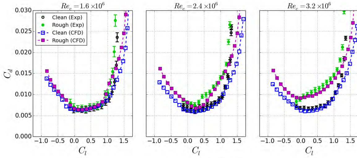
Figure 7.29. Predicted drag polars compared to experimental results, NACA 633-418 airfoil, k/c = 172 \times 10^{-6} roughness applied from x/c = -0.13 : 0.02 , distribution density 3%, k_s/c = 70 \times 10^{-6} input into roughness model.
