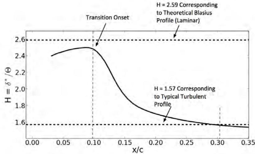
Figure 7.17. Plot of boundary layer shape factor along chord, NACA 0012 airfoil, Re_c = 1.25 \times 10^6 , \alpha = 0^\circ , Tu = 0.1\% , distributed roughness applied x/c = 0.0314 - 0.0539
