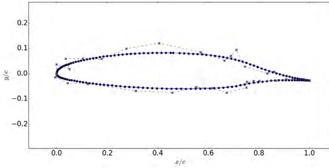
Figure B.3. Graphical representation of Bezier curves used for NLF(1)-0414F airfoil, control points indicated by x's with the dashed line connecting them.
