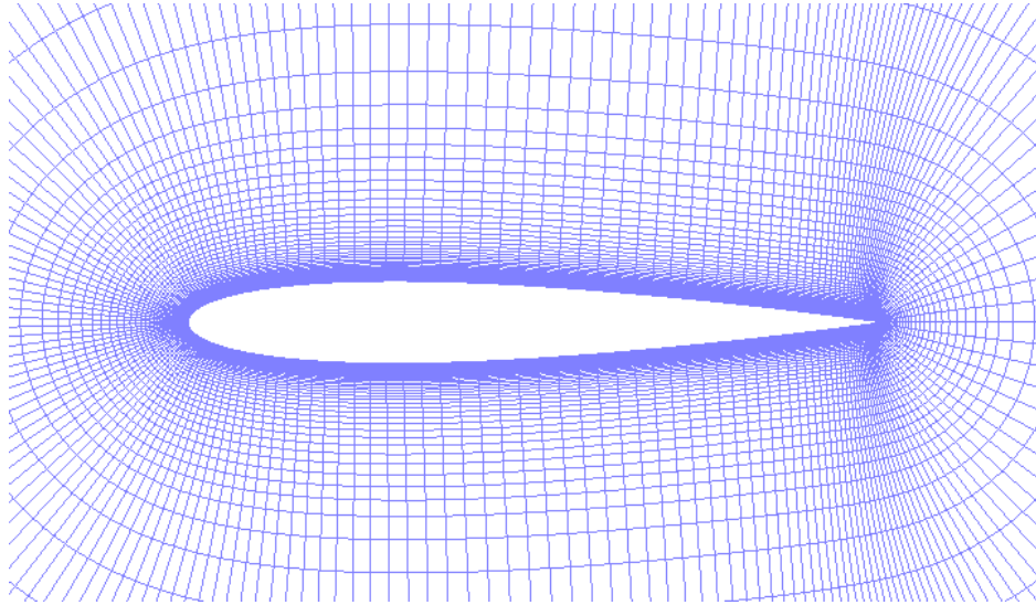
Figure 7.13. Grid used for NACA 0012 simulations, every other grid line shown for clarity.
