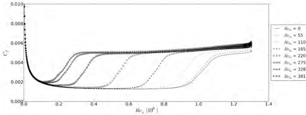
Figure 7.9. The effect on local skin friction coefficient ( C_f ) of varying Re_{ks} . Flat plate, favorable pressure gradient, freestream turbulence intensity = 2.10%.
