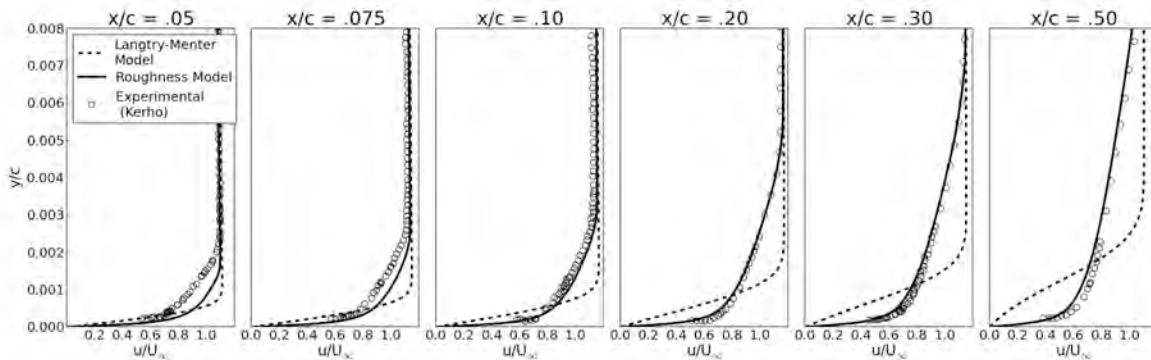
Figure 7.15. Boundary layer profiles: Kerho [54], unmodified Langtry-Menter transition model, computational roughness model. NACA 0012 airfoil, Re_c = 1.25 \times 10^6 , \alpha = 0^\circ , Tu = 0.1\% , distributed roughness applied x/c = 0.0061 - 0.0258
