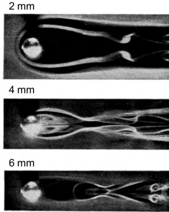
Figure 2.6. Details of the horseshoe vortex system using smoke streaks at various heights, the hairpin structure can also be seen, adapted from Mochizuki [46]
