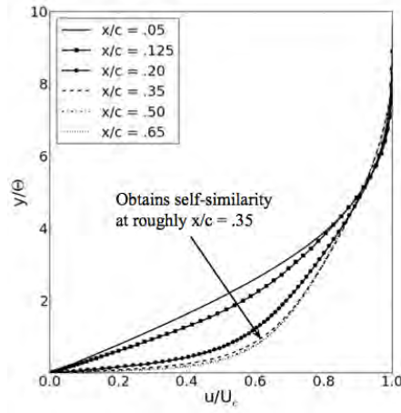
Figure 7.18. Plot of boundary layer normalized by momentum thickness at several chord locations, NACA 0012 airfoil, Re_c = 1.25 \times 10^6 , \alpha = 0^\circ , Tu = 0.1\% , distributed roughness applied x/c = 0.0314 - 0.0539
