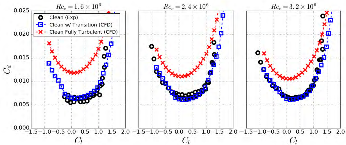
Figure 5.14. Drag polar for NACA 633-418, experimental results taken from multiple tunnel entries at Texas A&M, freestream turbulence set to 0.75%.
