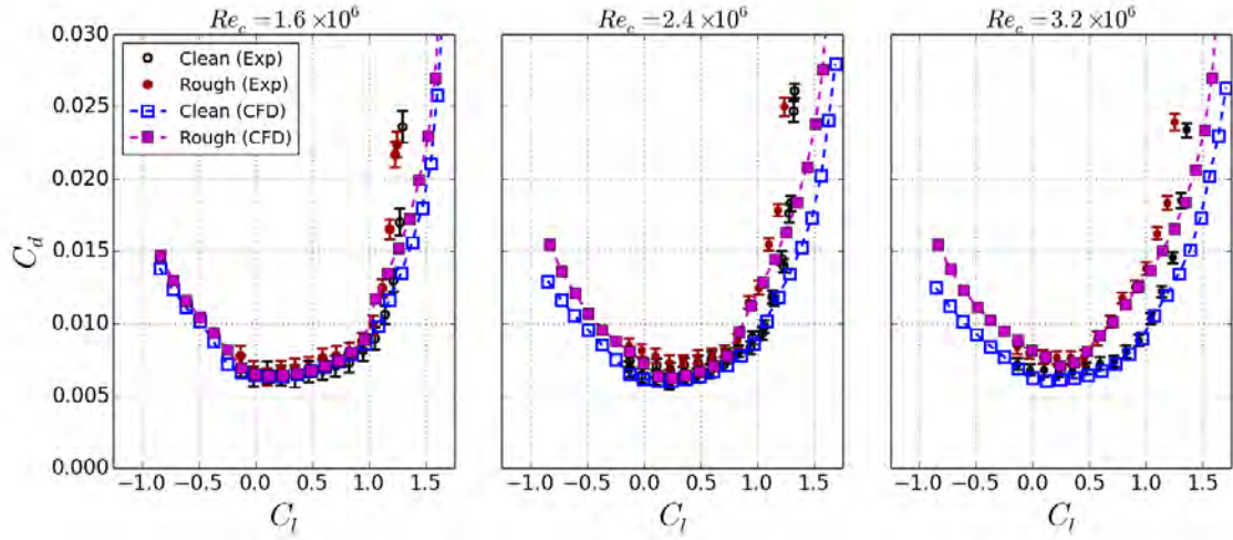
Figure 7.24. Predicted drag polars compared to experimental results, NACA 63 3 -418 airfoil, k/c = 123 \times 10^{-6} roughness applied from x/c = -0.13 : 0.02 , distribution density 15%, k_s/c = 57 \times 10^{-6} input into roughness model.
