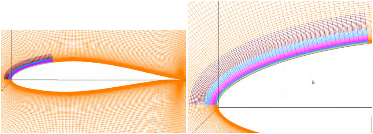
Figure 6.2. Sketch of domain partition used in integrated norm for function optimization.
