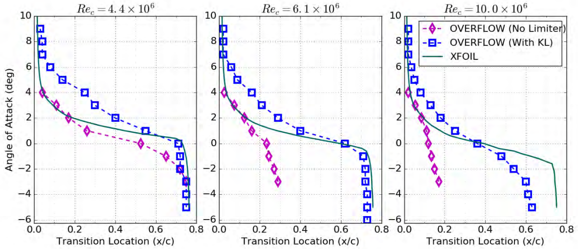
Figure 5.12. Comparison of upper surface transition location at three different Reynolds numbers for both an e^N type and local correlation method on the NLF(1)-0414F airfoil. Freestream turbulence level set to 0.05% for \gamma - \tilde{Re}_{\theta t} model, N_{crit} = 9 used for XFOIL.
