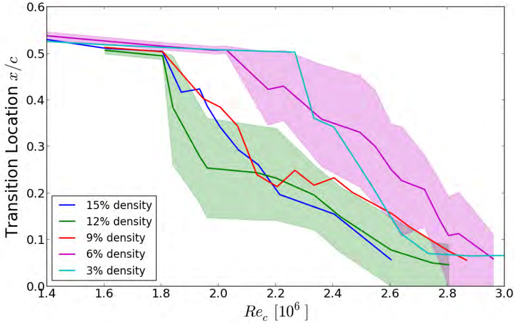
Figure 3.13. The effect of roughness distribution density on transition location, NACA 63 3 -418 airfoil, 140 \mu m roughness height from tunnel entry 2, angle of attack fixed at 0 degrees, Re_c varied by increasing freestream velocity, 25% and 75% transition bands shown on the 12% and 6% density cases.
