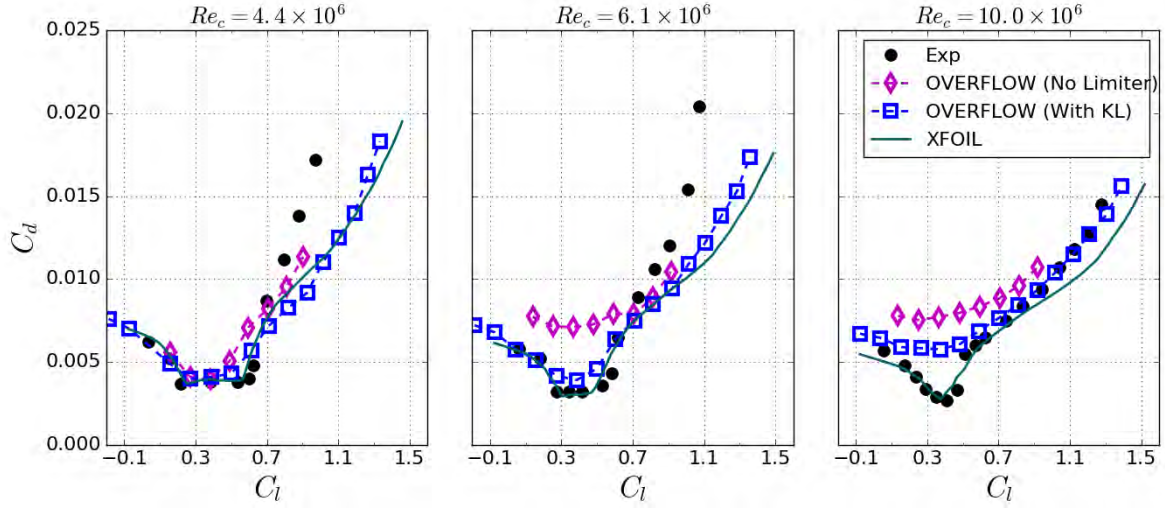
Figure 5.11. Comparison of lift and drag at three different Reynolds numbers for both an e^N type and local correlation method on the NLF(1)-0414F airfoil. Freestream turbulence level set to 0.05% for \gamma - \tilde{Re}_{\theta t} model, N_{crit} = 9 used for XFOIL.
