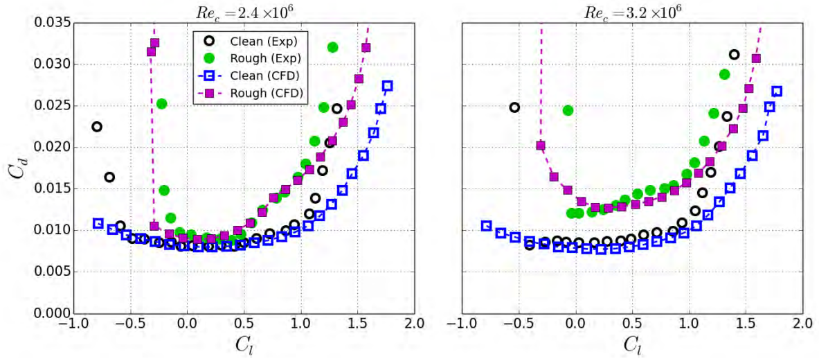
Figure 7.33. Predicted drag polars compared to experimental results, S814 airfoil, k/c = 154 \times 10^{-6} roughness applied from x/c = -0.14 : 0.025 , distribution density 3%, k_s/c = 80 \times 10^{-6} input into roughness model.
