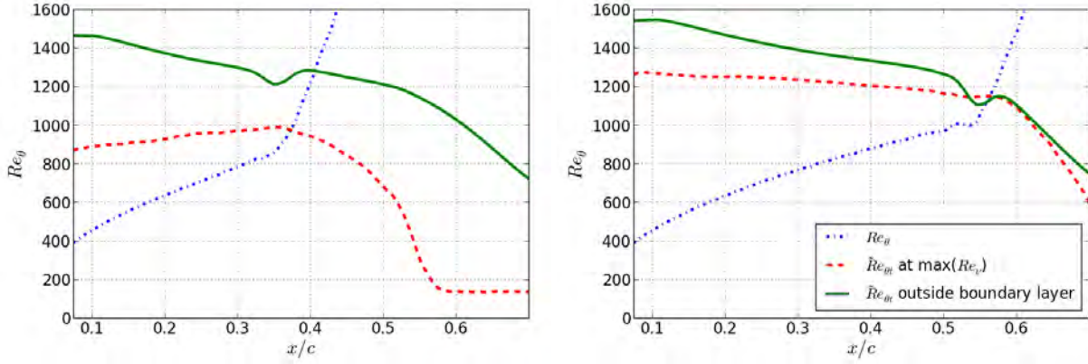
Figure 5.9. Re_\theta along with the critical value, Re_{\theta_c} both just outside the boundary layer and at the position where Re_v obtains its maximal value in the boundary layer without (left) and with (right) the Kato-Launder modification applied. NLF(1)-0414F airfoil, Re_c = 6.1 \times 10^6 , \alpha = 0^\circ , Tu = 0.05\% .
