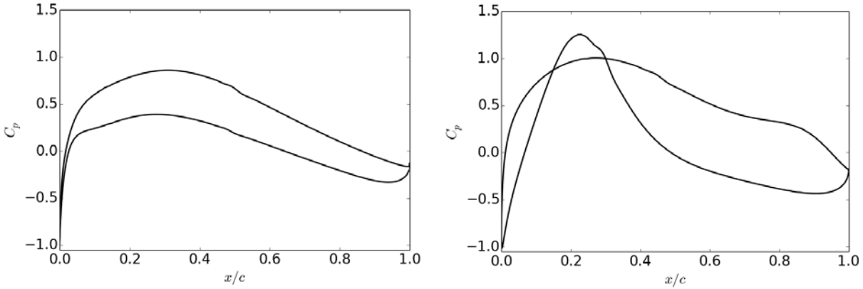
Figure 3.3. Pressure distributions of both NACA 63 3 -418 (left) and S814 (right), \alpha = 0^\circ and Re_c = 2.4 \times 10^6 for both.
