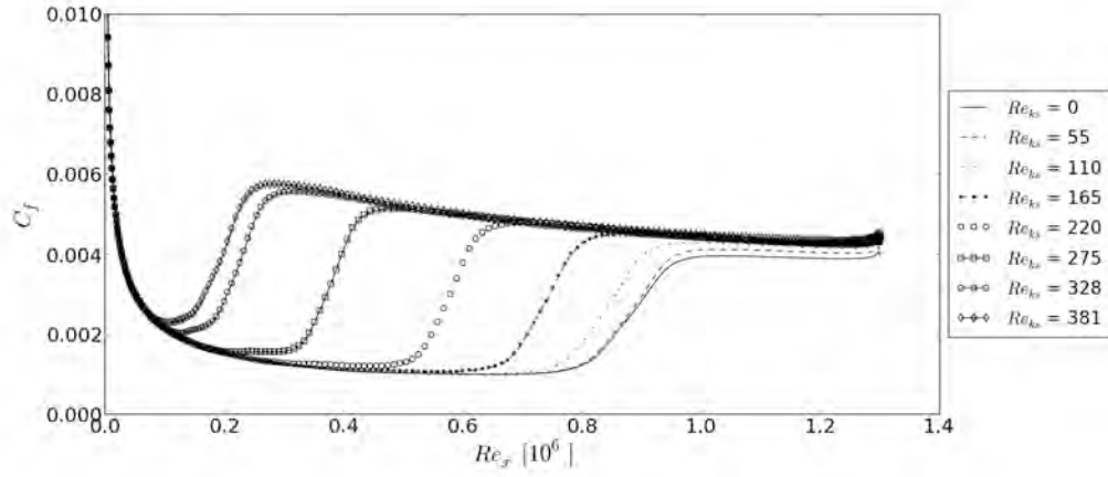
Figure 7.5. The effect on local skin friction coefficient ( C_f ) of varying Re_{ks} . Zero pressure gradient flat plate, freestream turbulence intensity = 0.91%.
