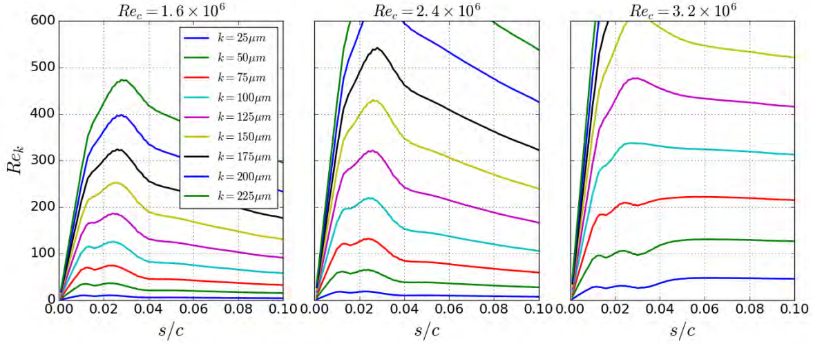
Figure 3.6. Projected Re_k values along upper surface of NACA 633-418, s/c measured from leading edge center, angle of attack fixed at 6 degrees. Boundary layer profiles taken from OVERFLOW RANS simulations.
