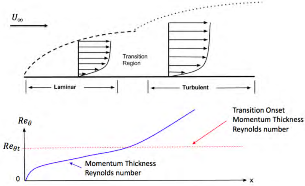
Figure 2.3. Sketch of developing boundary layer to demonstrate the approximate behavior of momentum thickness Reynolds number.
