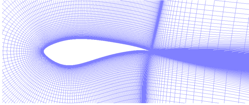
Figure 5.15. Grid used for S814 simulations, grid has 500 points along the airfoil surface with 350 points in the normal direction, every other grid line shown for clarity.
