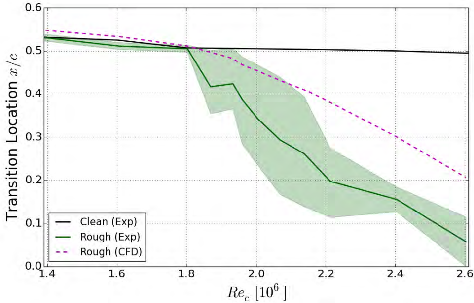
Figure 7.22. Comparison of upper surface transition location prediction, angle of attack fixed at 0 degrees, Re_c varied by increasing freestream velocity. NACA 633-418 airfoil, k/c = 172 \times 10^{-6} roughness applied from x/c = -0.13 : 0.02 , distribution density 15%, shaded region corresponds to 25% and 75% spanwise turbulent locations, k_s/c = 80 \times 10^{-6} input into roughness model.
