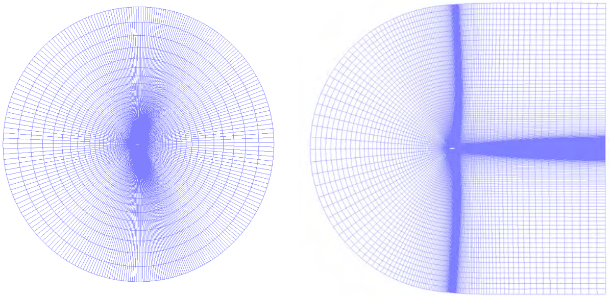
Figure 4.2. Far field view of both O-type (left) and C-type (right) grids for NACA 63 3 -418 airfoil.
