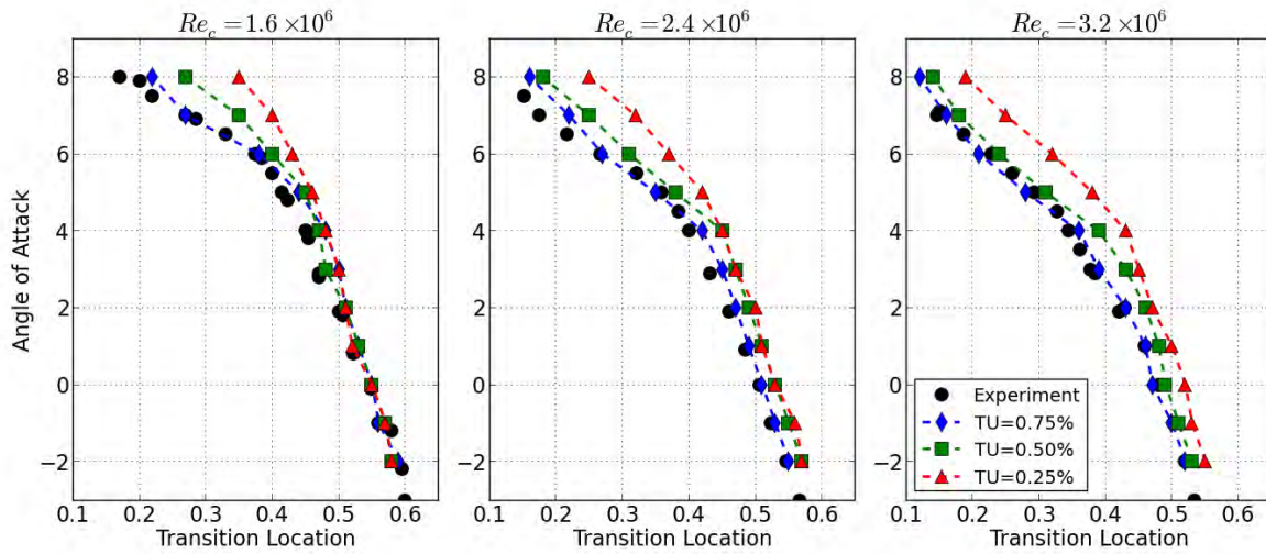
Figure 5.4. Comparison of upper surface transition location prediction with variation in input turbulence intensity ( Tu ) compared to experimental results of Ehrmann and White [1], NACA 63-418.
