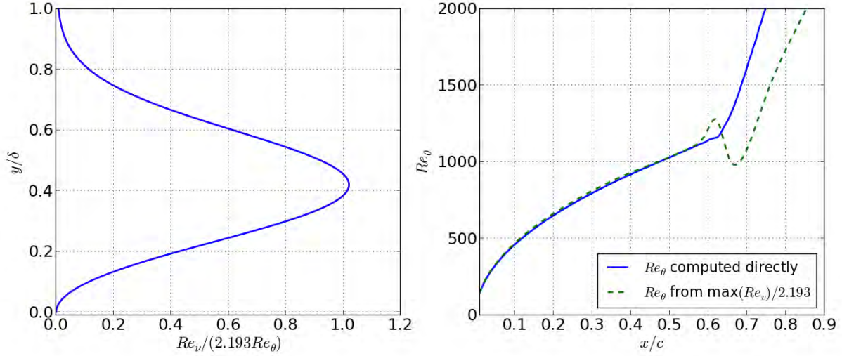
Figure 5.2. (left) Profile of vorticity Reynolds number normalized by 2.193Re_\theta , with Re_\theta computed directly, profile taken at x/c = 0.2 . (right) Plot of momentum thickness Reynolds number along flat plate computed both directly and using relationship with Re_v , Re_c = 5.0 \times 10^6 .
