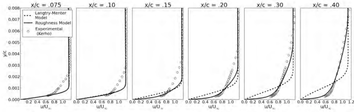
Figure 7.16. Boundary layer profiles: Kerho [54], unmodified Langtry-Menter transition model, computational roughness model. NACA 0012 airfoil, Re_c = 1.25 \times 10^6 , \alpha = 0^\circ , Tu = 0.1\% , distributed roughness applied x/c = 0.0314 - 0.0539
