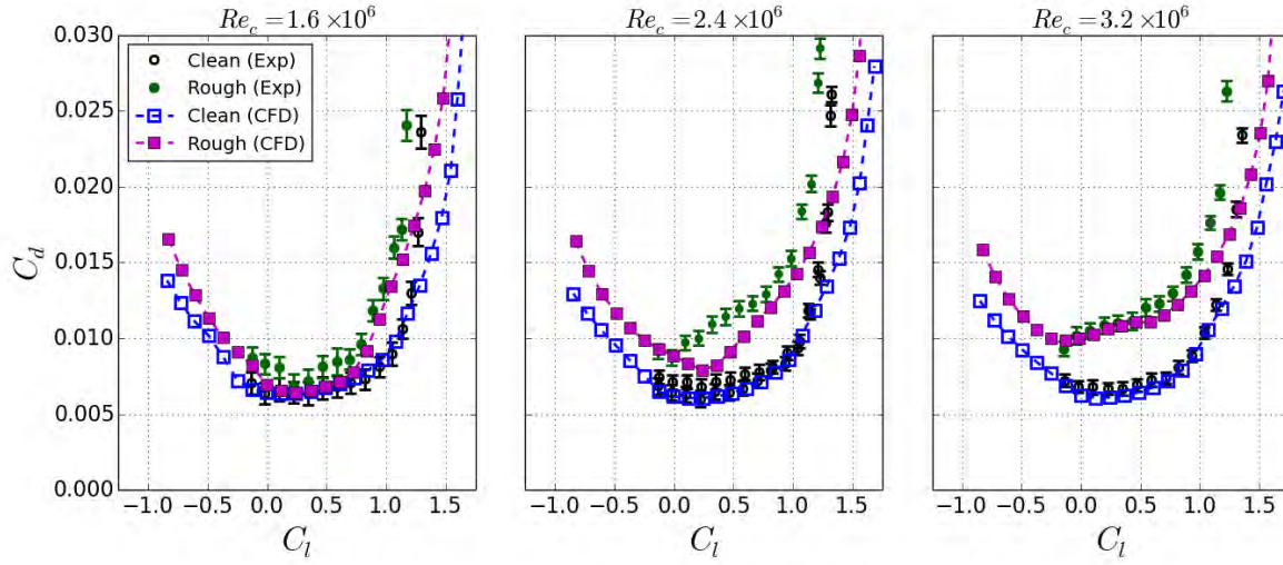
Figure 7.21. Predicted drag polars compared to experimental results, NACA 633-418 airfoil, k/c = 172 \times 10^{-6} roughness applied from x/c = -0.13 : 0.02 , distribution density 15%, k_s/c = 80 \times 10^{-6} input into roughness model.
