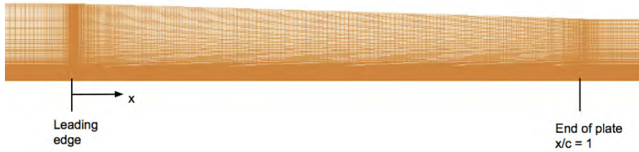
Figure 7.4. Sketch of grid used for favorable pressure gradient test cases, inflow and outflow sections continue 10 and 25 chord lengths respectively in either direction (not shown).
