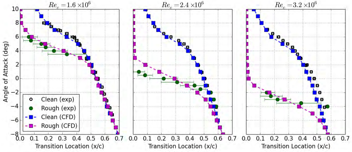
Figure 7.20. Comparison of upper surface transition location prediction with experimental results, NACA 633-418 airfoil, k/c = 172 \times 10^{-6} roughness applied from x/c = -0.13 : 0.02 , distribution density 15%, k_s/c = 80 \times 10^{-6} input into roughness model.
