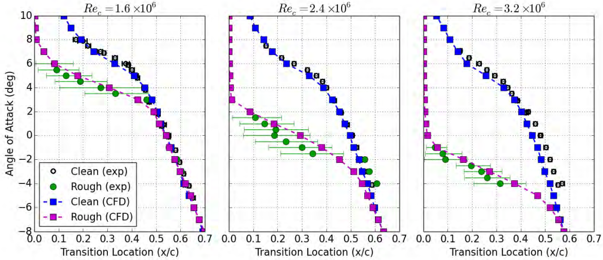
Figure 7.26. Comparison of upper surface transition location prediction with experimental results, NACA 633-418 airfoil, k/c = 172 \times 10^{-6} roughness applied from x/c = -0.13 : 0.02 , distribution density 9%, k_s/c = 75 \times 10^{-6} input into roughness model.
