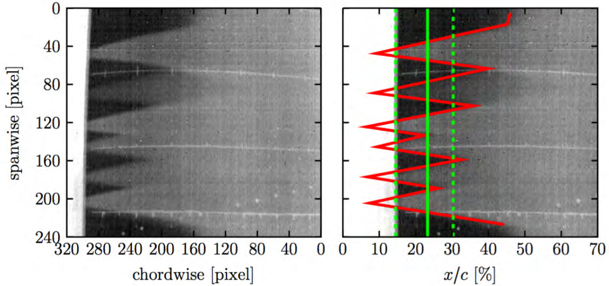
Figure 3.10. Raw (left) and processed (right) IR image demonstrating how the transition location was determined. The solid green line represents the position where 50% of the span is turbulent, while from left to right the dotted lines represent the 25% and 75% value.
