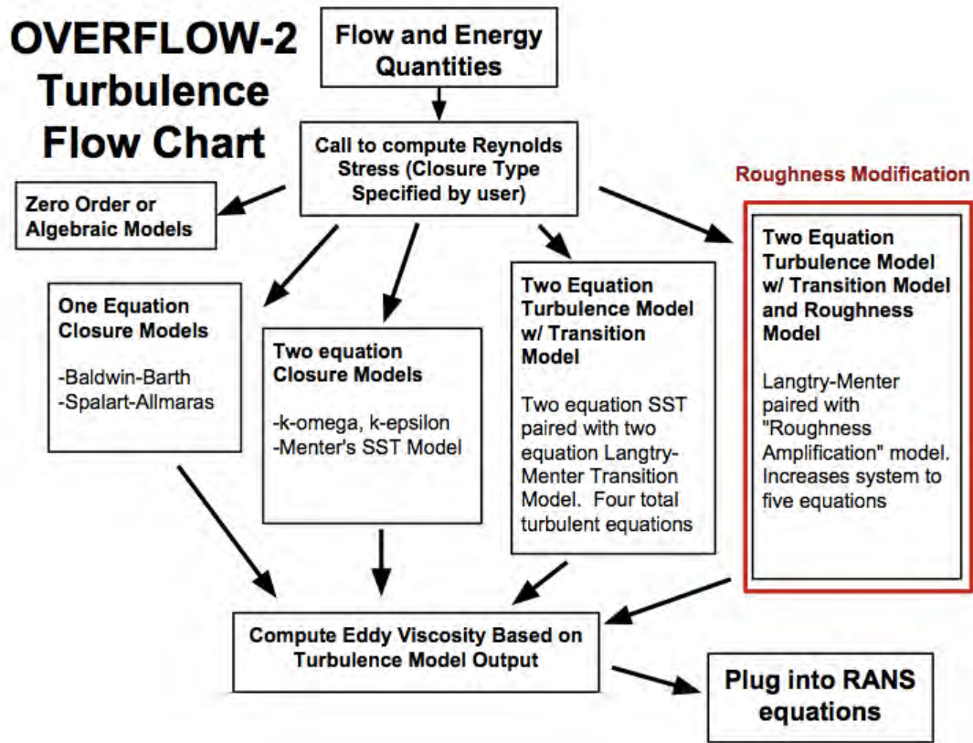
Figure 6.6. Graphical description of turbulence model implementation in OVERFLOW-2
