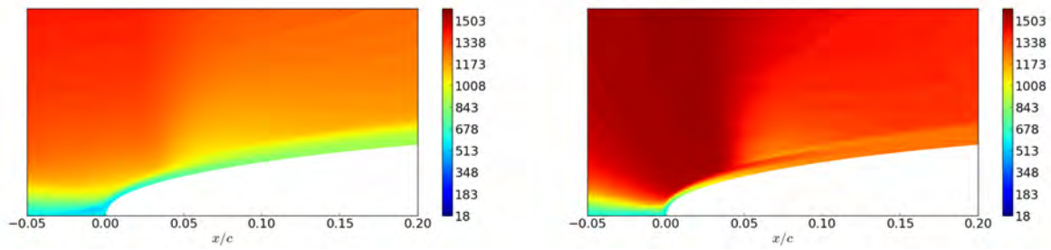
Figure 5.7. Enlargement near the leading edge of the \tilde{Re}_{\theta_t} variable both without (left) and with (right) the Kato-Launder limiter. NLF(1)-0414F airfoil, Re_c = 6.1 \times 10^6 , \alpha = 0^\circ , Tu = 0.05\% . The images have been enlarged 20 \times in the wall normal direction to show the boundary layer details, the airfoil profile is to scale.
