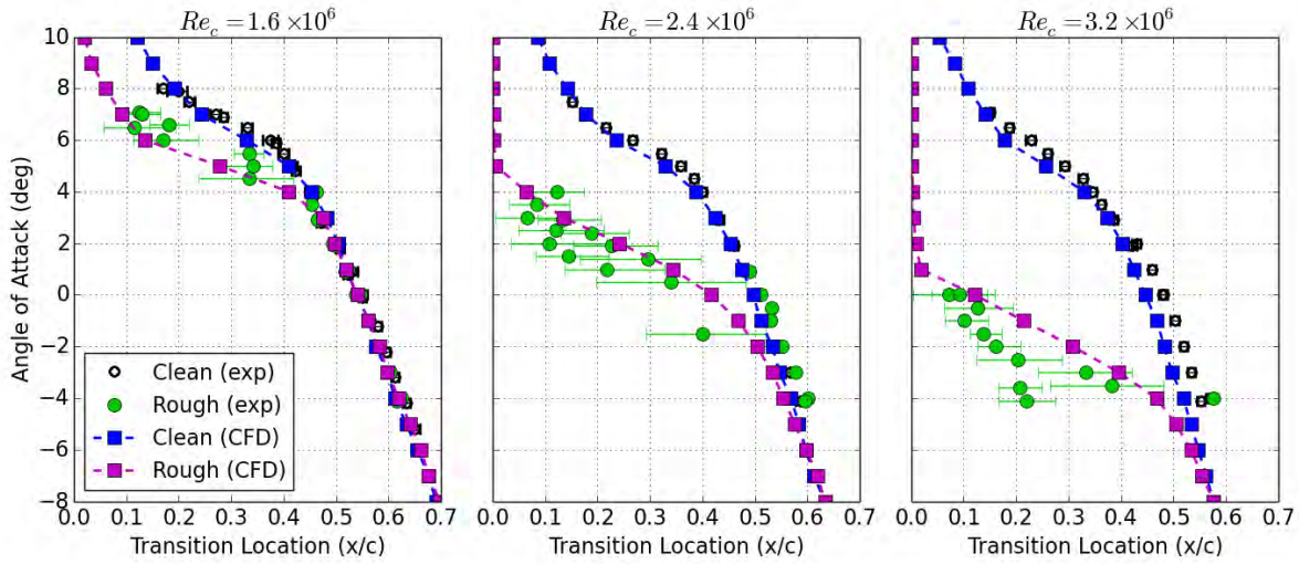
Figure 7.28. Comparison of upper surface transition location prediction with experimental results, NACA 633-418 airfoil, k/c = 172 \times 10^{-6} roughness applied from x/c = -0.13 : 0.02 , distribution density 3%, k_s/c = 70 \times 10^{-6} input into roughness model.
