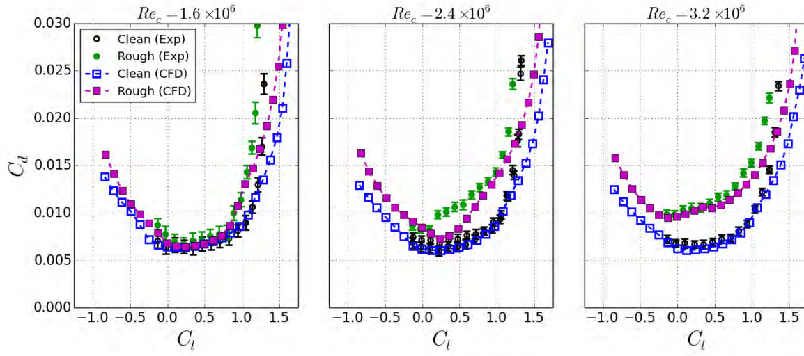
Figure 7.27. Predicted drag polars compared to experimental results, NACA 633-418 airfoil, k/c = 172 \times 10^{-6} roughness applied from x/c = -0.13 : 0.02 , distribution density 9%, k_s/c = 75 \times 10^{-6} input into roughness model.
