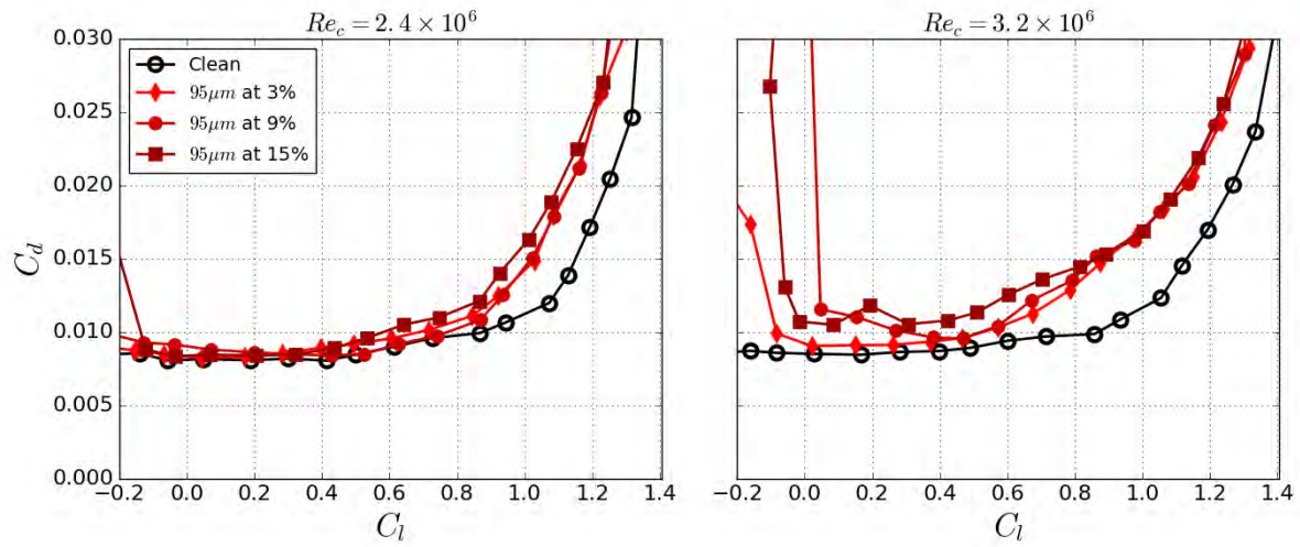
Figure 3.15. Effect of roughness distribution density on lift and drag, S814 airfoil, 3%, 9%, and 15% distribution densities, all at 95\mu\text{m} height and from tunnel entry 7.
