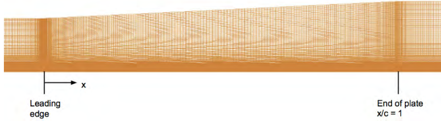
Figure 7.3. Sketch of grid used for adverse pressure gradient test cases, inflow and outflow sections continue 10 and 25 chord lengths respectively in either direction (not shown).
