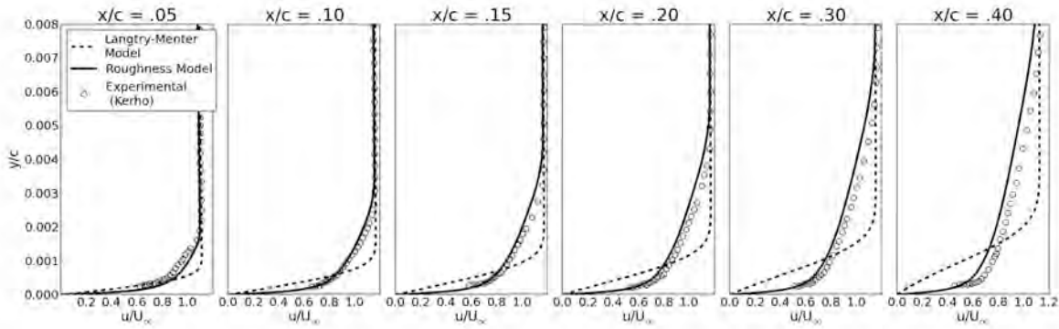
Figure 7.14. Boundary layer profiles: Kerho [54], unmodified Langtry-Menter transition model, computational roughness model. NACA 0012 airfoil, Re_c = 1.25 \times 10^6 , \alpha = 0^\circ , Tu = 0.1\% , distributed roughness applied x/c = 0.0018 - 0.0191
