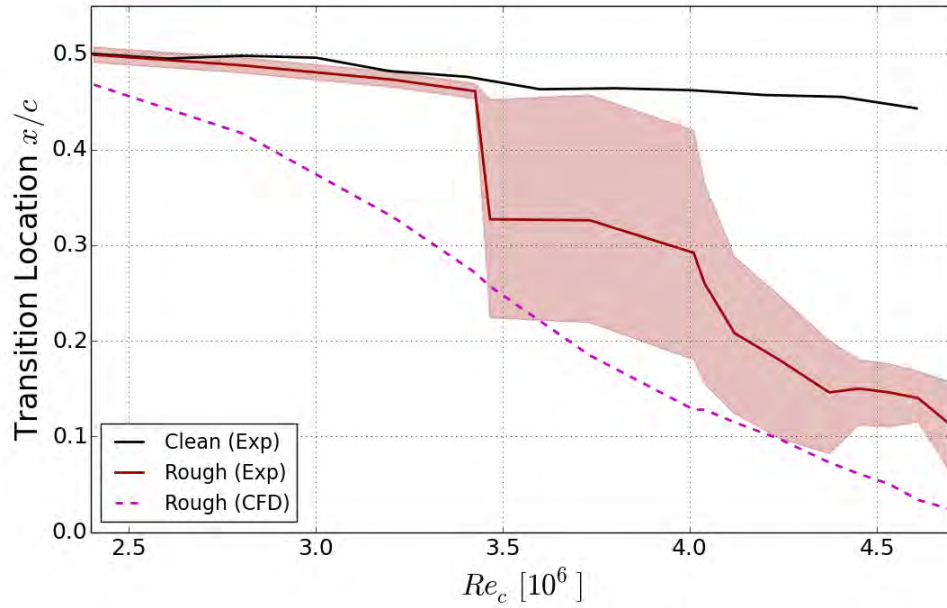
Figure 7.25. Comparison of upper surface transition location prediction with experimental results, NACA 63 3 -418 airfoil, k/c = 123 \times 10^{-6} roughness applied from x/c = -0.13 : 0.02 , distribution density 15%, k_s/c = 57 \times 10^{-6} input into roughness model.
