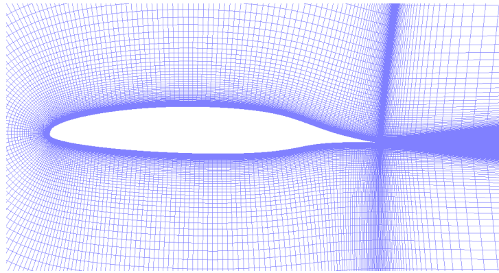
Figure 5.10. Grid used for NLF(1)-0414F simulations, grid has 500 points along the airfoil surface with 350 points in the normal direction, every other grid line shown for clarity.
