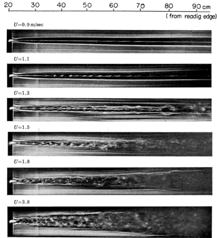
Figure 2.5. Varying freestream velocities and the flow feature generated behind the roughness element, adapted from Mochizuki [46]
