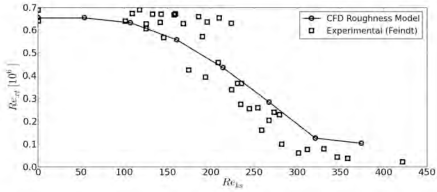
Figure 7.6. Roughness Reynolds number ( Re_{ks} ) plotted against location of transition onset ( Re_{xt} ) for zero pressure gradient flat plate.
