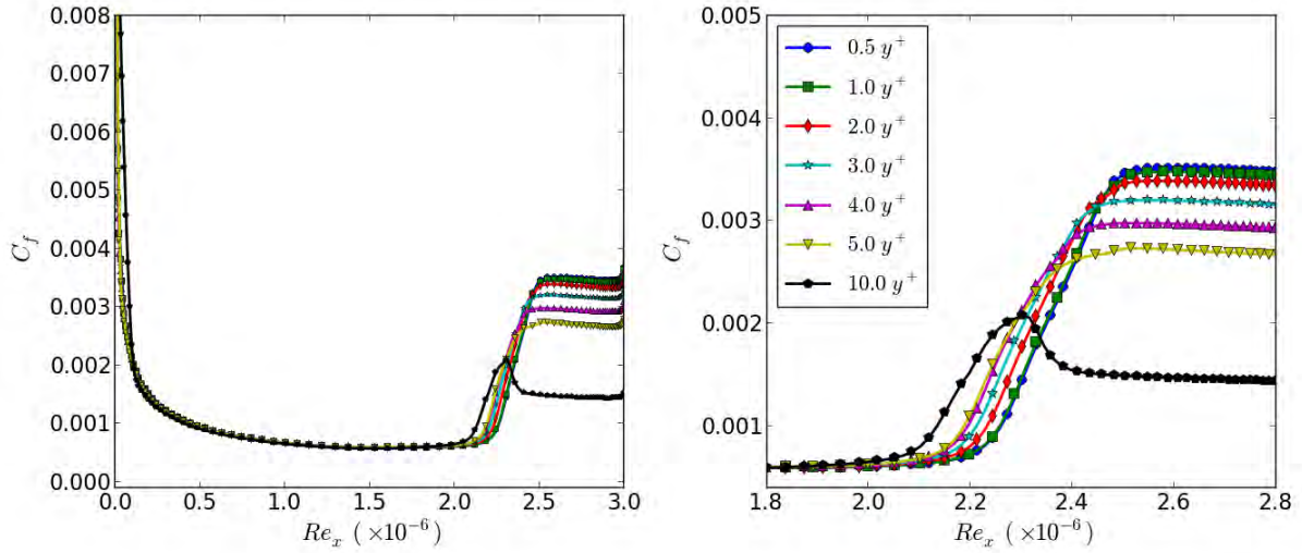
Figure 5.5. Skin friction along a flat plate, with a variation in initial wall spacing. Tu = 0.5\% .
