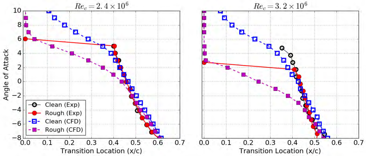
Figure 7.34. Comparison of upper surface transition location prediction with experimental results, S814 airfoil, k/c = 117 \times 10^{-6} roughness applied from x/c = -0.14 : 0.025 , distribution density 3%, k_s/c = 60 \times 10^{-6} input into roughness model.
