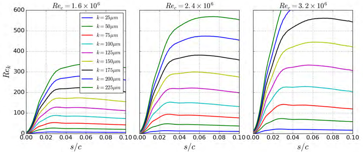
Figure 3.5. Projected Re_k values along upper surface of NACA 633-418, s/c measured from leading edge center, angle of attack fixed at 0 degrees. Boundary layer profiles taken from OVERFLOW RANS simulations.
