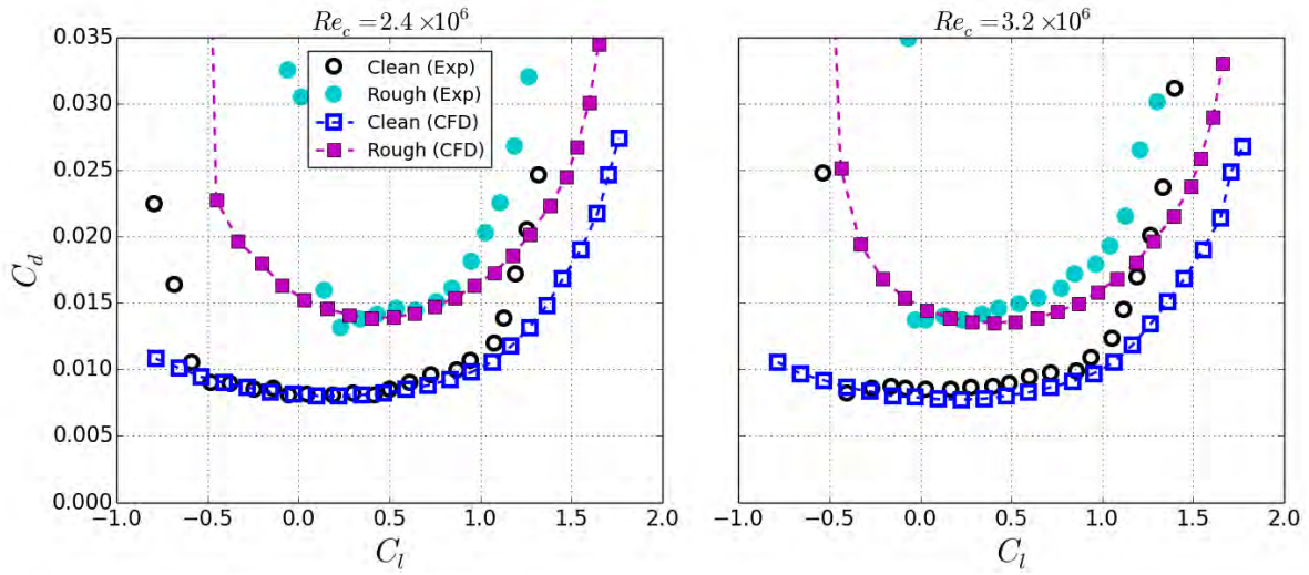
Figure 7.36. Predicted drag polars compared to experimental results, S814 airfoil, k/c = 276 \times 10^{-6} roughness applied from x/c = -0.14 : 0.025, distribution density 3%, k_s/c = 141 \times 10^{-6} input into roughness model.
