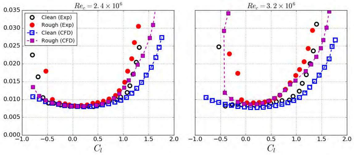
Figure 7.35. Predicted drag polars compared to experimental results, S814 airfoil, k/c = 117 \times 10^{-6} roughness applied from x/c = -0.14 : 0.025, distribution density 3%, k_s/c = 60 \times 10^{-6} input into roughness model.
