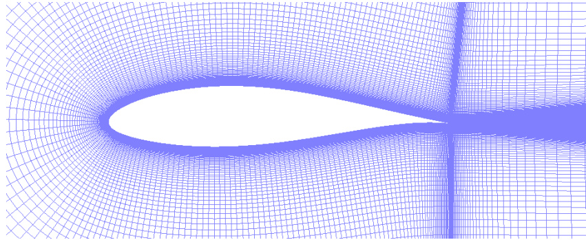
Figure 5.13. Grid used for NACA 63 3 -418 simulations, grid has 500 points along the airfoil surface with 350 points in the normal direction, every other grid line shown for clarity.
