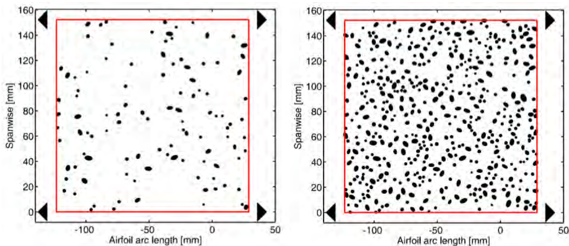
Figure 3.7. 3% and 15% density roughness distributions used for tunnel entries 1-4 on the NACA 63 3 -418, negative arc lengths correspond to placement on the lower airfoil surface.
