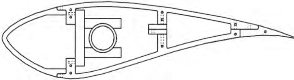
Figure 3.4. Cross sectional view of S814 airfoil model.
