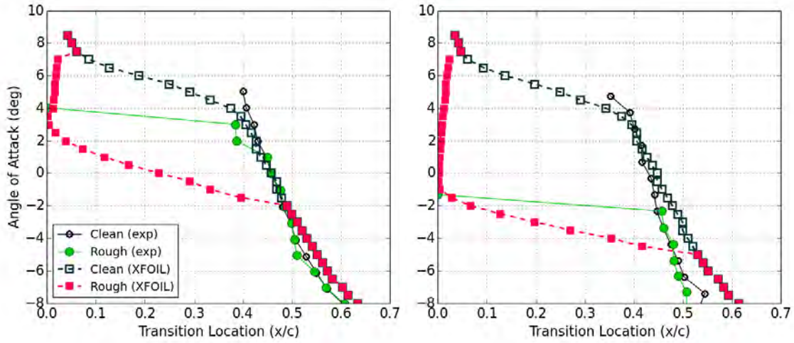
Figure A.5. Comparison of upper surface transition location prediction with experimental results, S814 airfoil, 172 \times 10^{-6} k/c roughness applied from x/c = -0.13 : 0.02 , distribution density 15%. N_{crit} = 6 used for free transition prediction in XFOIL, k_s/c = 80 \times 10^{-6} used in correlation calculations.
