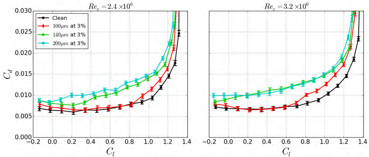
Figure 3.11. Effect of roughness height on lift and drag, NACA 63 3 -418, 100 \mu m, 140 \mu m, 200 \mu m heights, all at 3% distribution density and from tunnel entry 3.
