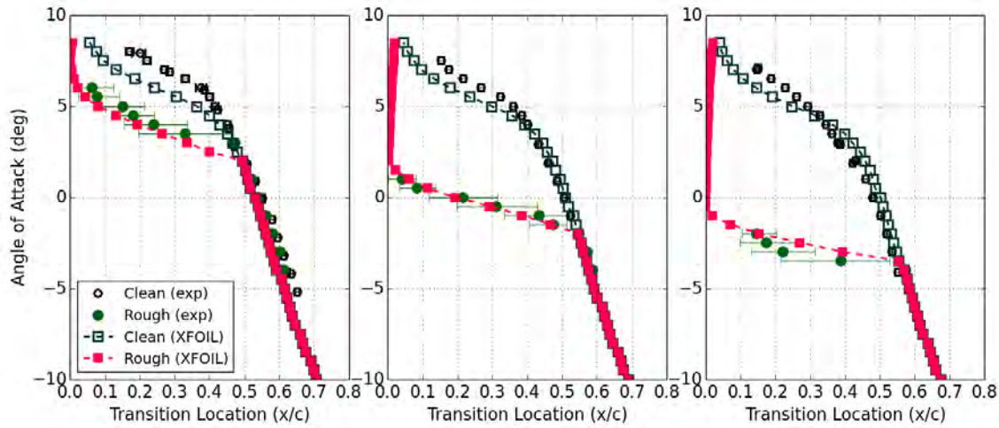
Figure A.2. Comparison of upper surface transition location prediction with experimental results, NACA 63 3 -418 airfoil, 172 \times 10^{-6} k/c roughness applied from x/c = -0.13 : 0.02 , distribution density 15%. N_{crit} = 6 used for free transition prediction in XFOIL, k_s/c = 80 \times 10^{-6} used in correlation calculations.
