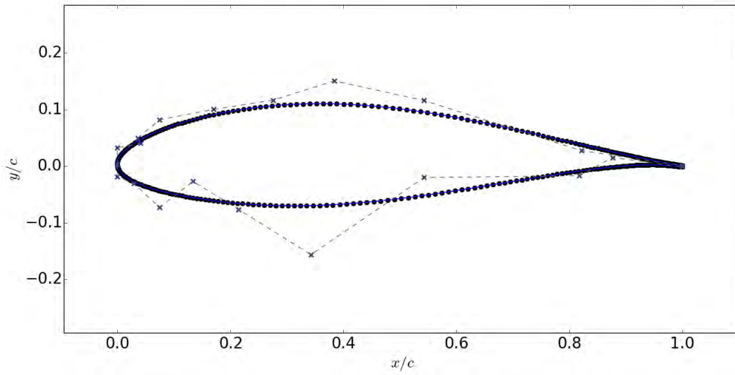
Figure B.1. Graphical representation of Bezier curves used for NACA 63 3 -418 airfoil, control points indicated by x's with the dashed line connecting them.
