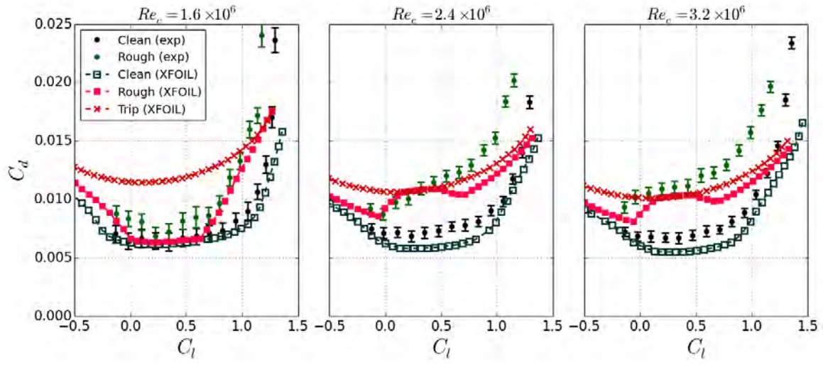
Figure A.4. Predicted drag polars compared to experimental results, NACA 633-418 airfoil, k/c = 172 \times 10^{-6} roughness applied from x/c = -0.13 : 0.02 , distribution density 15%. N_{crit} = 6 used for free transition prediction in XFOIL, k_s/c = 80 \times 10^{-6} used in correlation calculations.
