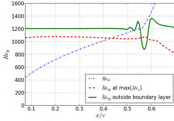
Figure 5.8. Re_\theta along with the critical value, Re_{\theta_c} both just outside the boundary layer and at the position where Re_v obtains its maximal value in the boundary layer, the solution is identical whether or not the Kato-Launder modification is applied. Flat-plate geometry, Re_c = 6.1 \times 10^6 , \alpha = 0^\circ , Tu = 0.05\% .
