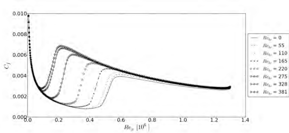
Figure 7.7. The effect on local skin friction coefficient ( C_f ) of varying Re_{k_s} . Flat plate, adverse pressure gradient, freestream turbulence intensity = 0.91%.
