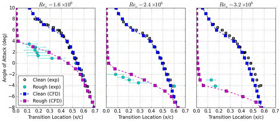
Figure 7.30. Comparison of upper surface transition location prediction with experimental results, NACA 633-418 airfoil, k/c = 246 \times 10^{-6} roughness applied from x/c = -0.13 : 0.02 , distribution density 3%, k_s/c = 101 \times 10^{-6} input into roughness model.
