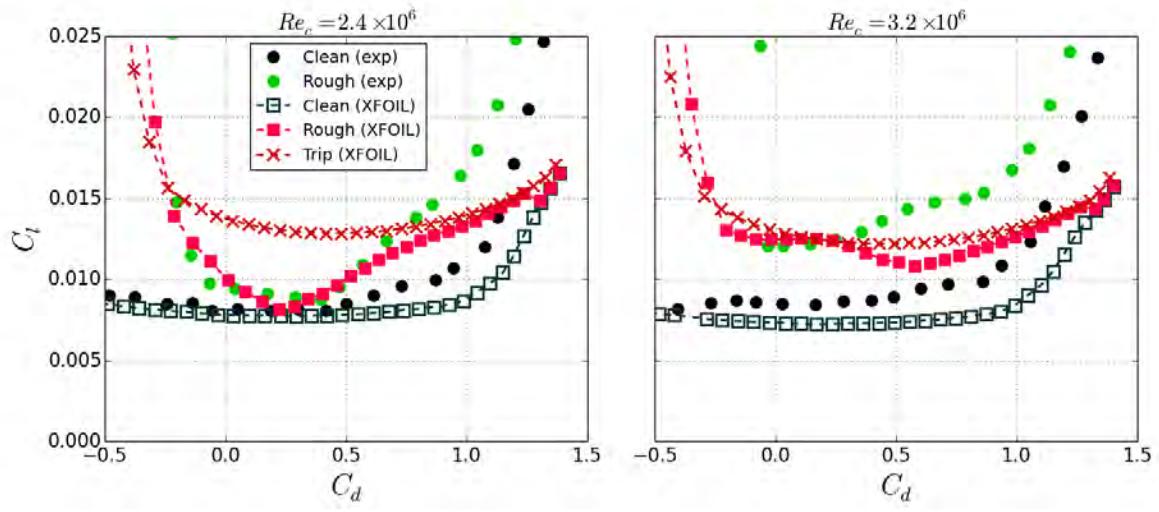
Figure A.6. Predicted drag polars compared to experimental results, S814 airfoil, 172 \times 10^{-6} k/c roughness applied from x/c = -0.13 : 0.02 , distribution density 15%. N_{crit} = 6 used for free transition prediction in XFOIL, k_s/c = 80 \times 10^{-6} used in correlation calculations.
