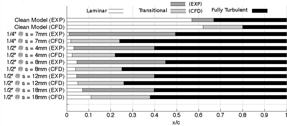
Figure 7.19. Comparison of boundary layer states for simulations run at Re_c = 1.25 \times 10^6 , details of test configurations can be found in Table 7.1
