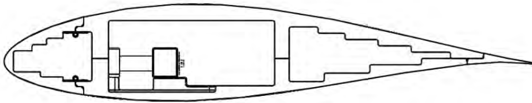
Figure 3.2. Cross sectional view of NACA 63 3 -418 airfoil model.
