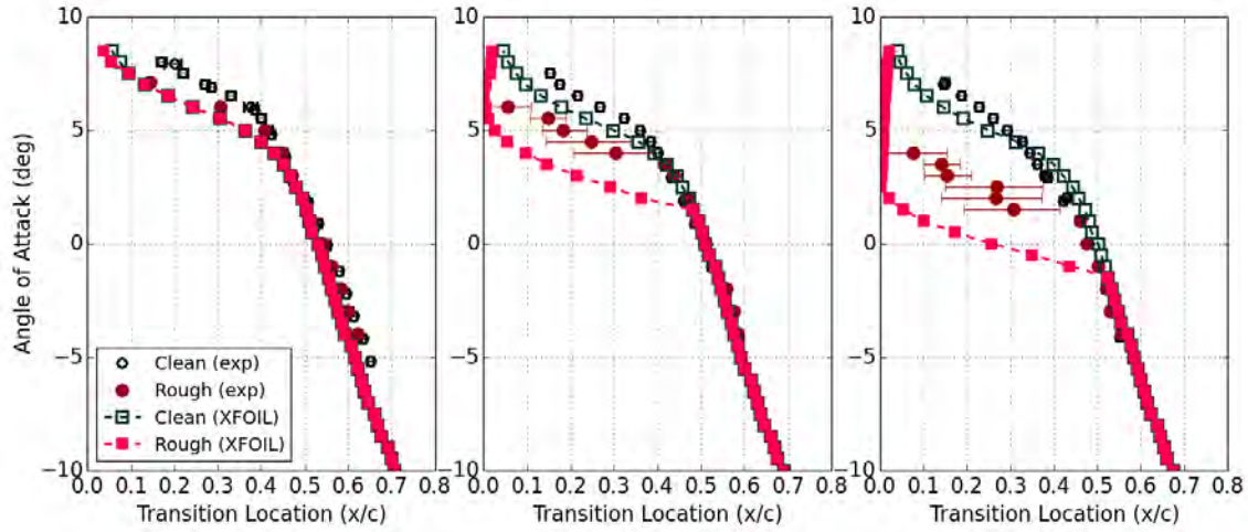
Figure A.3. Comparison of upper surface transition location prediction with experimental results, NACA 633-418 airfoil, 123 \times 10^{-6} k/c roughness applied from x/c = -0.13 : 0.02 , distribution density 15%. N_{crit} = 6 used for free transition prediction in XFOIL, k_s/c = 57 \times 10^{-6} used in correlation calculations.
