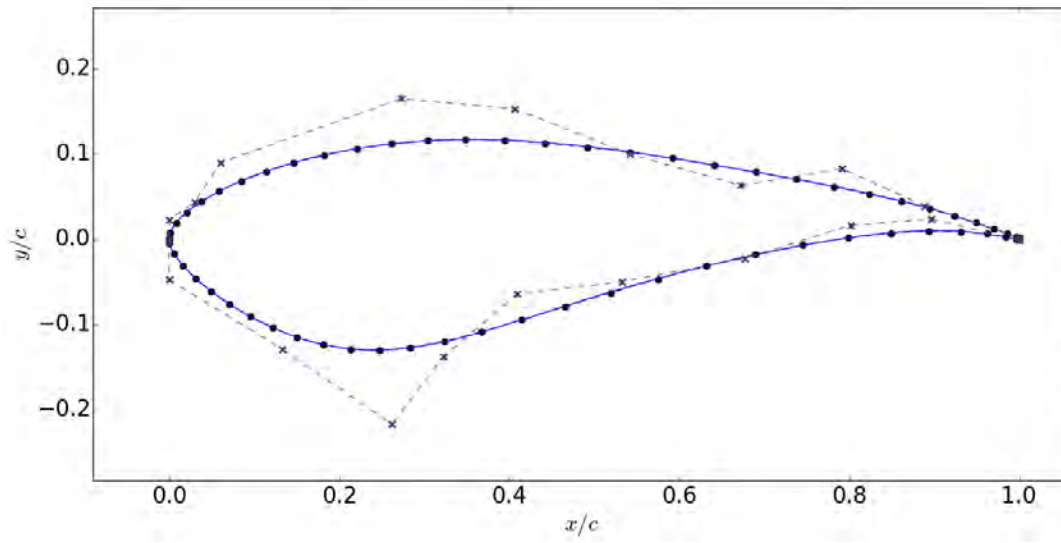
Figure B.2. Graphical representation of Bezier curves used for S814 airfoil, control points indicated by x's with the dashed line connecting them.
