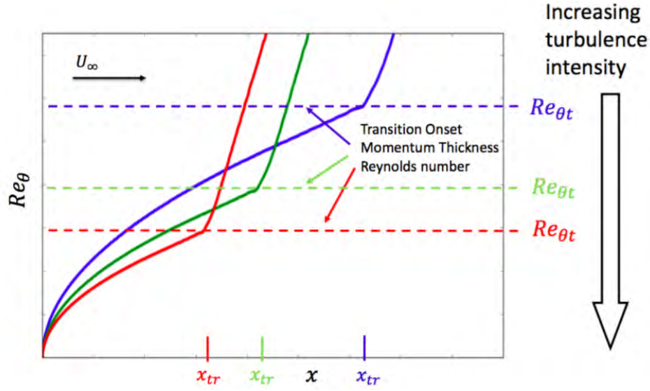
Figure 5.1. Sketch of impact of freestream turbulence intensity on the transition onset momentum thickness Reynolds number.
