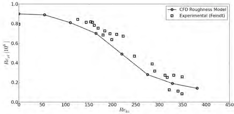
Figure 7.10. Roughness Reynolds number ( Re_{ks} ) plotted against location of transition onset ( Re_{xt} ) for flat plate, favorable pressure gradient.
