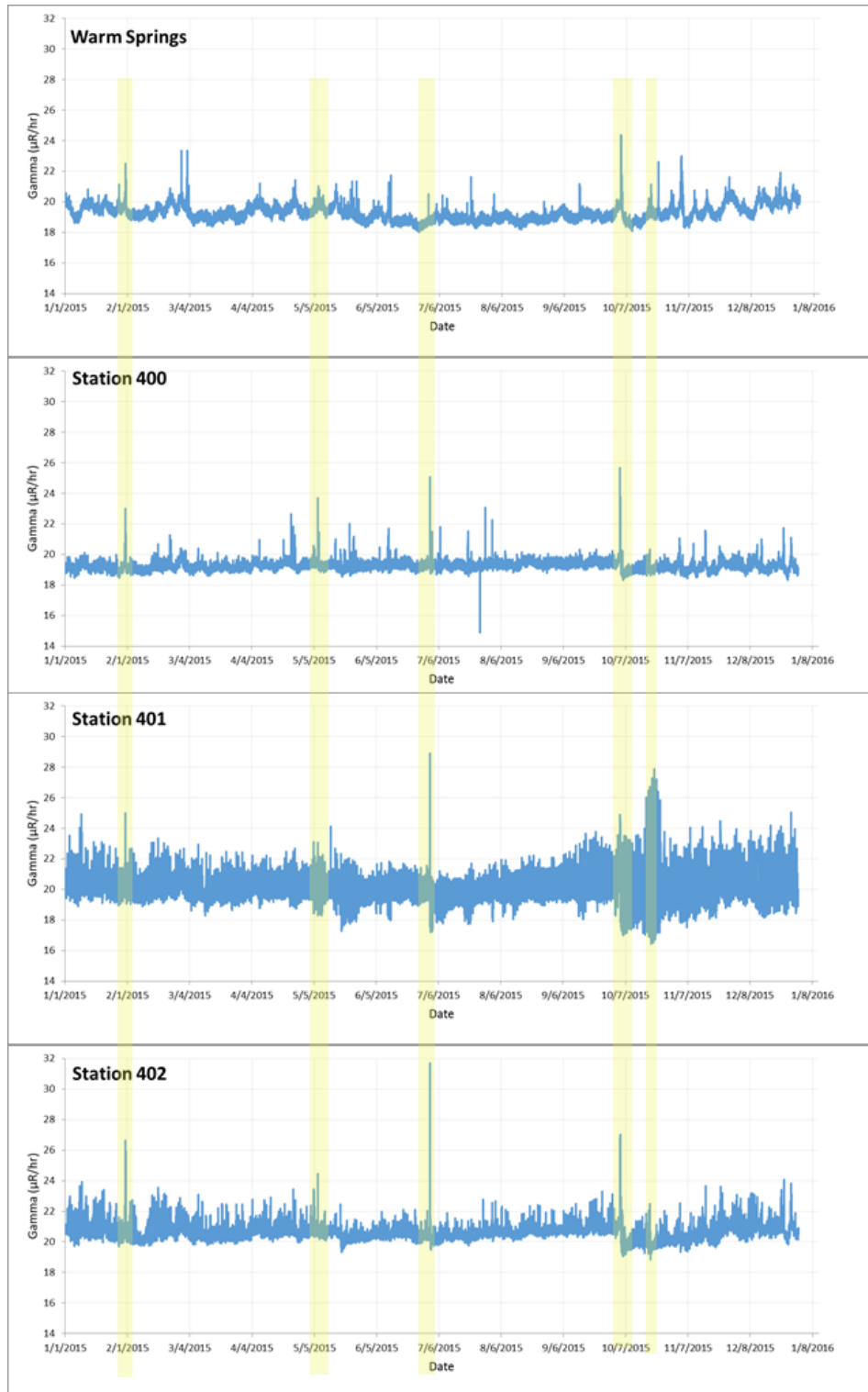
Figure 28. The CY2015 PIC gamma data for the CEMP station at Warm Springs Summit and the TTR stations that highlight select coincident times of increased values.
