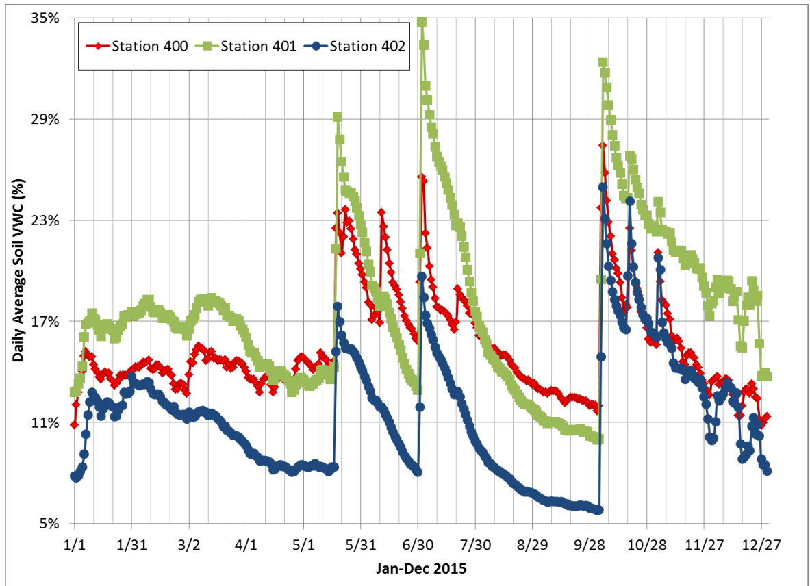
Figure 18. Soil volumetric water content for Stations 400, 401, and 402 for CY2015.
