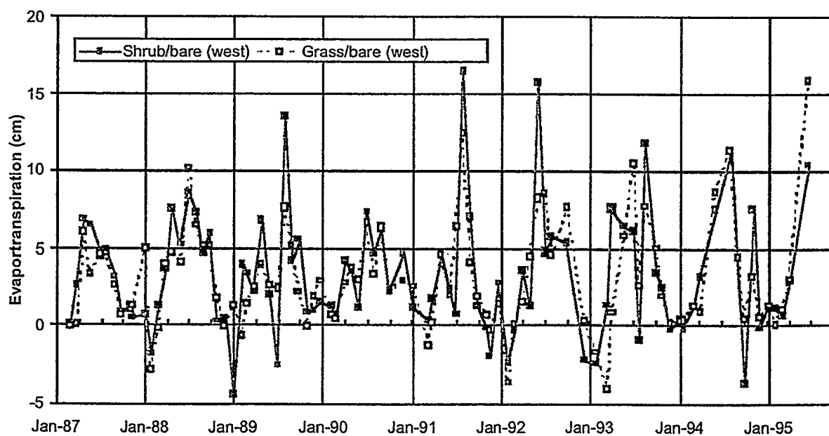
Figure 7. Monthly evapotranspiration for MDA B west plots with shrub/bare and grass/bare covers.
