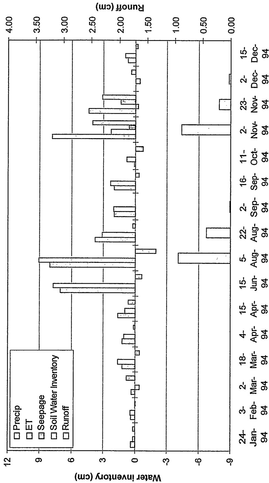
Figure 38. Water balance data collected for plot 4.
