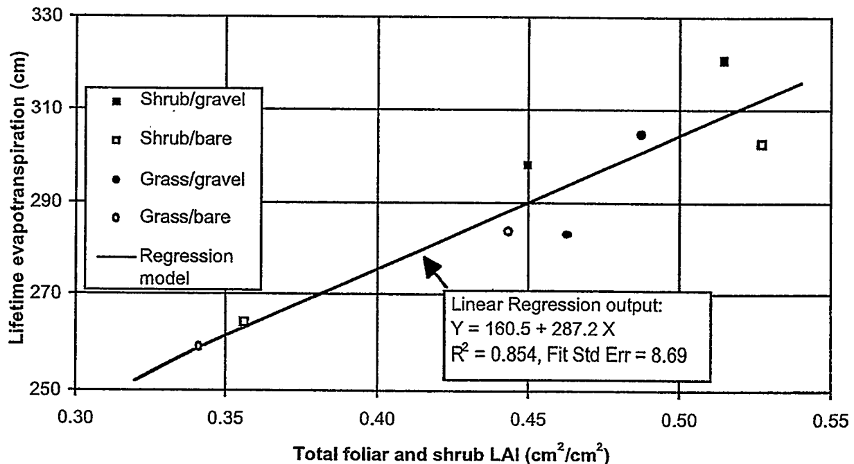
Figure 11. Total foliar and shrub leaf area index versus lifetime evapotranspiration for each of the four surface treatments at MDA B.
