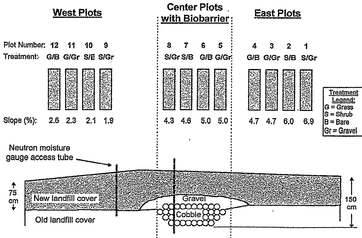
Figure 2a. Plot locations, surface treatments, and average percent downhill slope for study plots at MDA-B (top), and a cross section of soil profile characteristics (bottom). For further details refer to plot map in Appendix A.
