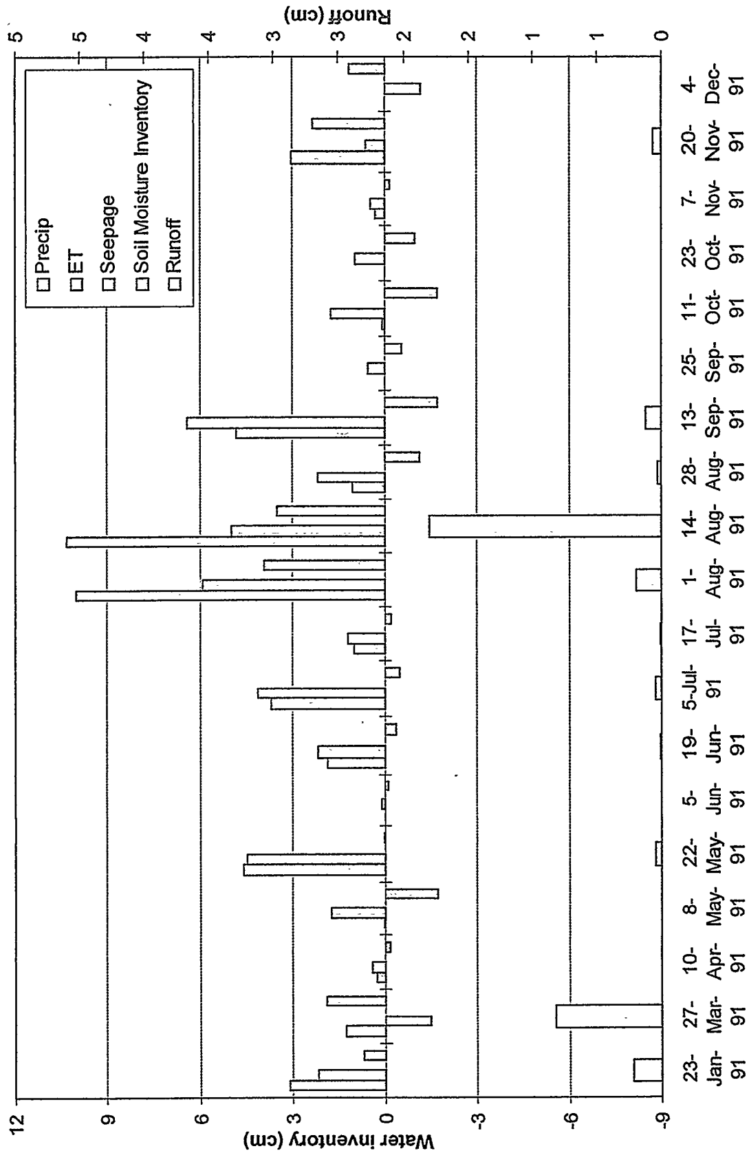
Figure 85. Water balance data collected for plot 9.
