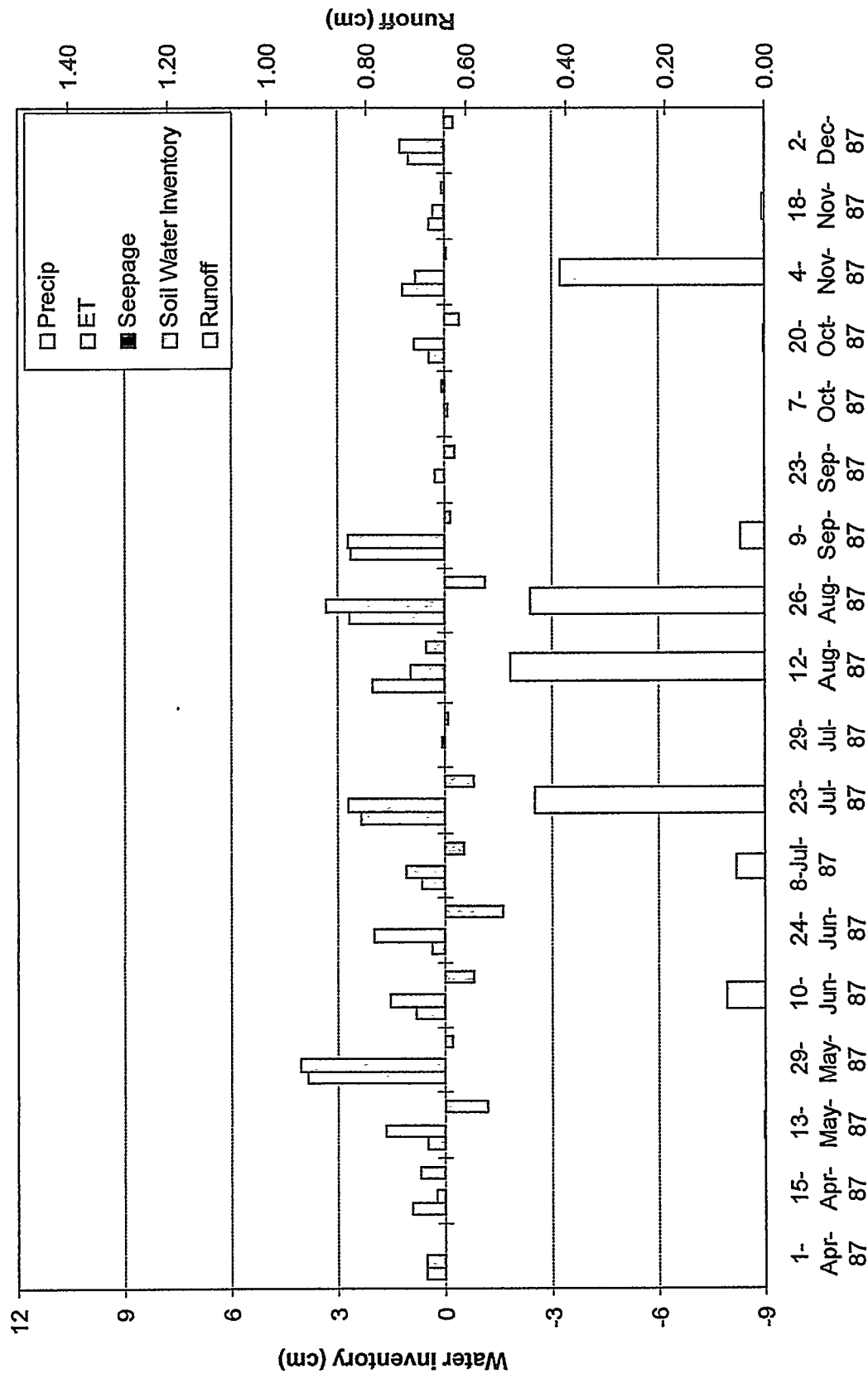
Figure 31. Water balance data collected for plot 4.
