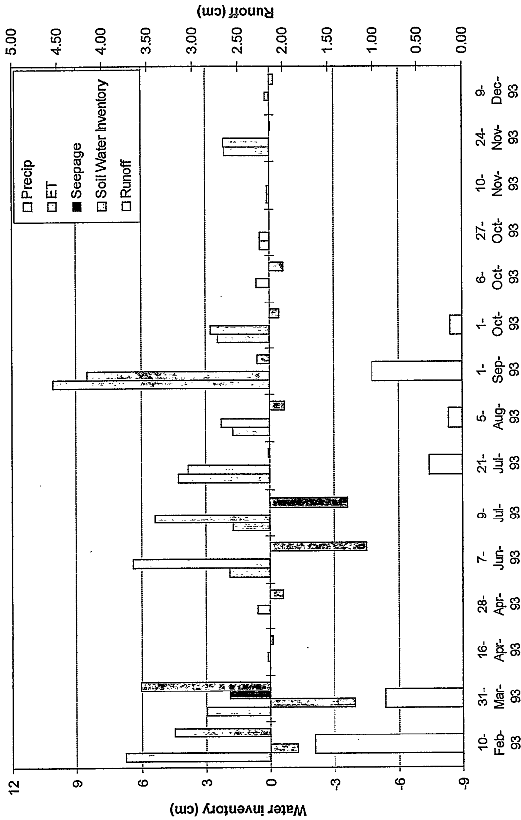
Figure 17. Water balance data collected for Plot 2.
