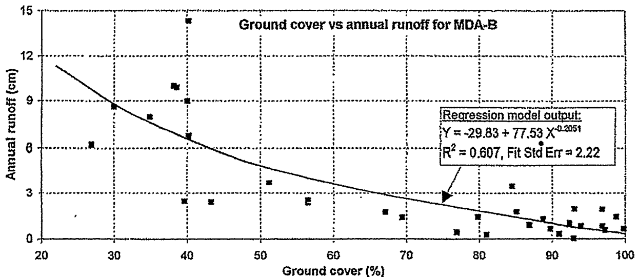
Figure 16. Ground cover and annual runoff for the MDA B plots for 1989, 1990, and 1994.
