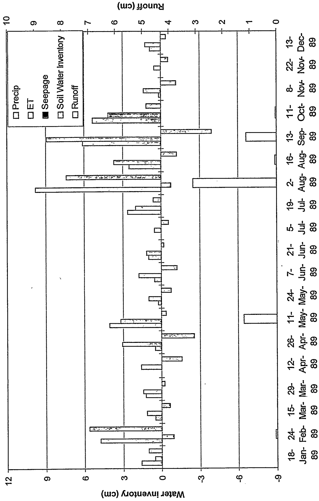
Figure 3. Water balance data collected for Plot 1.
