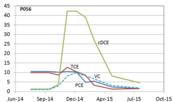
Figure 3. cVOC Concentrations in Treatment-Zone Monitoring Well P056 (in \mu\text{g/L} concentration)
