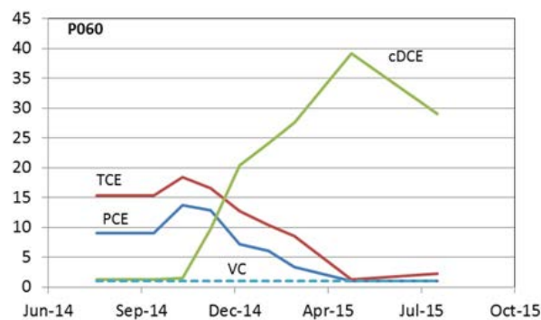
Figure 4. cVOC Concentrations in Treatment-Zone Monitoring Well P060 (in \mu\text{g/L} concentration)
