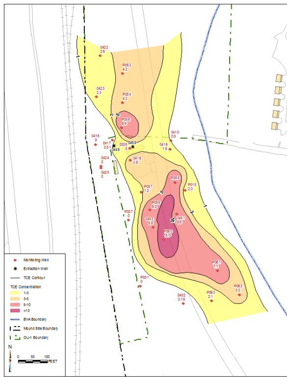
Figure 1. OU-1 TCE Plume Distribution in August 2014 (in \mu\text{g/L} concentration)
