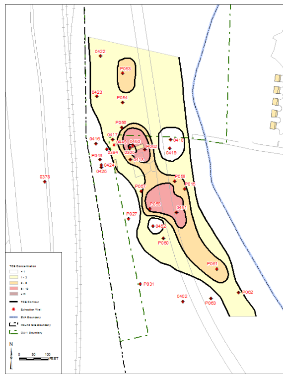
Figure 2. OU-1 TCE Plume Distribution in August 2015 (in \mu\text{g/L} concentration)
