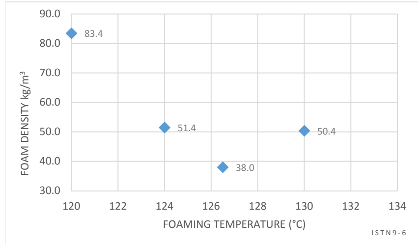
Figure 5. PS/SEBS/clay/Al foamed in the pressure vessel. Carbon dioxide pressure of 2000 psi (138 bar). Release rate of 50 bar/sec.
