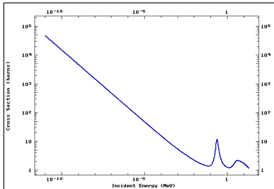
Figure 14 – Total neutron cross-section for ^6\text{Li} [3]
