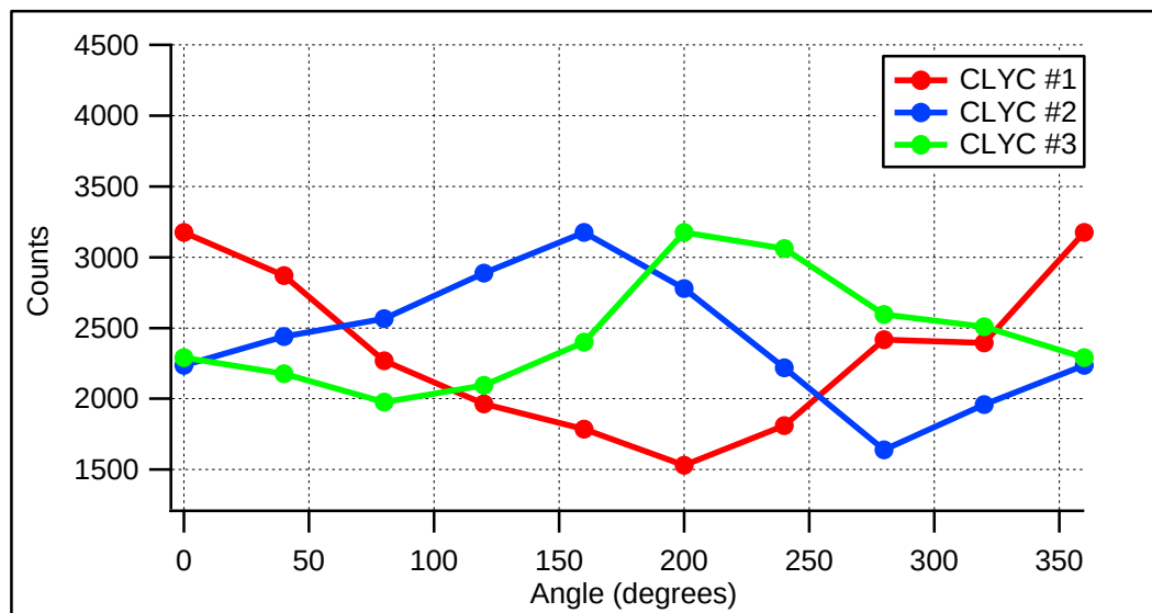
Figure 50 – ^{137}\text{Cs} gamma-ray directional measurements results, R=20 cm, z=10 cm
