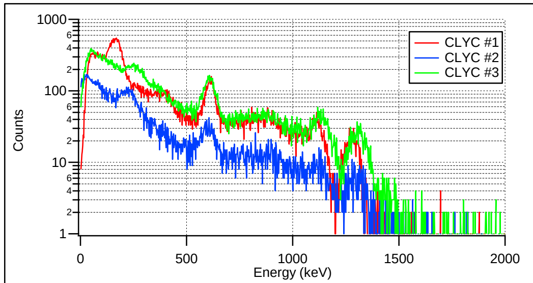
Figure 56 – Gamma-ray spectra for two source directional measurements, co-located sources
