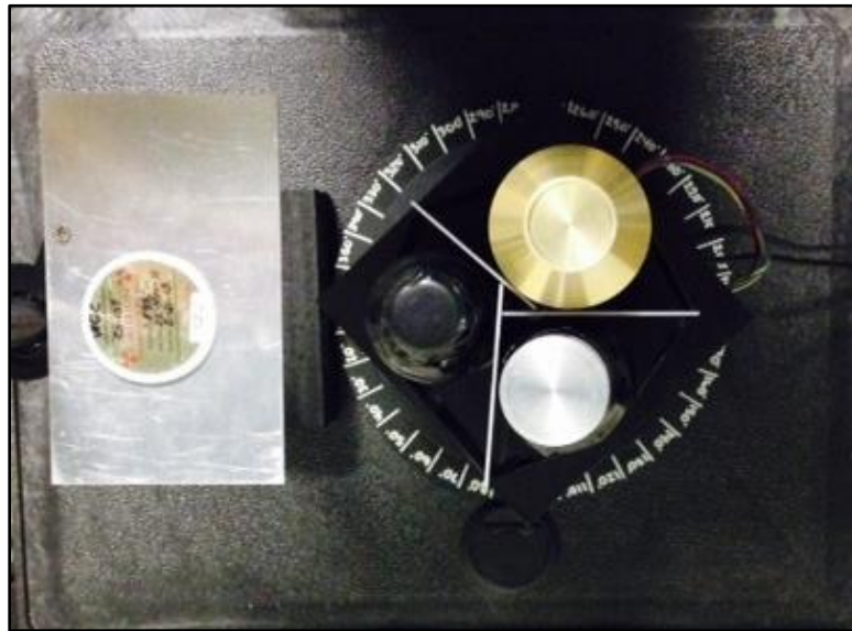
Figure 44 – ^{137}\text{Cs} gamma-ray directional measurements experimental setup, top view
