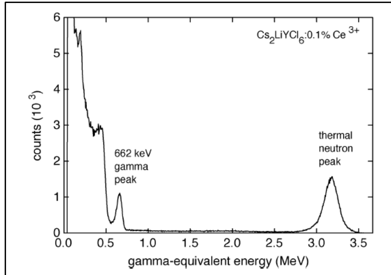
Figure 7 – Scintillation pulse-height spectrum of CLYC exposed to gamma rays of ^{137}\text{Cs} and thermal neutrons [17]
