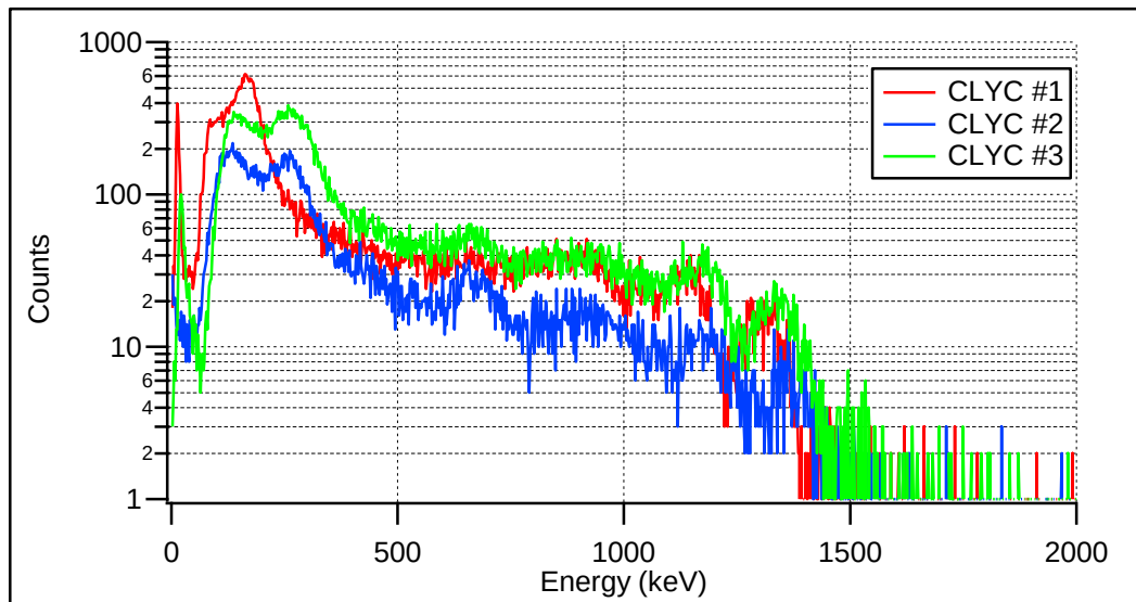
Figure 52 – Gamma-ray spectrum for two source directional measurements
