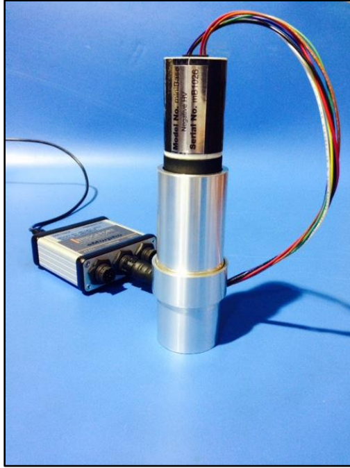
Figure 21 – Completed 1-inch CLYC detector assembly
