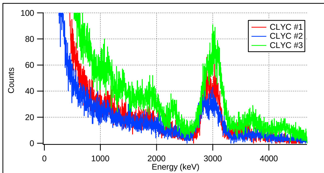
Figure 58 – Spectra for thermal neutron source directional measurements
