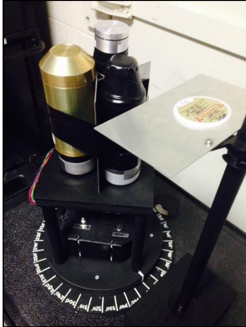
Figure 45 – ^{137}\text{Cs} gamma-ray directional measurements experimental setup, angled view
