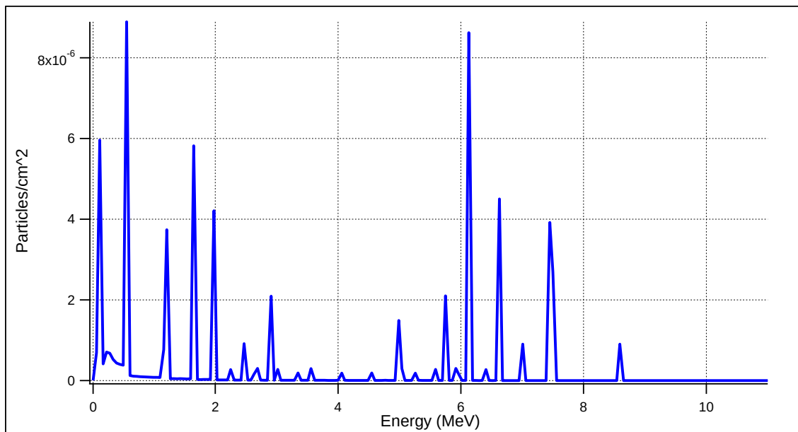
Figure 33 – Thermal neutron induced gamma rays in the 1"×1" NaCl scintillator
