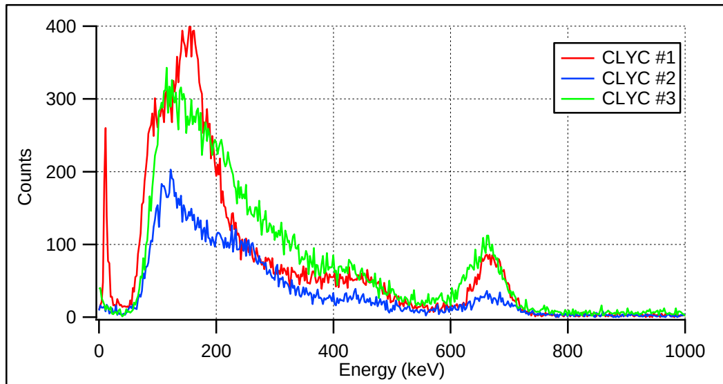
Figure 46 – Gamma-ray spectra at 0° for CLYC #1, #2 and #3
