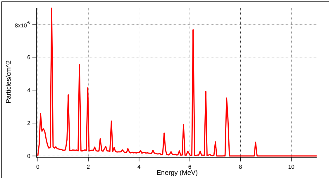
Figure 32 – Thermal neutron induced gamma rays in the 1"×1" CLYC
