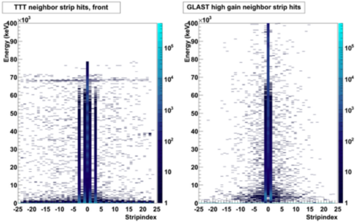
Figure 2. Cross talk effects in TTT2 (left) and GLAST (right) from A/Z = 2 cocktail beam at 400 MeV/u. Strip index 0 indicates highest energy observed in an event with closest 25 strips on either side of such event displayed.
