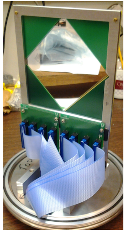
Figure 7: Left panel: A photo of the Micron Semiconductor Ltd. TTT2 type Si strip detector with the new PCB packaging funded by this award. Right panel: The detector on a mounting frame, attached to a standard vacuum flange. This configuration allows easy handling of detectors and minimizes the required cabling length. The box housing HINP motherboard and chips can be attached directly on the opposite side of the flange.
