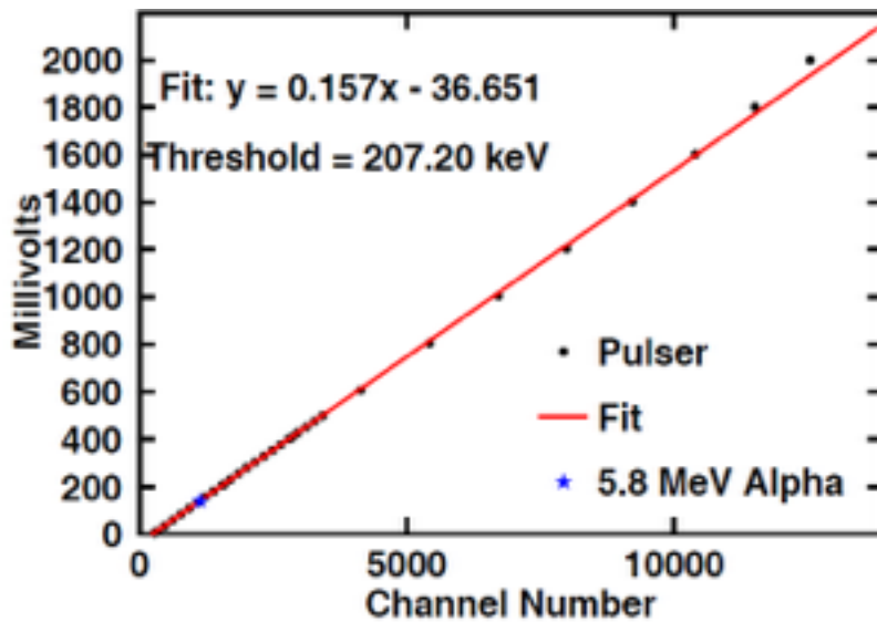
Figure 6: Pulser and \alpha linearity test of the high-gain channel of the dual-range chip. Not all channels are this linear. The linear fit is on the dense data at low pulse height.
