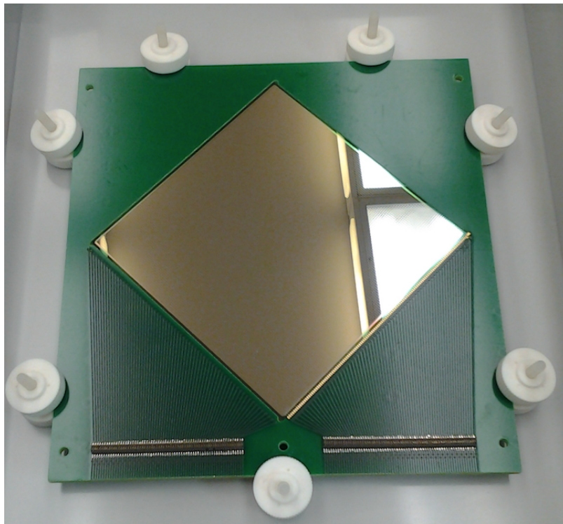
Figure 7: Left panel: A photo of the Micron Semiconductor Ltd. TTT2 type Si strip detector with the new PCB packaging funded by this award. Right panel: The detector on a mounting frame, attached to a standard vacuum flange. This configuration allows easy handling of detectors and minimizes the required cabling length. The box housing HINP motherboard and chips can be attached directly on the opposite side of the flange.
