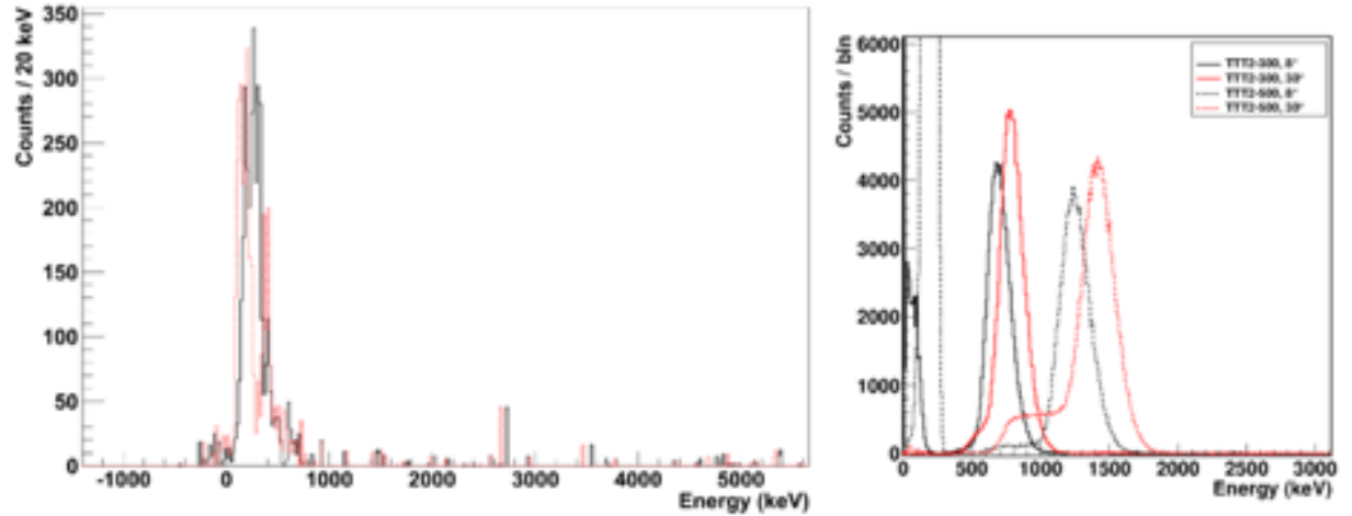
Figure 3. On the left, TTT2 response to 150 MeV/u protons at HIMAC in 2012 (front strips in black and back in red). On the right, response to 50 MeV/u protons at TAMU with different detector thicknesses and angles.
