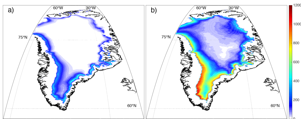
Figure 7. Regional Atmospheric Climate Model (RACMO2.3/GR) annual melt rates ( \text{kg m}^{-2} ) shown for areas of the GrIS with predicted positive surface mass balance (i.e. above the equilibrium line). Annual melt rates shown for (a) the 1958–1999 average and (b) for 2012.
