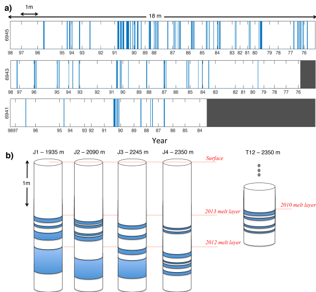
Figure 3. (a) Ice layers and ice lenses present in the visible stratigraphy of PARCA firm cores 6941, 6943, and 6945 drilled in 1998 are plotted with depth in core (m). The deepest core is 18 m long and the dates are assigned at depth (m) of each year's winter minima in dust concentration. (b) Schematic showing ice layer structure as measured in snow pits excavated between 2011 and 2014. The melt layer dashed lines indicate the position where the top of the ice layer was found in the field at J1 for the J-sites and at T12. J-sites are represented as found in April 2012. T12 representation is shown as found in 2011.
