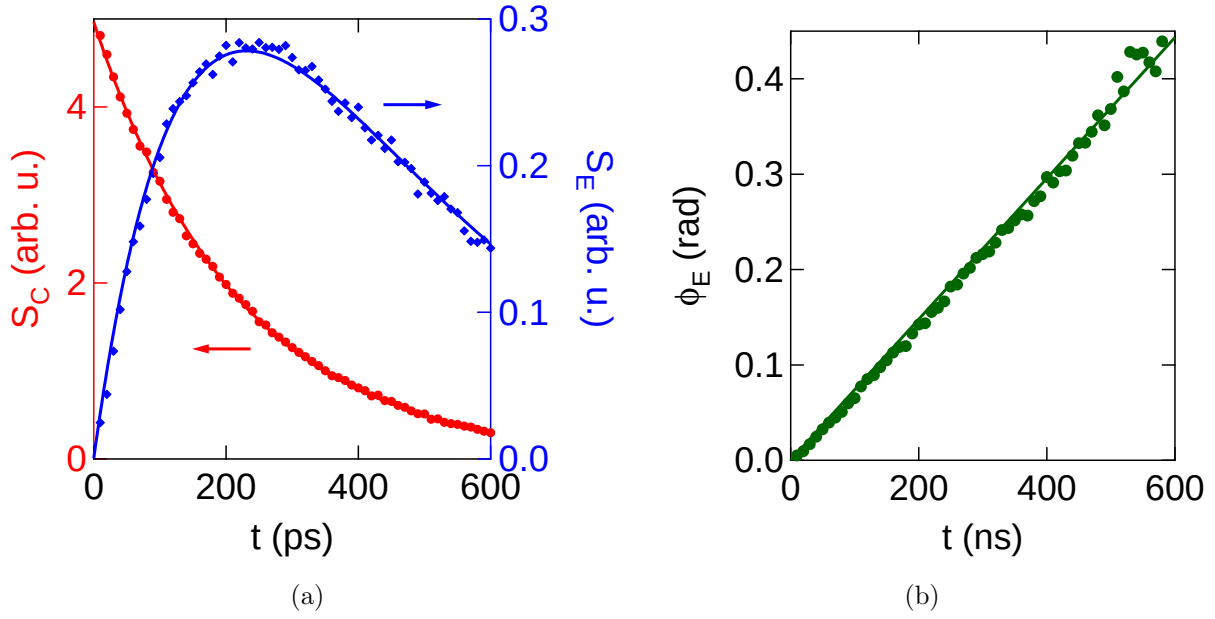
Figure 4.8: (a) The raw data for the two phase modulation schemes in the case of an e - h grating. (b) The ratio of the two measurements gives the phase of the density wave subjected to an applied E field.
