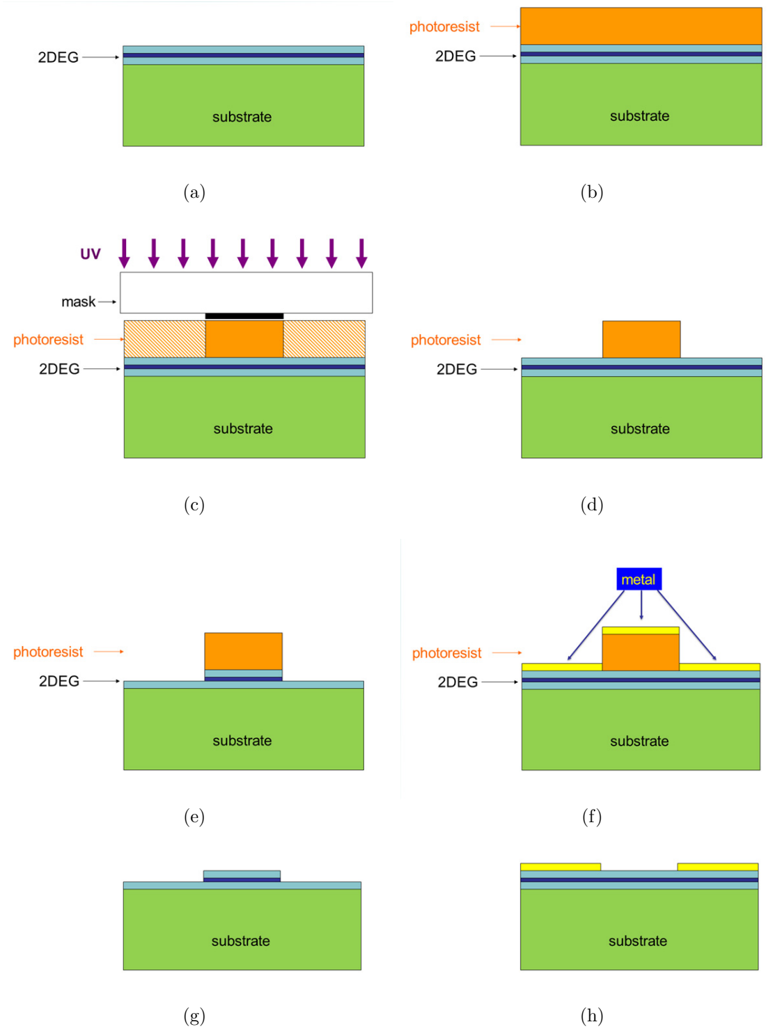
Figure A.7: Demonstration of a sample through the various steps of the photolithographic process. (a) Clean sample; (b) photoresist application; (c) mask alignment and UV exposure; (d) development; (e) mesa etching; (f) metal deposition; (g) and (h) resist removal.
