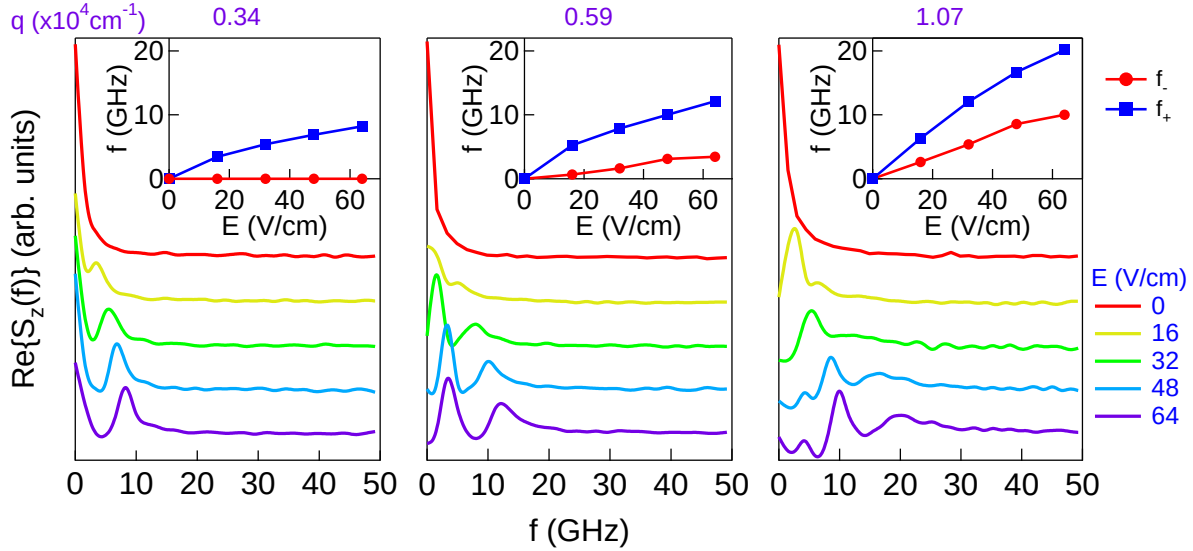
Figure 7.4: The three panels show the Fourier transform of S_z(t) as a function of f for several values of E at T = 30 K, for (left to right) q=0.34, 0.59 , and 1.07 \times 10^4 \text{ cm}^{-1} . Inset: the frequencies of the two peaks as a function of E .
