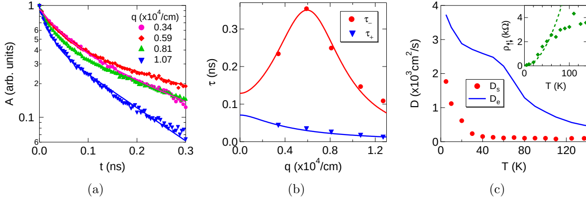
Figure 6.1: Spin diffusion and spin-Coulomb drag. (a) Decay of the amplitude of transient spin gratings measured at several values of the wave vector q . The solid lines are fits to a model of two exponentially decaying helical modes of equal amplitude. (b) Lifetimes \tau_{\pm}(q) for the spin helix modes of opposite pitch obtained from fits to the data in (a). The short-lived mode, \tau_{+}(q) , is proportional to 1/q^2 as expected for diffusion. The lifetime of the long-lived mode, \tau_{-}(q) , is peaked at a non-zero q which is commensurate with the inverse spin-precession length in the SO field. (c) Comparison of spin diffusion coefficient D_s(T) determined from TGS with electron diffusion coefficient D_e(T) determined by transport measurements. Inset: spin transresistivity \rho_{\uparrow\downarrow}(T) extracted from ratio of D_s(T)/D_e(T) . The dashed line is the RPA prediction for \rho_{\uparrow\downarrow}(T) .
