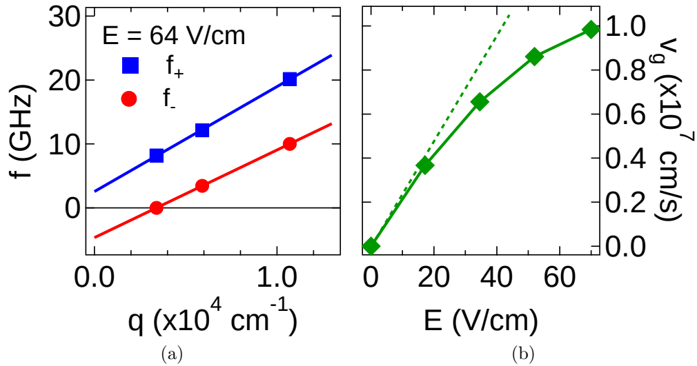
Figure 7.5: (a) The dispersion relations of the resonant frequencies associated with the two helical modes, f_{\pm} , at E = 64 \text{ V cm}^{-1} and T = 30 K. The solid lines are a linear fit. (b) The group velocity v_g of the spin packet as a function of the applied E field at q = 1.07 \times 10^4 \text{ cm}^{-1} and T = 10 K. The dashed line is the extrapolation of the linear response regime at low E , i.e., v_g = \mu_s E .
