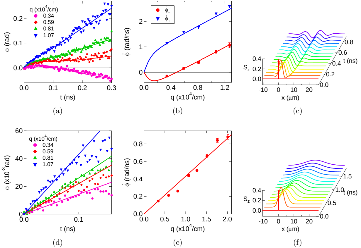
Figure 6.2: Spin drift in different temperature regimes. (a) Spin drift observed by Doppler velocimetry in the presence of an applied electric field ( E = 2 \text{ V/cm} ) at T = 30 \text{ K} . The quantity \phi is the optical phase shift of the probe beam diffracted from the drifting spin grating. After the short-lived helix has decayed, the slope of \phi(t) is proportional to the velocity of the long-lived helix. The solid lines are a fit to Eq. 6.1 describing two independently propagating spin helix modes. The negative slope of the data at low q demonstrates that the long-lived helix mode moves backwards (relative to the Fermi sea) for q < q_0 . (b) Wave vector dependence of the phase velocity associated with the two helical modes, \dot{\phi}_{\pm}(q) , obtained from the fits in (a). The solid lines are a fit to the theoretical model of spin propagation in the presence of Dresselhaus SO coupling described in the text. (c) Real-space spin propagator corresponding to the Fourier transform of the fit in (b). The spin propagator, which describes the space-time evolution of spin polarization following \delta -function injection, has the form of an envelope function that moves at velocity v_d while modulating a stationary helical SDW. Because this stationary pattern decays exponentially, it is necessary to multiply the propagator by \exp[t/\tau_-(q_0)] in order to visualize the motion at long times. (d) and (e) show the same quantities as in (a) and (b), but measured at 150 K. (f) Spin propagator at 150 K showing that transport takes place without coherent spin precession. Error bars (s.d.) in (b) and (e) represent the uncertainty in the fitting of (a) and (d).
