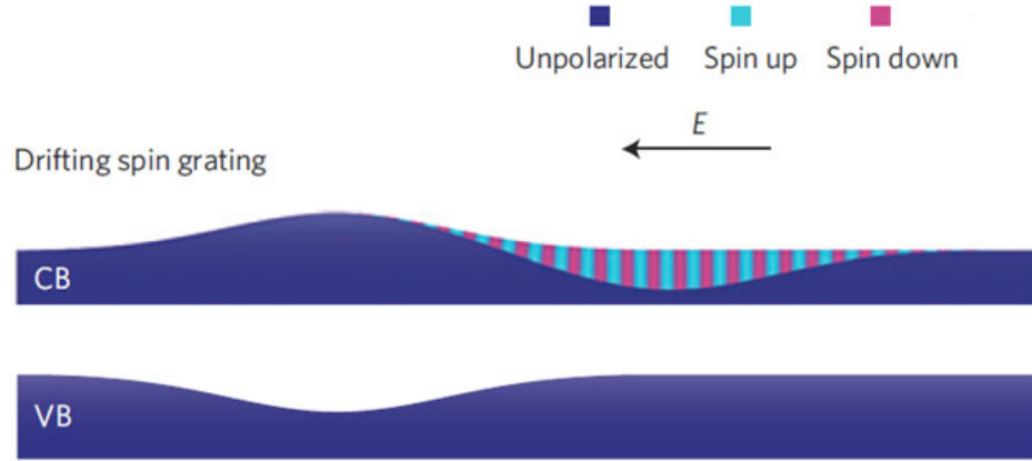
Figure 6.4: Under the influence of an applied E field, the spin grating and the Gaussian e - h packet move in the direction of the Fermi sea of electrons. While the spin grating moves at or near the velocity of the Fermi sea, the e - h packet moves at the much slower ambipolar velocity. This leads to an increasing spatial separation of the spin and charge degrees of freedom. c.f. Fig. 4.2.
