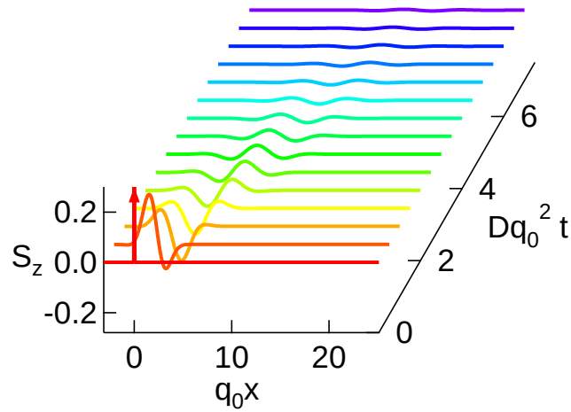
Figure 3.4: The space-time evolution of S_z in the linear-Dresselhaus-only case with the same initial condition and applied E field as in the SU(2) case. The features are similar to those in the SU(2) case, except the envelope function decays exponentially.
