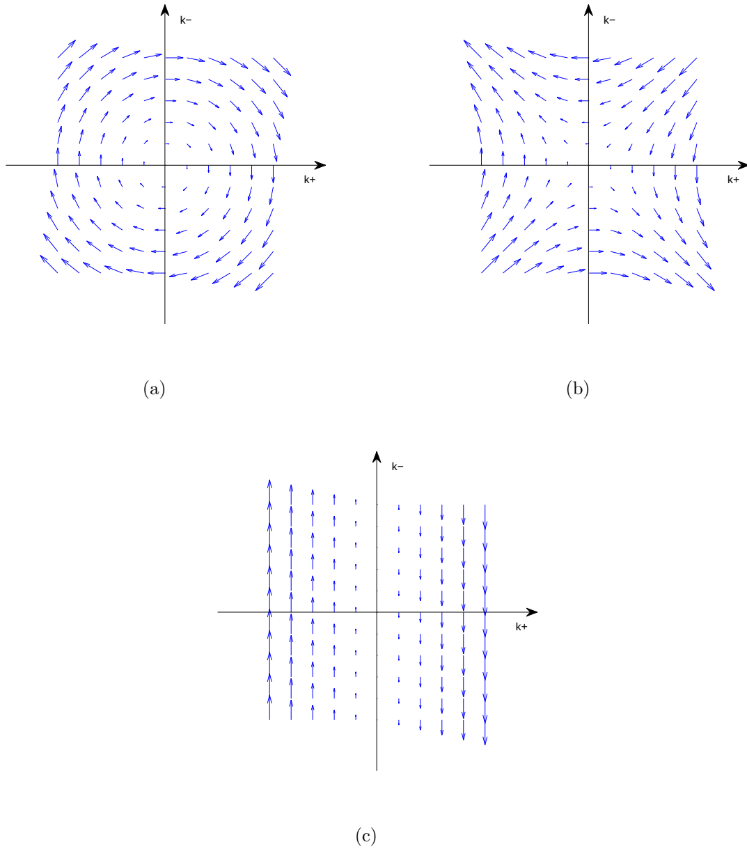
Figure 2.3: Effective SO magnetic fields in the momentum space. (a) Rashba only; (b) linear Dresselhaus only; (c) SU(2).
