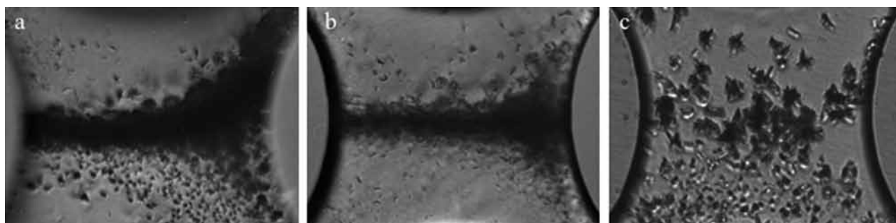
Figure 3. High-resolution (40X objective) brightfield microscopy images showing crystal sizes in single pores of the (a) UP, (b) UCnP, and (c) UPS systems. The pores are located near the inlet, and images were taken after approximately 12–15 h. Individual images are 200 \mu\text{m} in width.
