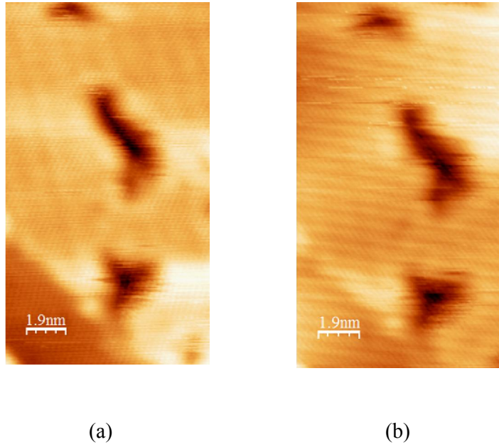
Fig. 6. Same protrusions on \text{ag}/\text{NiAl}(110) under different tunneling conditions. (a), +1.0 \text{ V} tip bias, (b) -1.0 \text{ V} tip bias. Both are taken at 0.5 \text{ nA} tunneling current. Images are both of 9.5 \times 17 \text{ nm}^2 .
