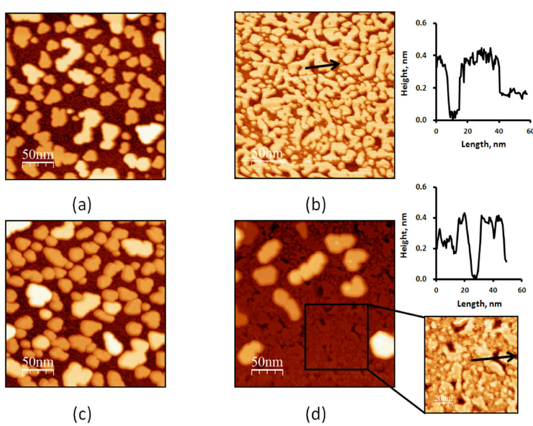
Fig. 13. Representative STM images of Ag/Si(111)- 7 \times 7 surface. A \sqrt{3} -like structure appears after 30 min annealing at 320-330 K. The 2-layer A experiment, 100 L oxygen exposure. (a) clean Ag/Si surface before annealing, (b) clean Ag/Si surface after annealing. The image to the right of (b) is a line profile corresponding to the solid line with an arrow in (b). The direction of the arrow corresponds to the direction of x^+ in the line profile. (c) oxygen-covered surface before annealing, (d) oxygen-covered surface after annealing. The
