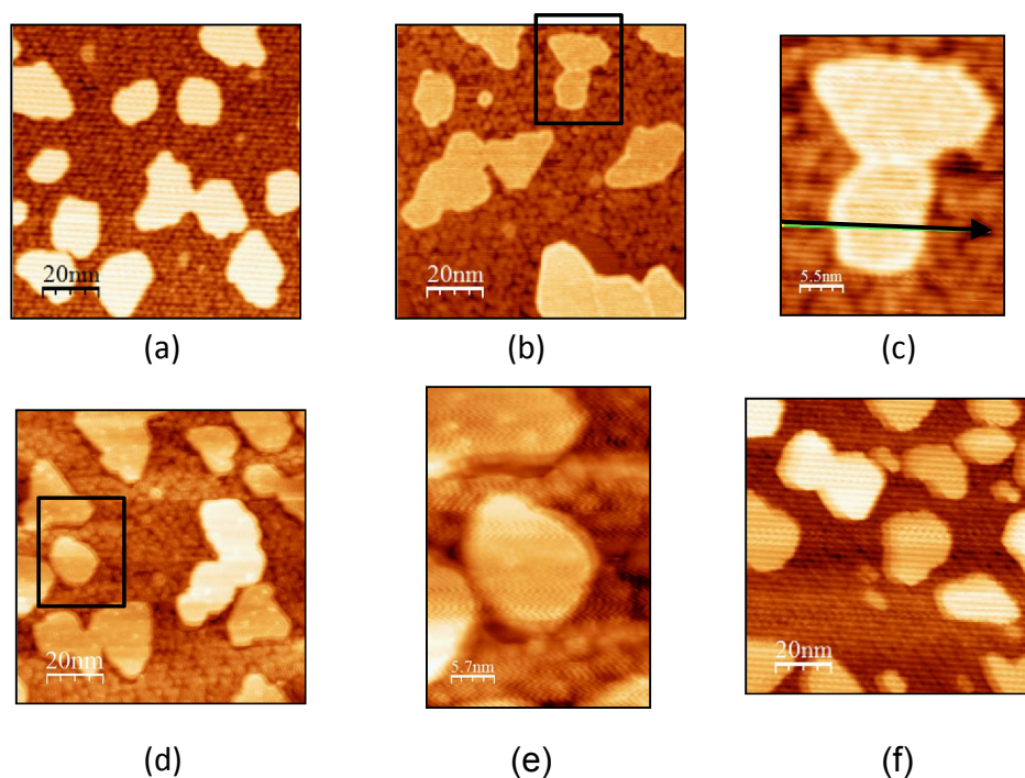
Fig. 3. (a) An STM images of Ag islands on Si(111)- 7\times 7 substrate before ethylene exposure, 100\times 100\text{ nm}^2 . (b) An STM images of Ag islands on Si(111)- 7\times 7 substrate after ethylene exposure (30 L, backfilling), 100\times 100\text{ nm}^2 . (c) An expansion of the boxed area in (b), 27\times 33\text{ nm}^2 . (d) An STM images of Ag islands on Si(111)- 7\times 7 substrate after ethylene exposure (30 L, tube dosing), 100\times 100\text{ nm}^2 . (e) An expansion of the boxed area in (d), 28\times 40\text{ nm}^2 . (f) An STM images of Ag islands on Si(111)- 7\times 7 substrate, annealed to 150 K after ethylene exposure (30 L, tube dosing), 100\times 100\text{ nm}^2 . All images are taken at tip bias of 3.0 V,
