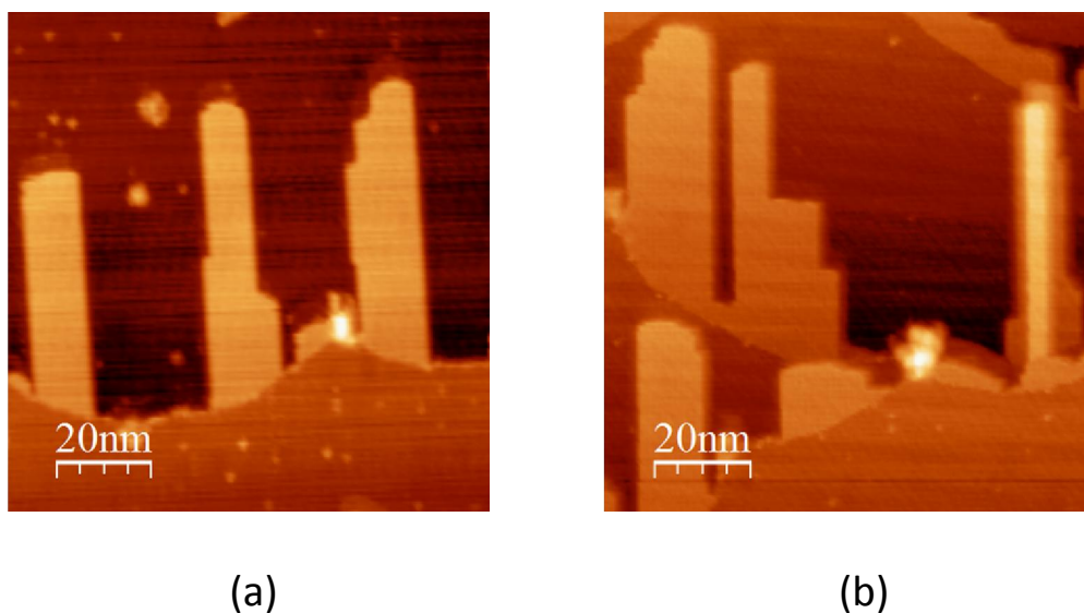
Fig. 1. STM data of Ag on NiAl(110) at 300 K. Image size 100 \times 100 \text{ nm}^2 . +1.0 V tip bias, 0.5 nA tunneling current. (a) and (b) are taken from different areas of the surface and are both representative images of the surface.
