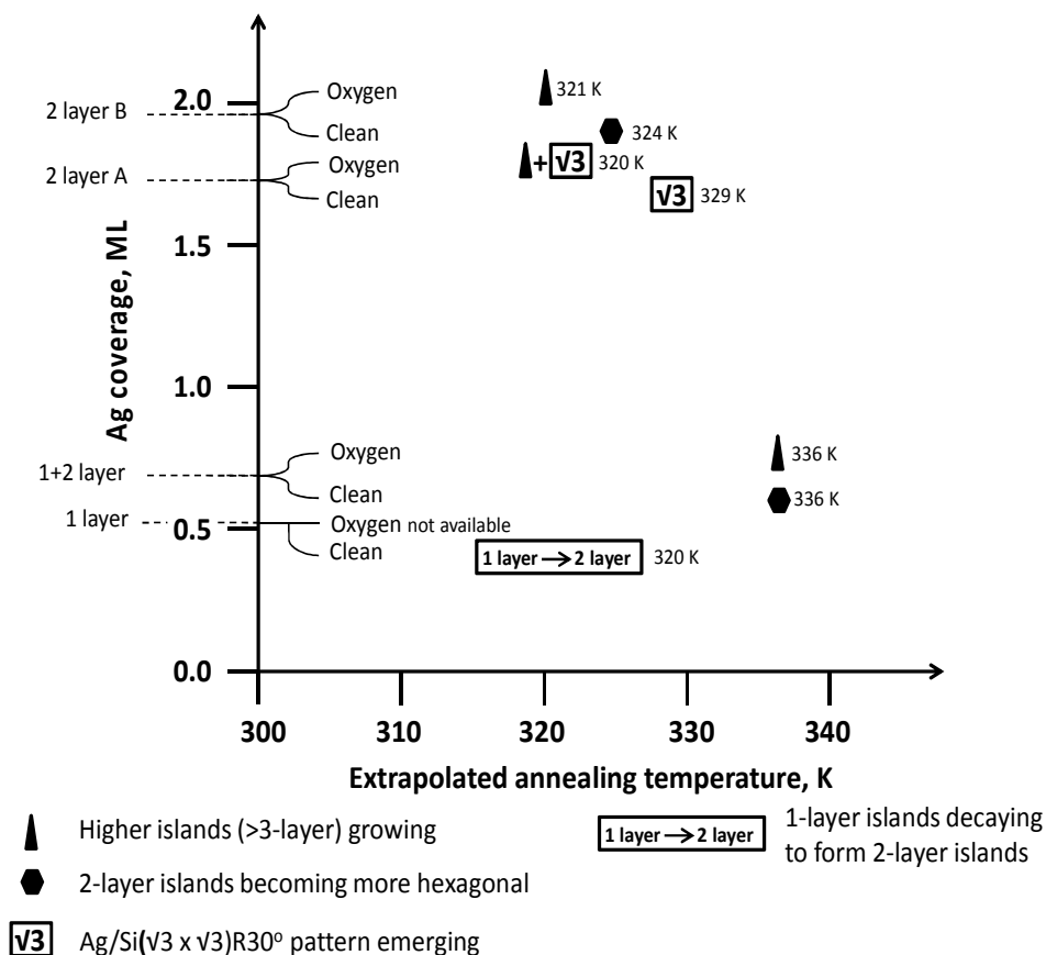
Fig. 14. A schematic diagram of annealing phenomena of all aforementioned experiments.
