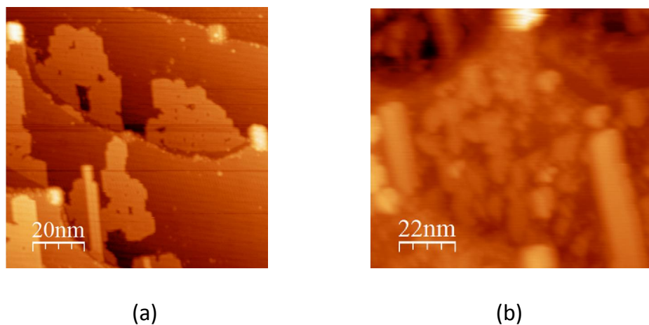
Fig. 8. STM images of Ag islands on NiAl(110) (a) after 11 L O 2 , 100 × 100 nm 2 , -1.0 V tip bias, 0.5 nA tunneling current, and (b) after 111 L O 2 , 110 × 100 nm 2 , +1.0 V tip bias, 0.5 nA tunneling current. The long bright rod-like features in both images are 2nd BL Ag islands.
