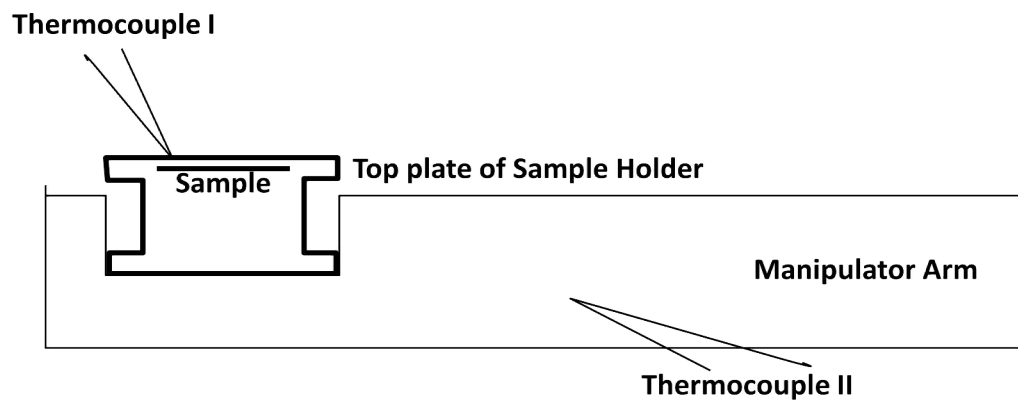
Fig. 1. Schematic diagram of temperature-measurement system.
