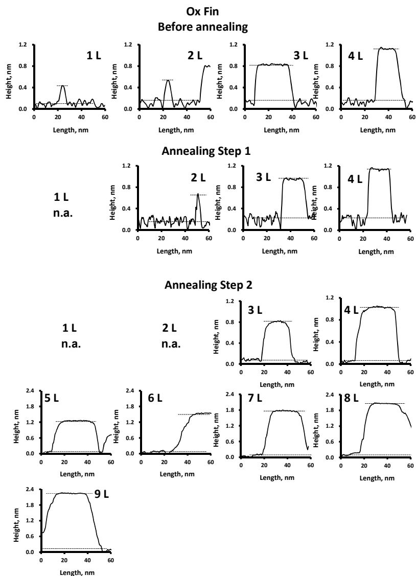
Fig. 4. Run 2: 2-layer B, oxygen exposure experiment (100 L). One representative line profile for an island of each layer thickness.
