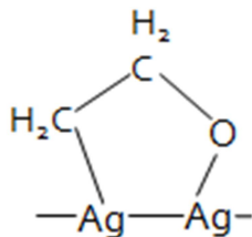
Fig. 1. A schematic diagram of surface oxametallacycles.
