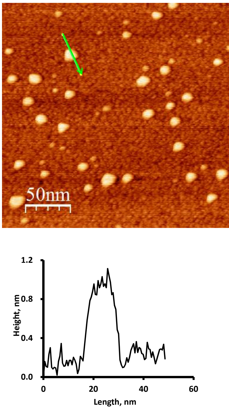
Figure 1.5 Run 1: 1+2-layer, 300 K, 100 L oxygen exposure, A line profile (lower panel) of a 3-layer Ag island (the island crossed by the green line from the upper panel) from the Ag/Si(111)-7×7 surface after oxygen exposure (100 L ) at 300 K, taken at -1.0 V tip bias, 0.5 nA. The upper image size is 250×250 nm 2 .
