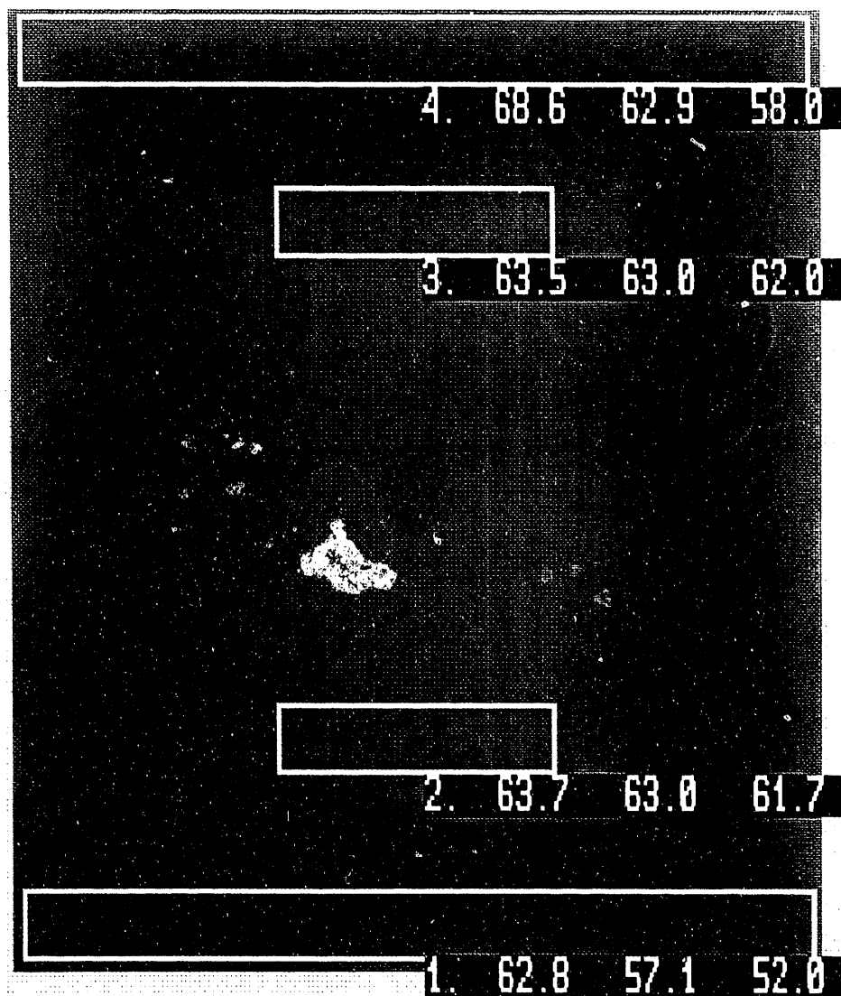
Figure 5. Thermographic image of the warm side of a standard vinyl-framed fixed window with an R-8 \text{ h}\cdot\text{ft}^2\cdot^\circ\text{F}/\text{Btu} ( R-1.41 \text{ m}^2\cdot\text{K}/\text{W} ) center-of-glass glazing. The window was subject to a temperature differential of 65^\circ\text{F} ( 36^\circ\text{C} ) and a cold-side wind speed estimated at 7 mph parallel to the glazing surface. The maximum, average, and minimum temperatures are given in degrees Fahrenheit for four rectangularly bounded regions. Convective airflow within the hollow extrusion cavities creates a temperature gradient between the top (region #4, average temperature 62.9^\circ\text{F} [ 17.2^\circ\text{C} ]) and bottom (region #1, average temperature 57.1^\circ\text{F} [ 13.9^\circ\text{C} ]) of the frame, while the temperature of the insulating glazing unit (regions #2 and 3) is fairly uniform.
