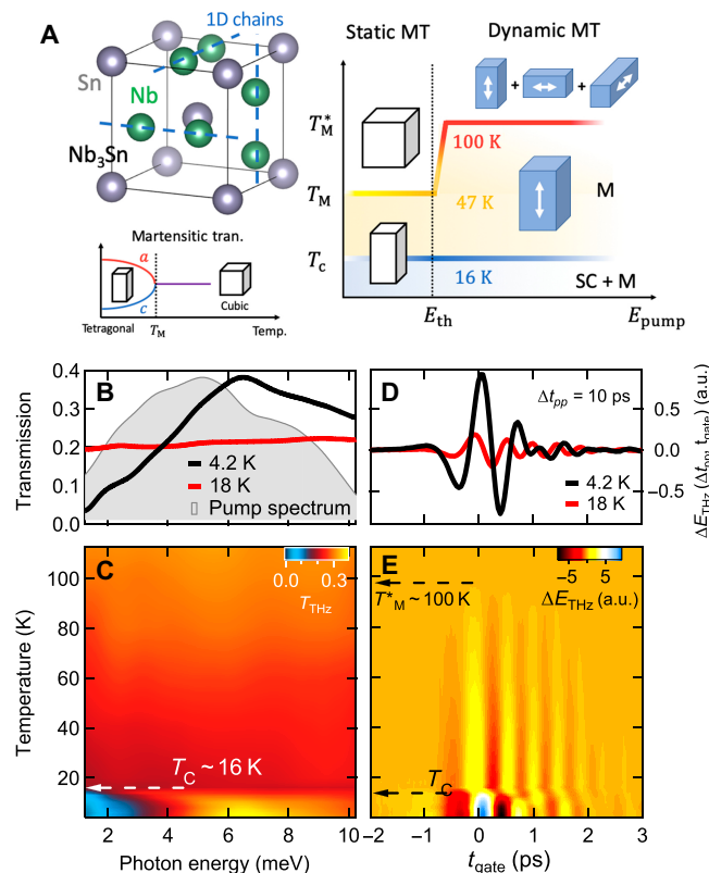
Fig. 1. (A) Left: The crystal structure of \text{Nb}_3\text{Sn} and martensitic transition (MT). Right: Phase diagram. Dynamic MT occurs when E_{\text{pump}} > E_{\text{th}} and T < T_M^* ; at T > T_M^* , vibration is equal superposition of the 3 directions, thus the cubic symmetry is intact. (B) Probe transmission rate T(\omega) shown together with the pump spectra (gray shade). (C) 2D plot of T(\omega) (without pump). (D) Transmitted probe field change \Delta E_{\text{THz}} caused by terahertz pumps, where \Delta E_{\text{THz}} = E_{\text{Trans}}^{\text{pump}} - E_{\text{Trans}}^{\text{NoPump}} . (E) 2D plot of \Delta E_{\text{THz}} (with terahertz pump). A “kink” occurs at T_C \sim 16 K, and \Delta E_{\text{THz}} signals vanish at T_M^* \sim 100 K. The terahertz pump electric field strength used is 940 kV/cm. a.u., arbitrary units.
