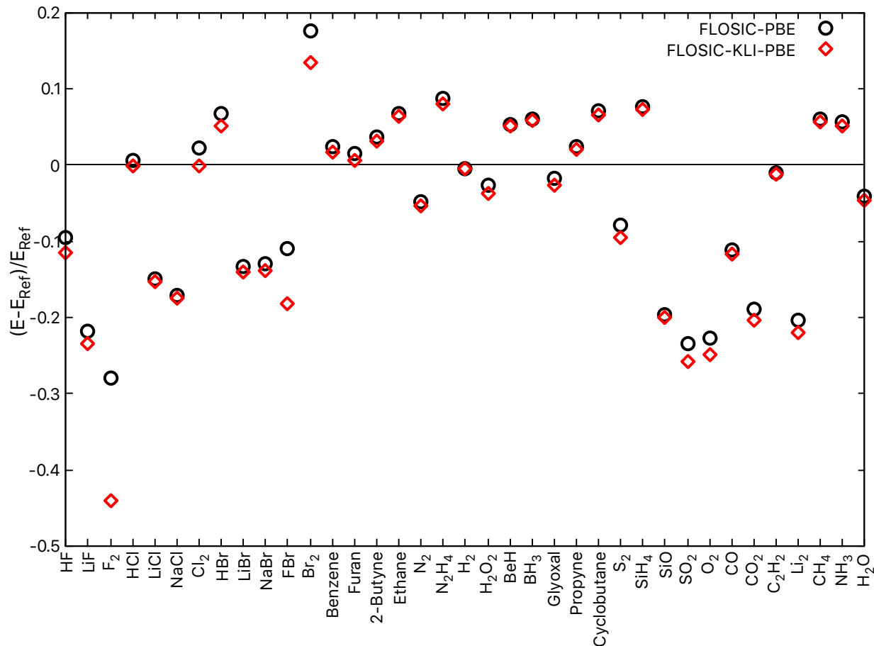
FIG. 4. Relative error (E - E_{Ref})/E_{Ref} of atomization energies of molecules compared against the reference experimental values found in Ref. [68].
