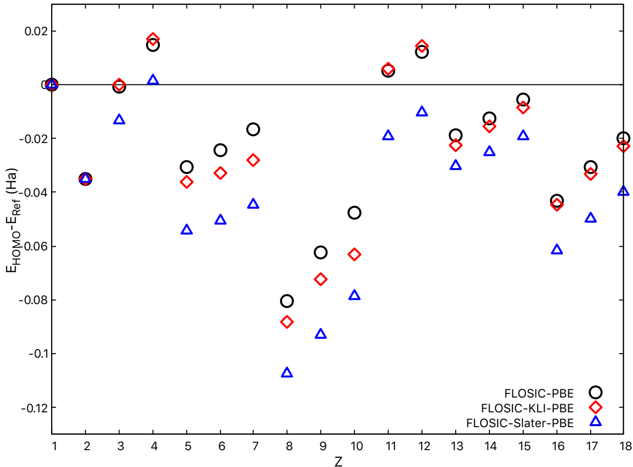
FIG. 3. Error in HOMO eigenvalues compared to experimental IPs 68 .
