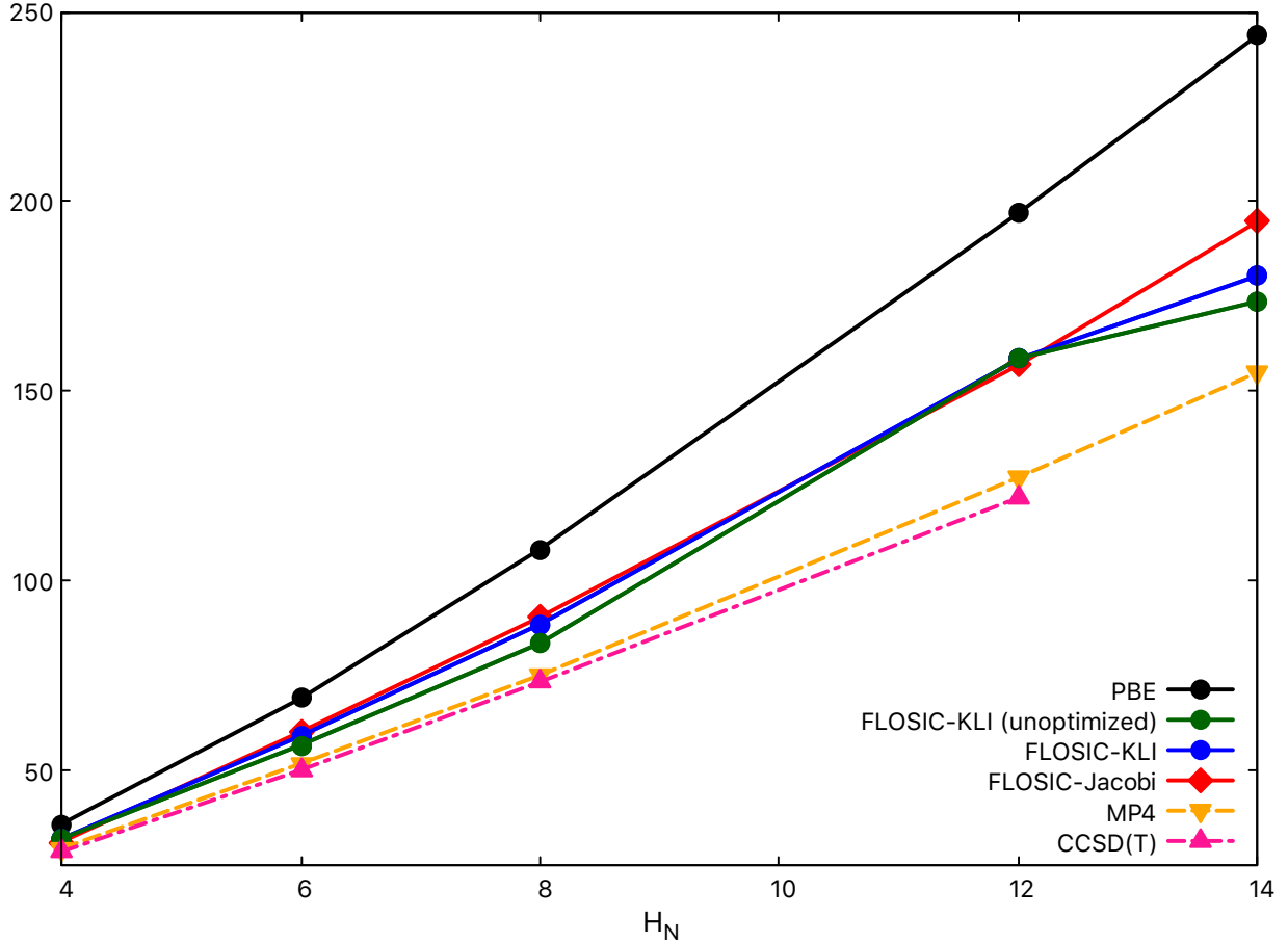
FIG. 6. Polarizabilities \alpha_{zz} of H_2 chains plotted as a function of number of hydrogen atoms. MP4 and CCSD values from Ref. [82].
