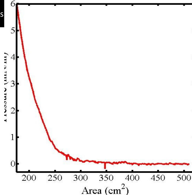
Figure : A surface pressure-area isotherm for P(VDF-TrFE) at the surface of water prior to Langmuir-Blodgett deposition.
