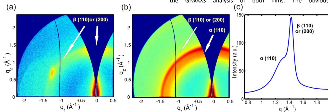
Figure : (a) and (b): GIWAXS diffraction image from (a) an LB-deposited P(VDF-TrFE) (70:30) film; (b) a spin-coated film. Only highly-oriented \beta -phase material is observed in figure 2(a), whereas randomly oriented \beta -phase and \alpha -phase is observed in figure 2(b). This difference indicates substantial changes in the films' structural properties. (c): Integrated intensity of (b) as a function of q .
