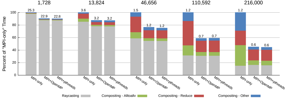
Figure 4: In terms of total render time, MPI-hybrid outperforms MPI-only at every concurrency level, with performance gains improving at higher concurrency.
