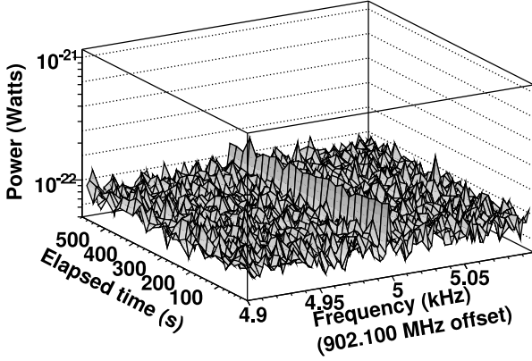
FIG. 3: A simulated chameleon signal corresponding to \beta_\gamma = 2 \times 10^9 with an effective mass of 1.952 \mu\text{eV} superimposed on real data. The data is shown as a series of sequential power spectra; for this case the chameleon decay time is long compared to the integration time.
