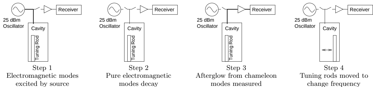
FIG. 1: Chameleon search procedure
