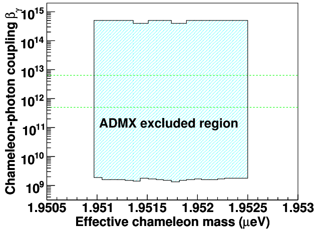
FIG. 4: Shaded region: 90% confidence limit excluded parameters for scalar chameleons from ADMX search. Dashed lines: upper and lower exclusion bounds from Ref. [12].
