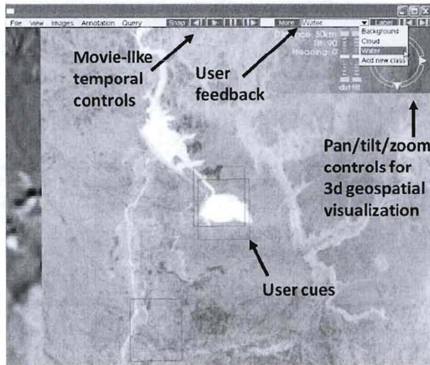
Figure 9. Prototype interface for identifying anomalous changes in remote sensing imagery.
