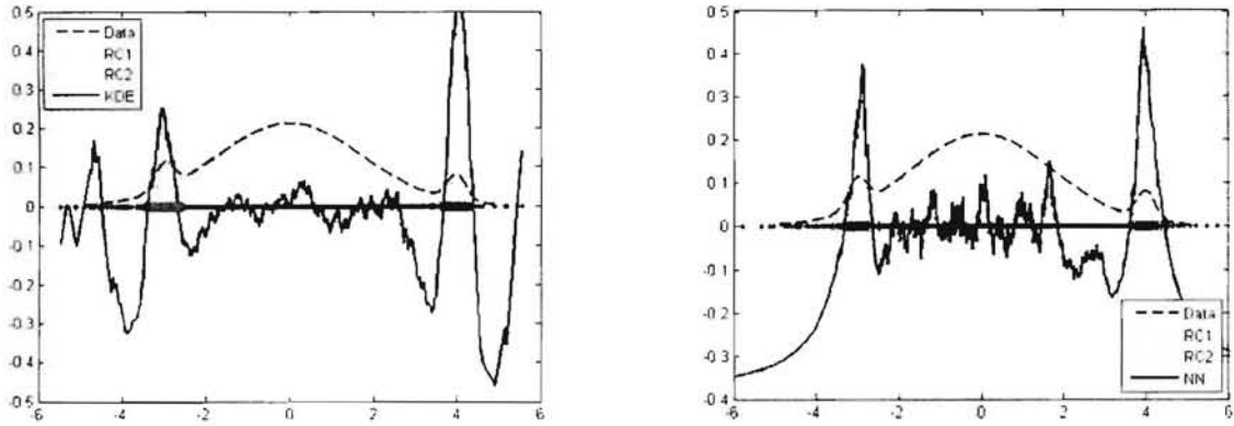
Figure 4. Left) A Kernel Density Estimate (Equation 4) with d_1 = 0.1 and d_2 = 1 and Right) Nearest Neighbor Estimate (Equation 5) with k = 20 and l = 75 .
