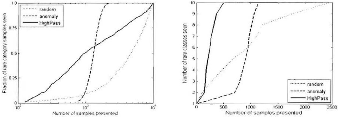
Figure 5. Left) Performance comparison when detecting all rare category samples and Right) comparison when detecting at least one sample from each category.
