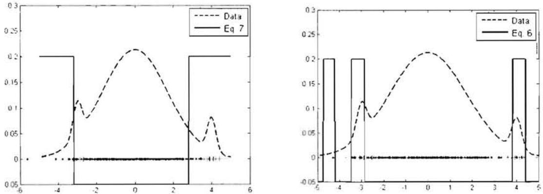
Figure 6. Left) Indicator function produced via anomaly detection using a SVM classifier and Right) Indicator function produced by Equation 6 using a SVM classifier.
