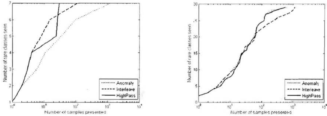
Figure 8. Performance comparison on Left) Shuttle dataset and Right) Abalone dataset.
