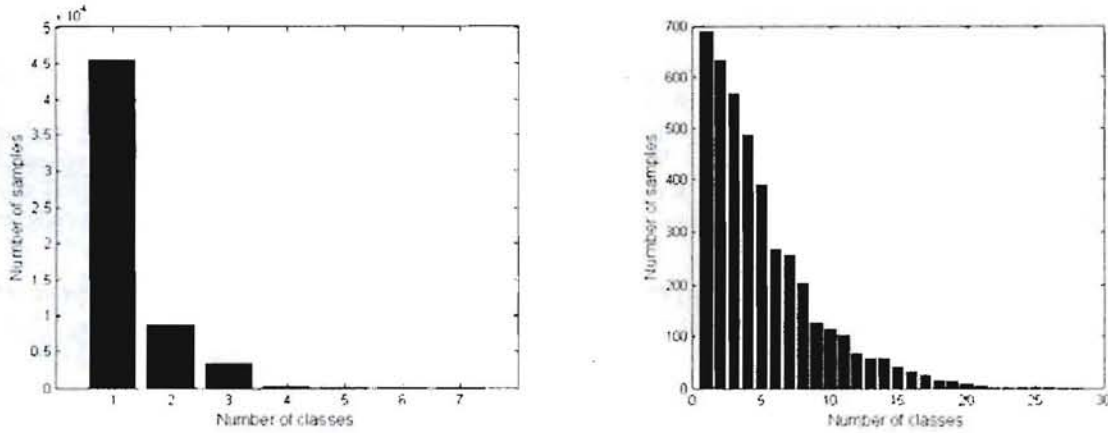
Figure 7. Left) Shuttle dataset class distribution and Right) Abalone dataset class distributions.
