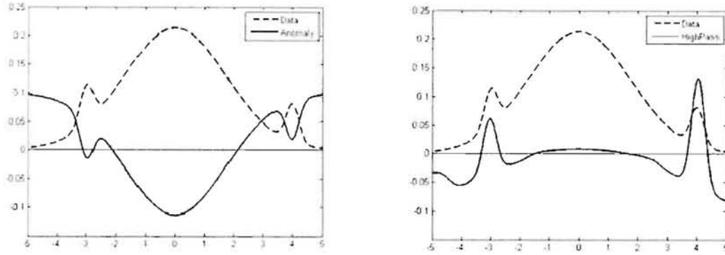
Figure 3. Left) Sample weighting function produced by Equation 1 (Anomaly) and Right) Sample weighting function produced by Equation 2 (HighPass).
