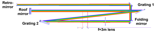
Figure 2: Hyper-dispersion stretcher provides dispersion of 7000 ps/nm in a compact 3x1 m footprint.
