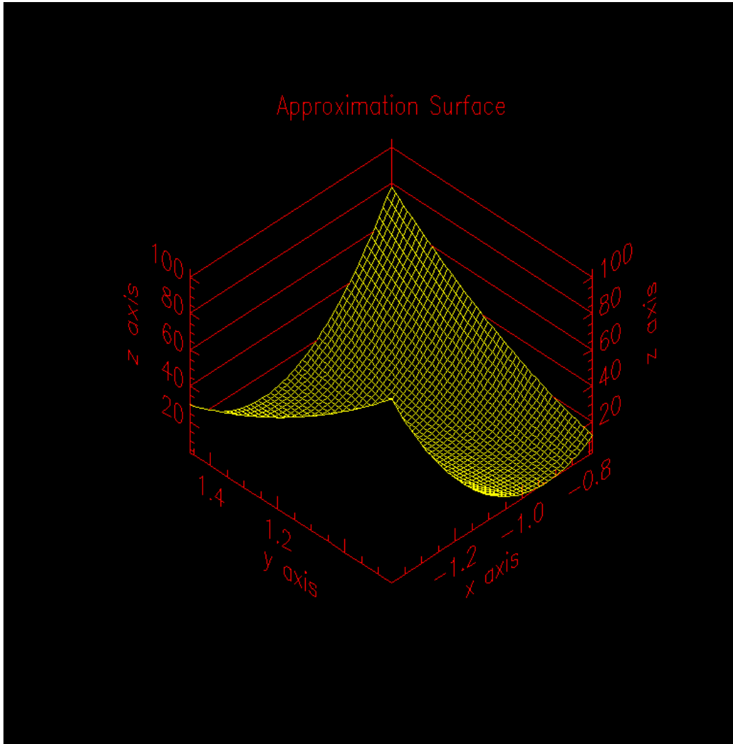
Figure 16.5: An example of the 3-D surface plotting that is available for surrogate-based optimization with two design parameters.
