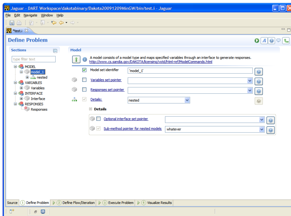
Figure 15.10: JAGUAR with push-up elements enabled (default).
