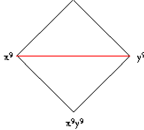
Figure 6.12: Pascal's triangle depiction of integrand monomial coverage for two dimensions and Gaussian tensor-product quadrature order = 5. Red line depicts maximal total-order integrand coverage.
