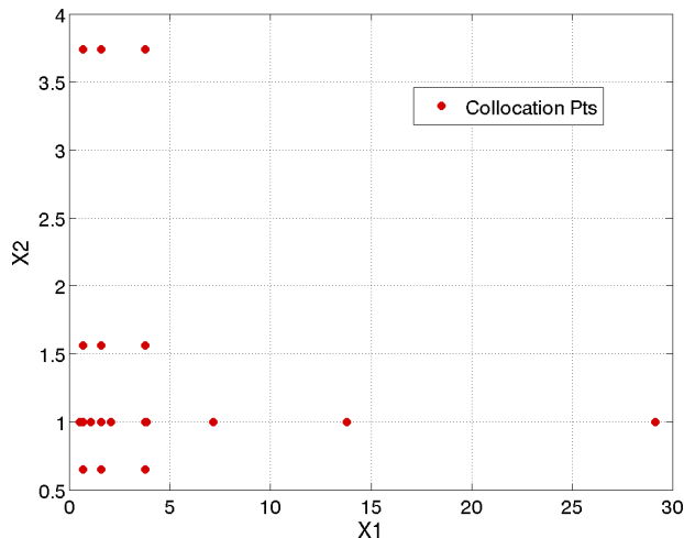
Figure 6.16: Rosenbrock stochastic collocation example: sparse grid points.
