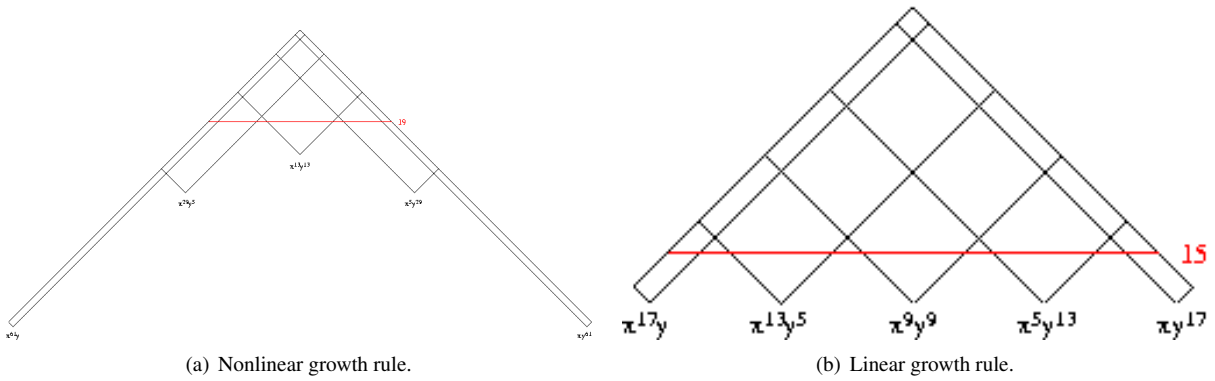
Figure 6.14: Pascal’s triangle depiction of integrand monomial coverage for two dimensions and Gaussian sparse grid level = 4. Red line depicts maximal total-order integrand coverage.
