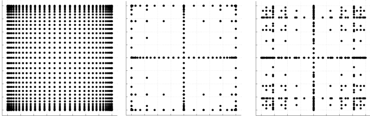
Figure 6.13: For a two-dimensional parameter space ( n = 2 ) and maximum level w = 5 , we plot the full tensor product grid using the Clenshaw-Curtis abscissas (left) and isotropic Smolyak sparse grids \mathcal{A}(5, 2) , utilizing the Clenshaw-Curtis abscissas (middle) and the Gaussian abscissas (right).
