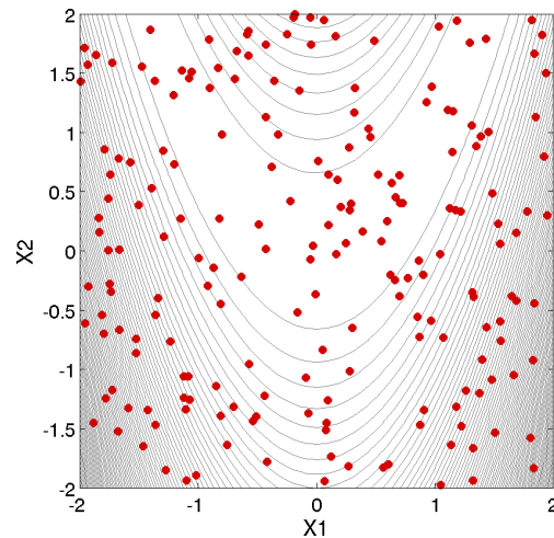
Figure 2.21: Monte Carlo sampling example: locations in the parameter space of the 200 Monte Carlo samples using a uniform distribution for both x_1 and x_2 .
