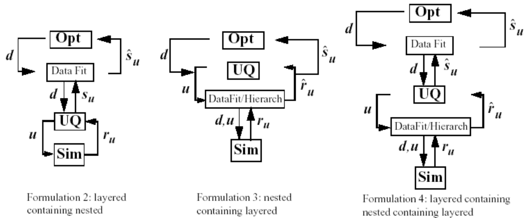
Figure 11.6: Formulations 2, 3, and 4 for Surrogate-based OOU.
