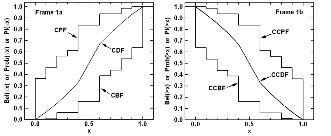
Figure 6.18: Example cumulative belief and plausibility distribution functions on left; complementary cumulative belief and plausibility distribution functions on right
