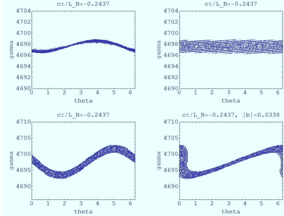
Figure 3: EEHG simulation results using GINGER showing the bunch phase space at a normalized distance of 0.24 from the tail of the bunch of a 43 nm oscillator followed by a 215 nm laser-driven modulator (replacing the second oscillator in Fig. 1). Plotted are the longitudinal phase space after the 43 nm oscillator (top left), the first chicane (top right), the 215 nm modulator (bottom left) and after the second chicane (bottom right). The bunching is over 3% at the 80th harmonic of 215 nm.
