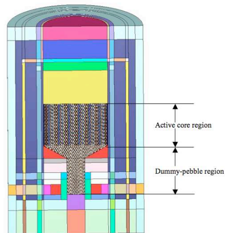
Fig. 2. SCALE/KENO geometric model of the HTR-10 startup core configuration.
