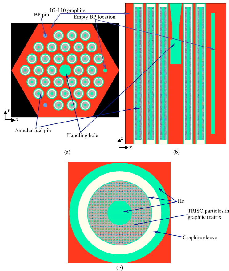
Fig. 1. Cross-sectional (a), vertical (b) views of the HTTR fuel block and fuel pin detail with explicit TRISO particles modeling (c) for the SCALE/KENO CE model.
