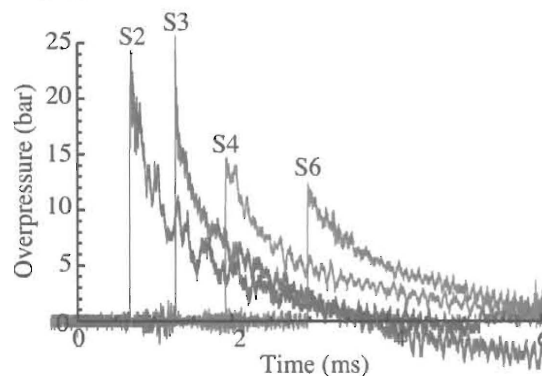
FIGURE 1. Pressure traces for a C4 test.
