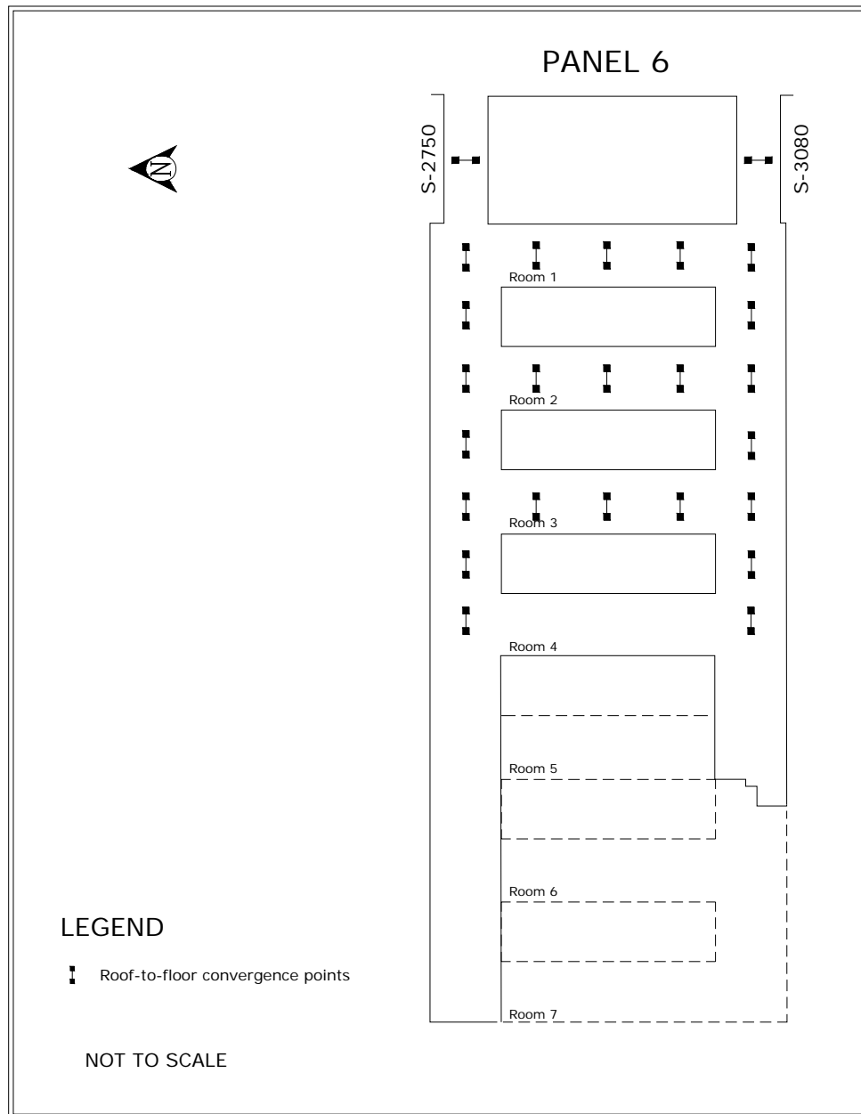
Figure 6-4 – Location of Panel 6 Geotechnical Instruments
