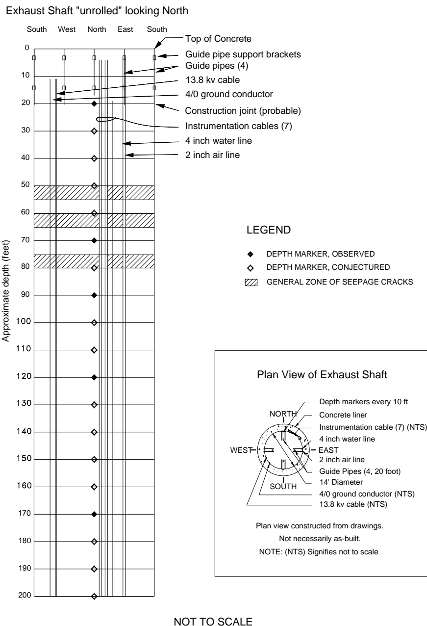
Figure 3-9 – Diagram of Exhaust Shaft Fixtures and Seepage Zones (Upper 200 ft)
