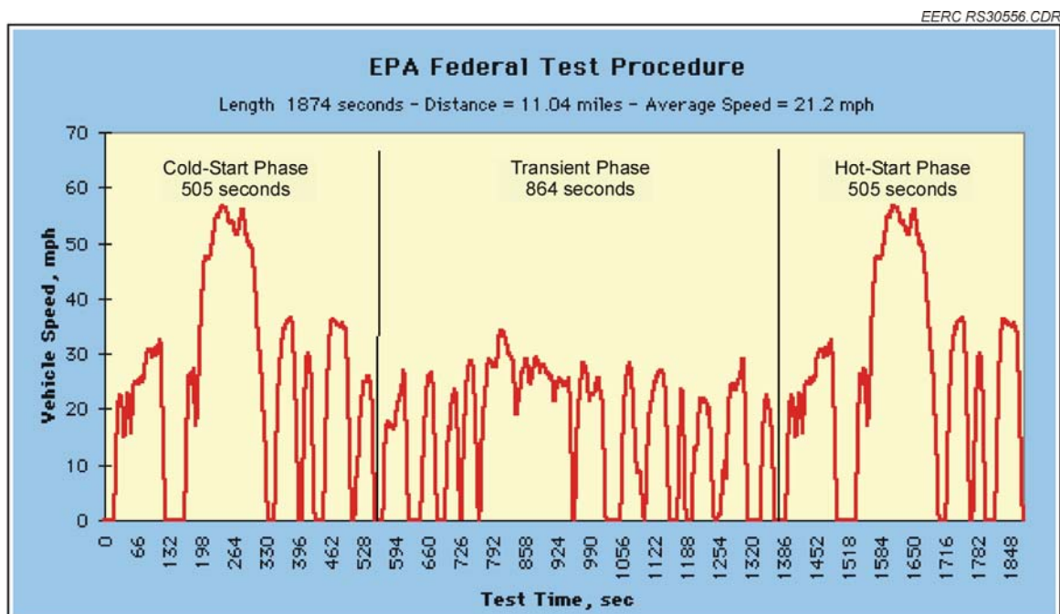
Figure 7. FTP-75.
