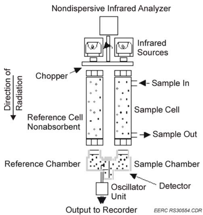
Figure A-2. Infrared analyzer.
