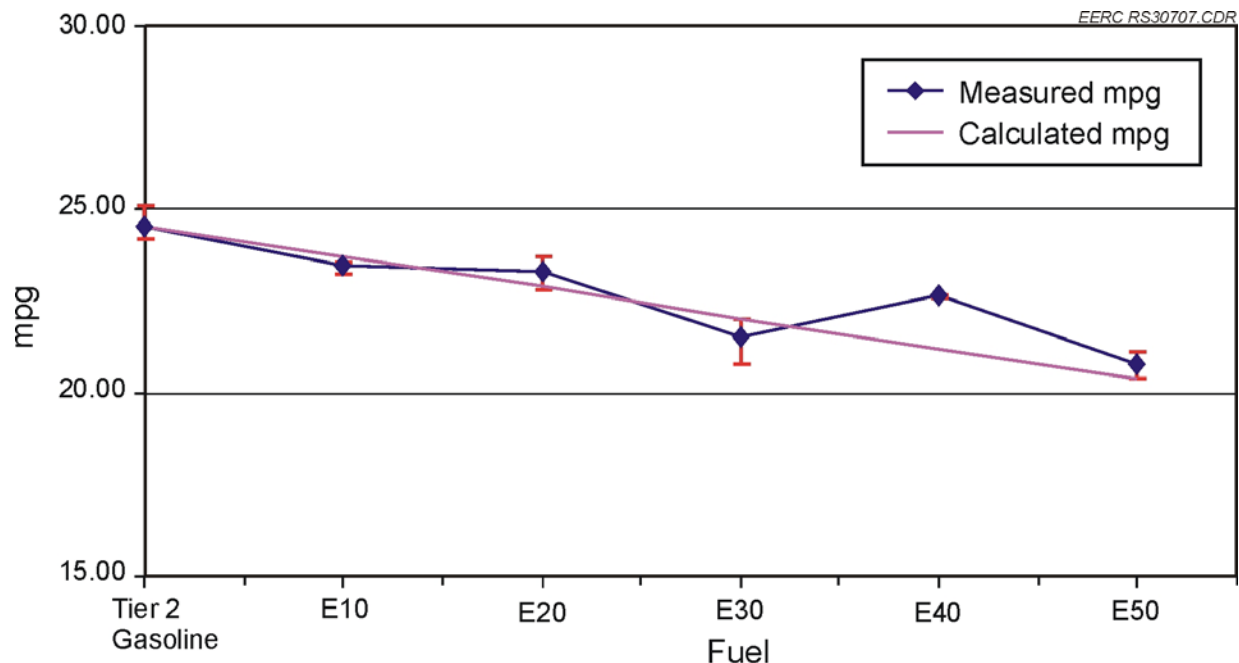
Figure 11. 2007 Chevrolet Impala (non-flex fuel), 3.5-L engine, highway fuel economy.
