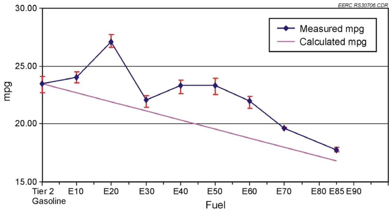
Figure 12. 2007 Chevrolet Impala (flex fuel), 3.5-L engine, highway fuel economy.
