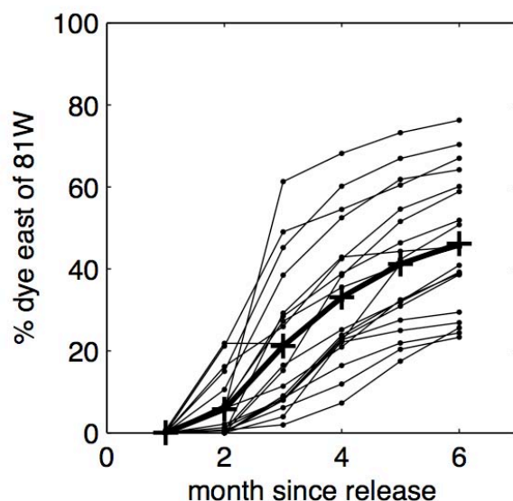
Figure 3. Percentage of total dye that exits the Gulf of Mexico at 81°W for all 20 ensemble members (thin lines). The thick line with “+” symbols denotes the ensemble mean.
