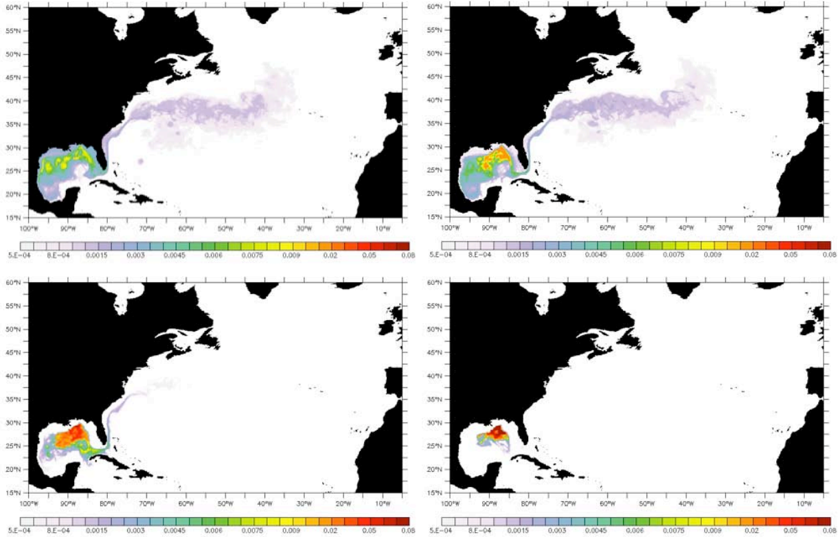
Figure 4: Mean dilution factors based on a five-member ensemble one year after the initial spill: a) dye release at 0–20 m depth; b) dye release at 20–210 m depth; c) dye release at 210–800 m depth; d) dye release at 800–1,500 m depth. Color represents dilution factor on a logarithmic scale.
