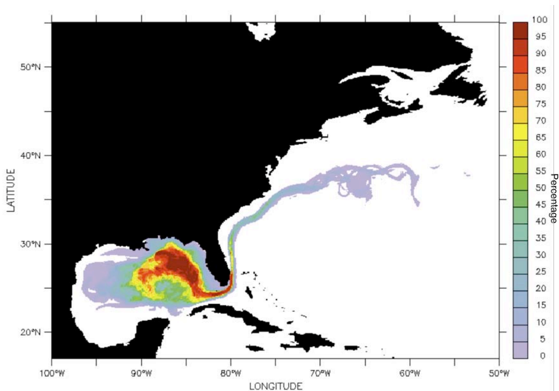
Figure 2: Percentage of ensemble members where dye (based on a 0.01 dilution factor) has reached a given location 190 days after the start of a two-month dye release.
