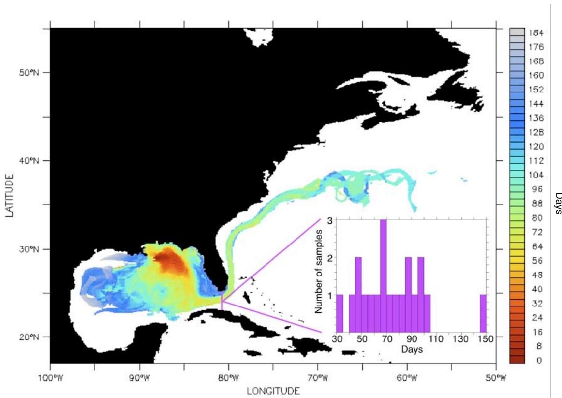
Figure 1: Ensemble mean arrival times (in days) of dye based on a 0.01 dilution factor in the 20-member ensemble. The insert histogram shows the ensemble distribution of arrival times in the Florida Strait.
