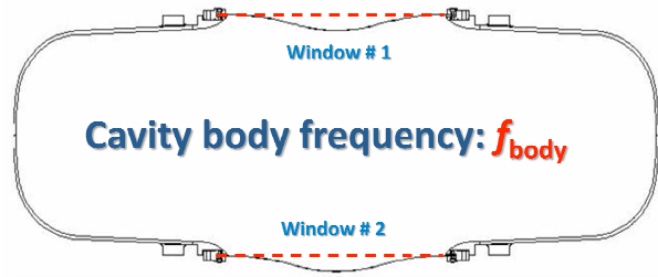
Figure 7: The measured frequency is referred to as cavity body frequency with flat windows as shown. The cavity frequency with curved windows is considered to be a perturbation on the cavity body frequency.
