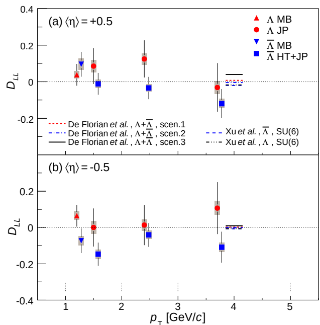
FIG. 4: (Color online) Comparison of \Lambda and \bar{\Lambda} spin transfer D_{LL} in polarized proton-proton collisions at \sqrt{s} = 200 \text{ GeV} for (a) positive and (b) negative \eta versus p_T . The vertical bars and bands indicate the sizes of the statistical and systematic uncertainties, respectively. The \bar{\Lambda} data points have been shifted slightly in p_T for clarity. The dotted vertical lines indicate the p_T intervals in the analysis of HT and JP data. The horizontal lines show model predictions evaluated at \eta and largest p_T of the data.
